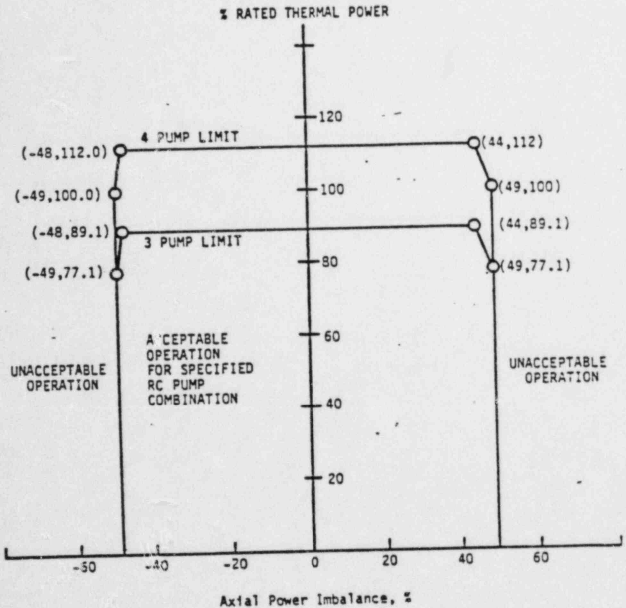
Figure 2.1-2 Reactor Core Safety Limit.
