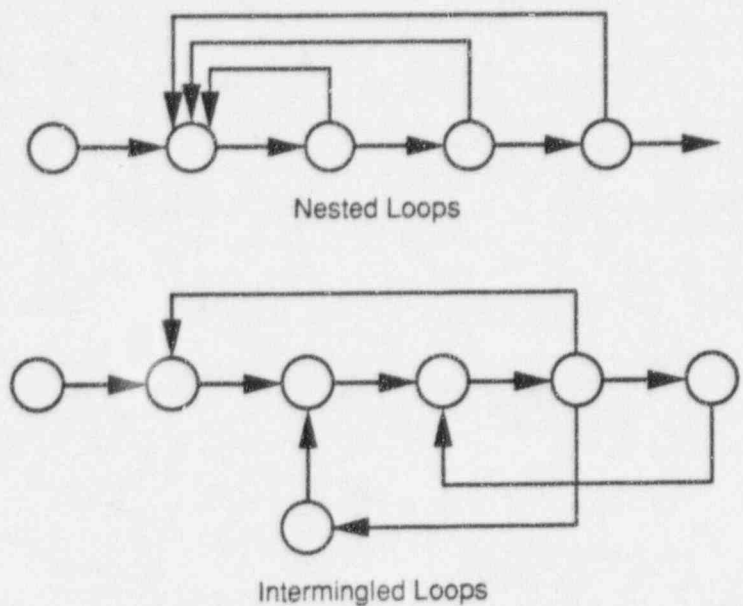
Figure 3-4. Examples of Loops in Flowgraphs
