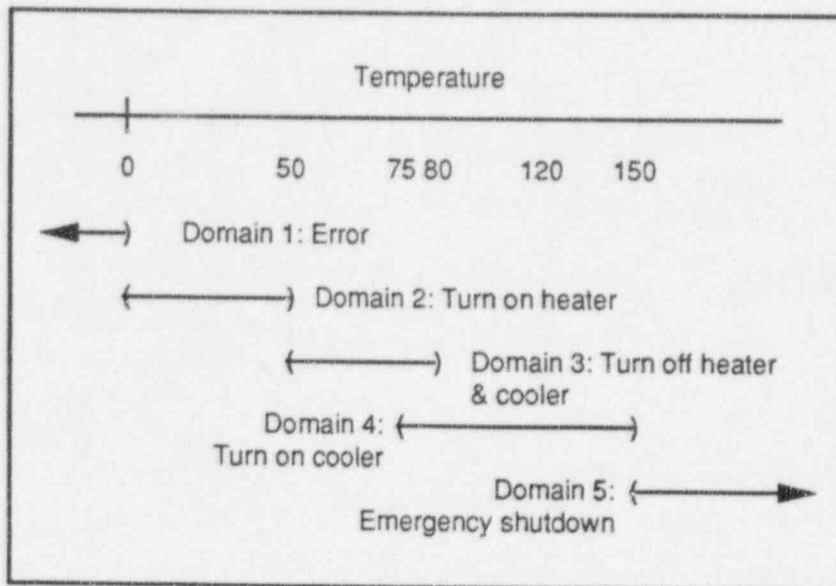
Figure 4-3. Example of Domains
