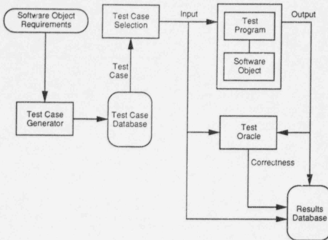
Figure 4-1. Typical Test Station Components for Functional Testing
