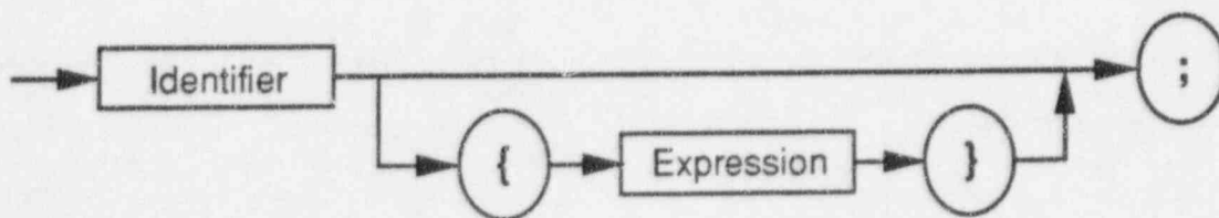
Figure 4-5. Example of a Syntax Graph
