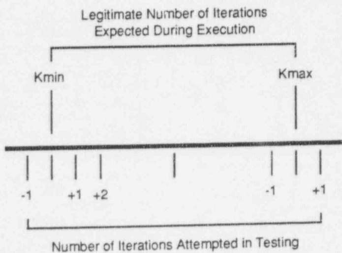
Figure 3-5. Test Cases in Loop Testing
