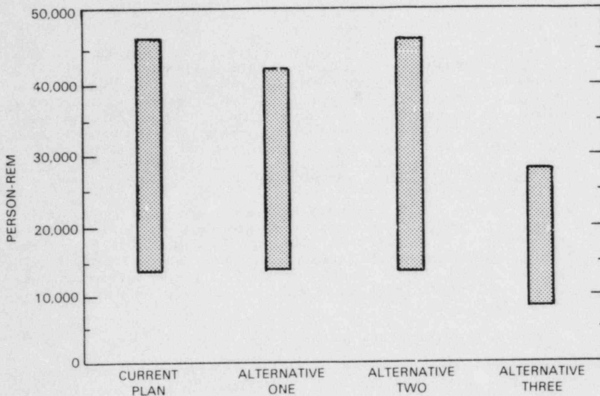
FIGURE 2.9. Occupational Radiation Dose to Complete Cleanup
