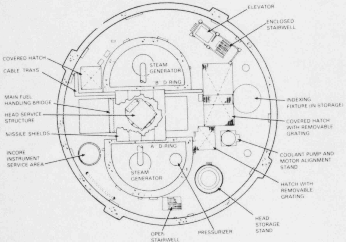
FIGURE 2.3. 347-Ft Elevation
