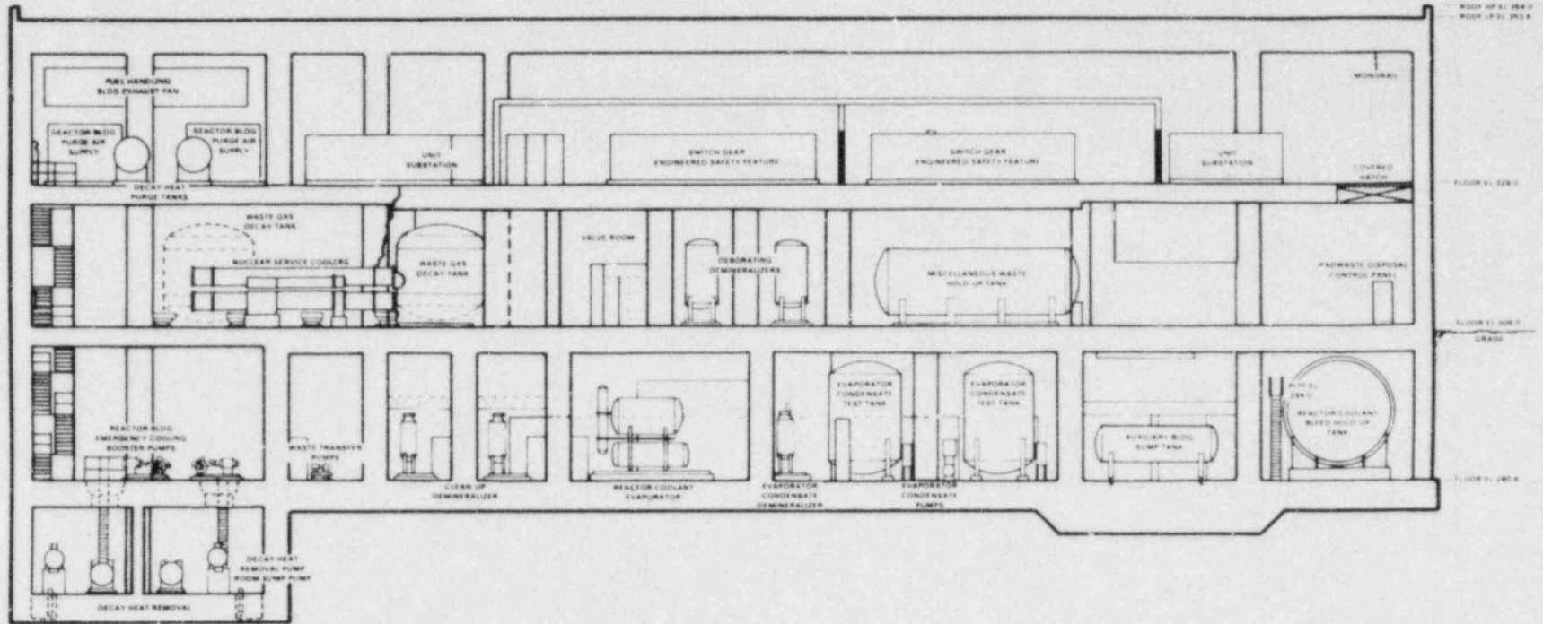
FIGURE 2.8. Cutaway View of Auxiliary and Fuel-Handling Building
