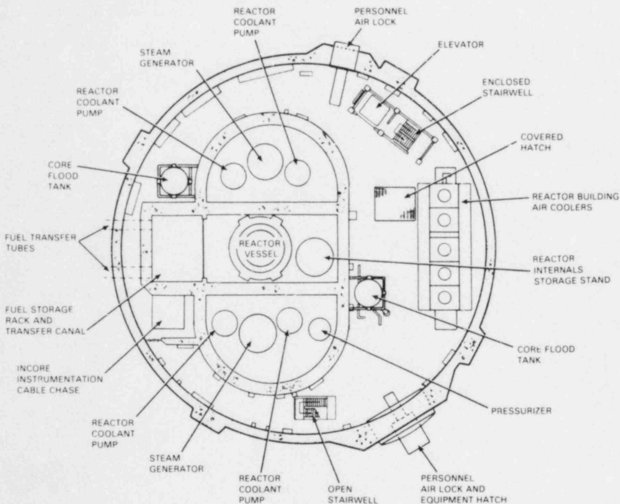
FIGURE 2.2. 305-ft Elevation
