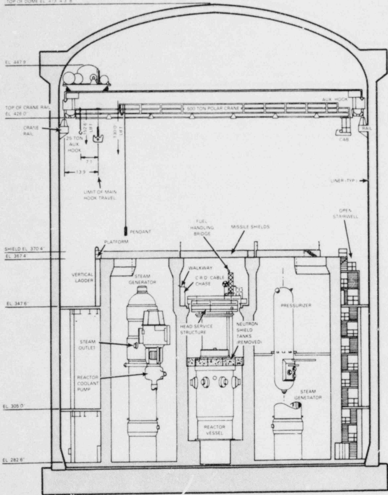
FIGURE 2.1. Reactor Building
