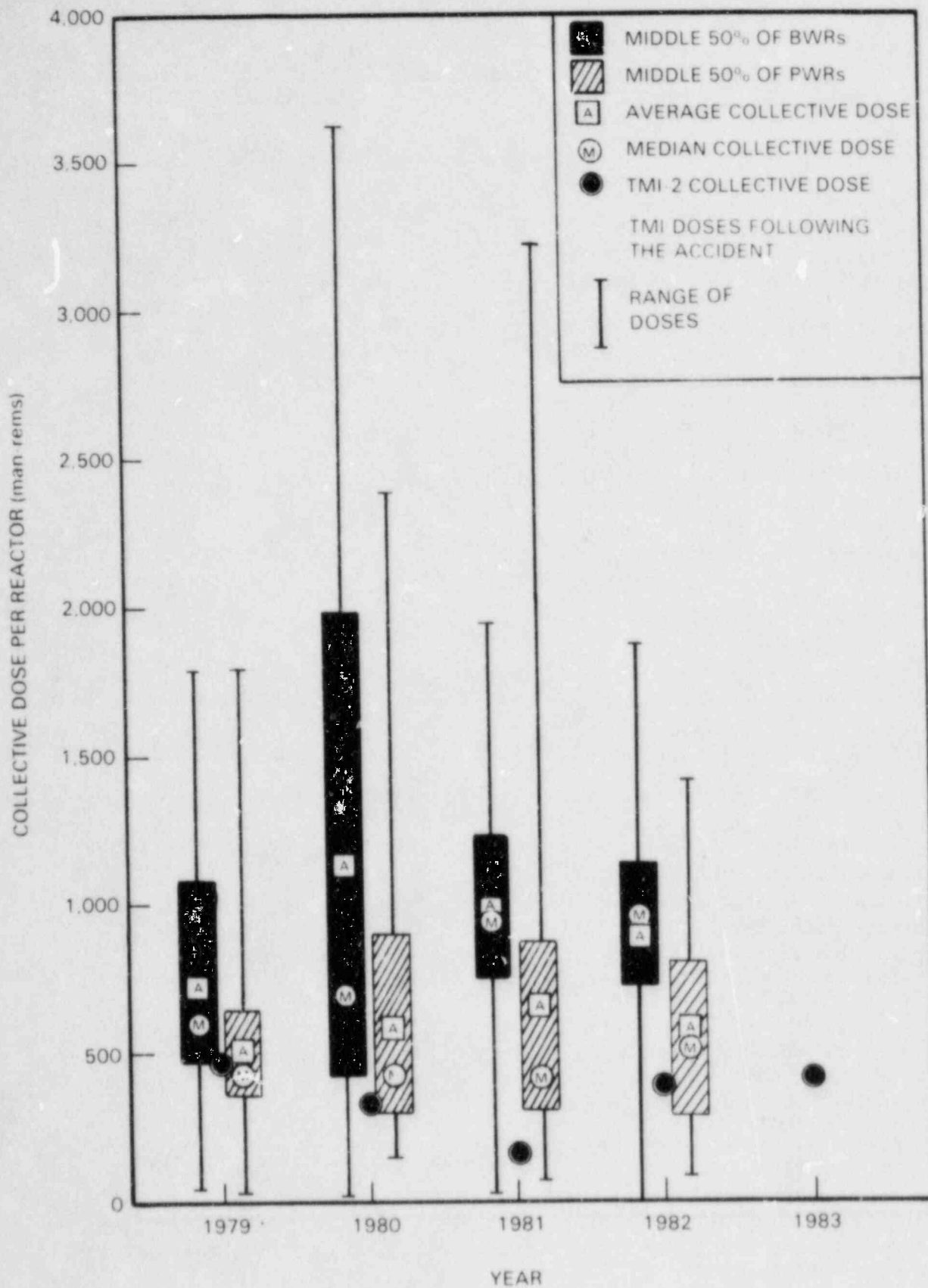
FIGURE 1.1. Doses at TMI-2 Compared with Doses Per Reactor at All Commercial Nuclear Plants in the United States
