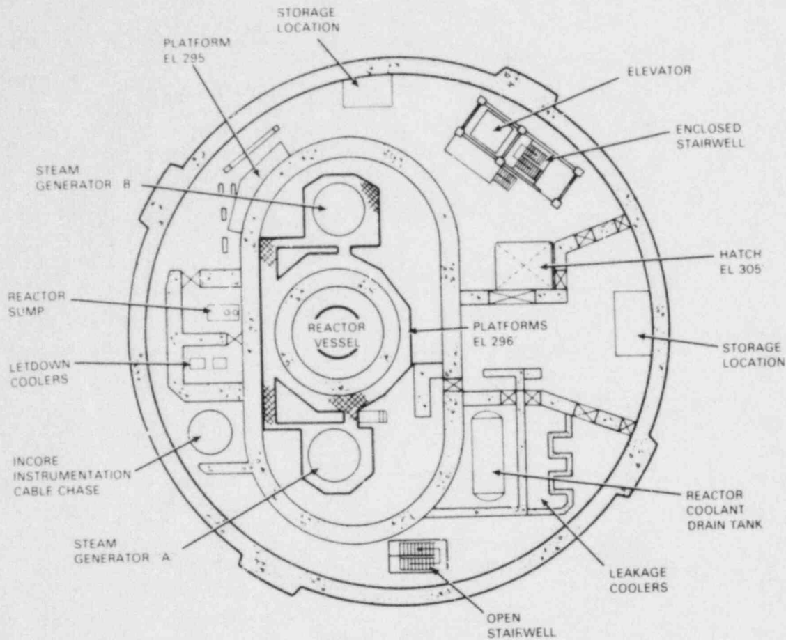
FIGURE 2.4. 282-ft Elevation
