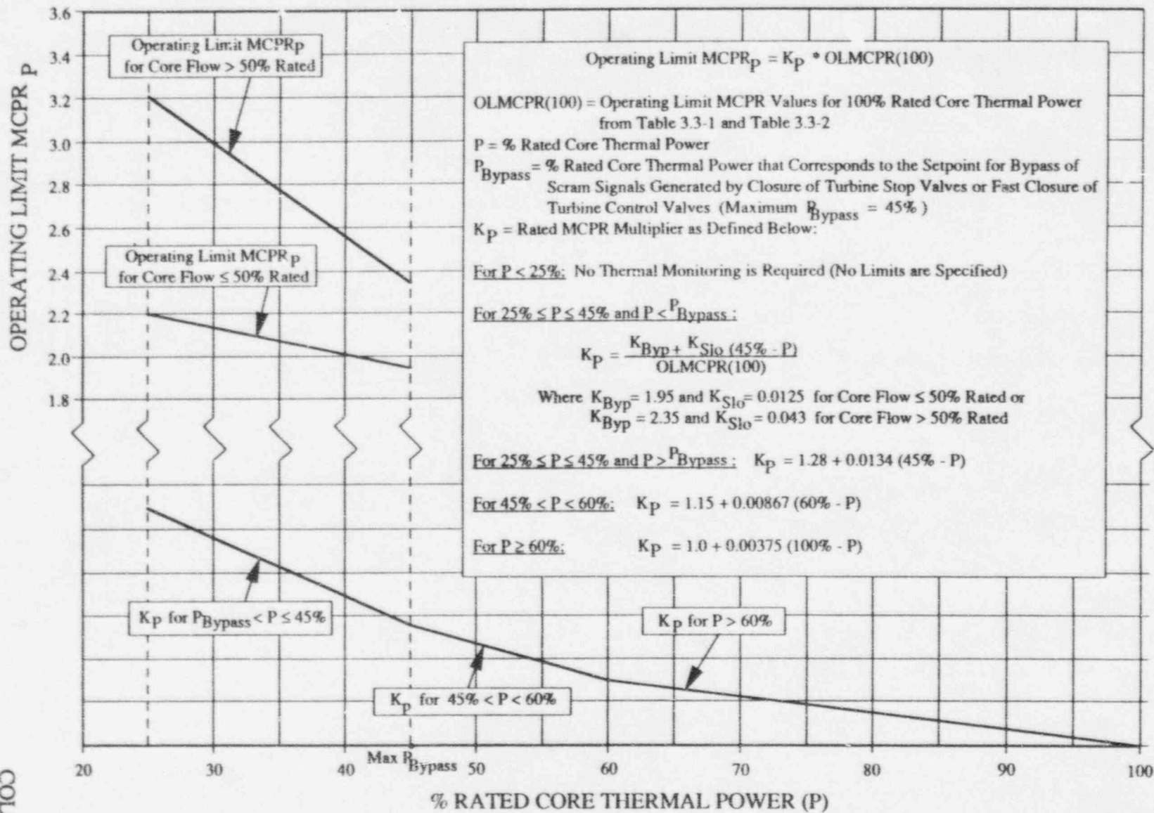
FIGURE 3.3-2 Power Dependent MCPR Limits (MCPR p )
