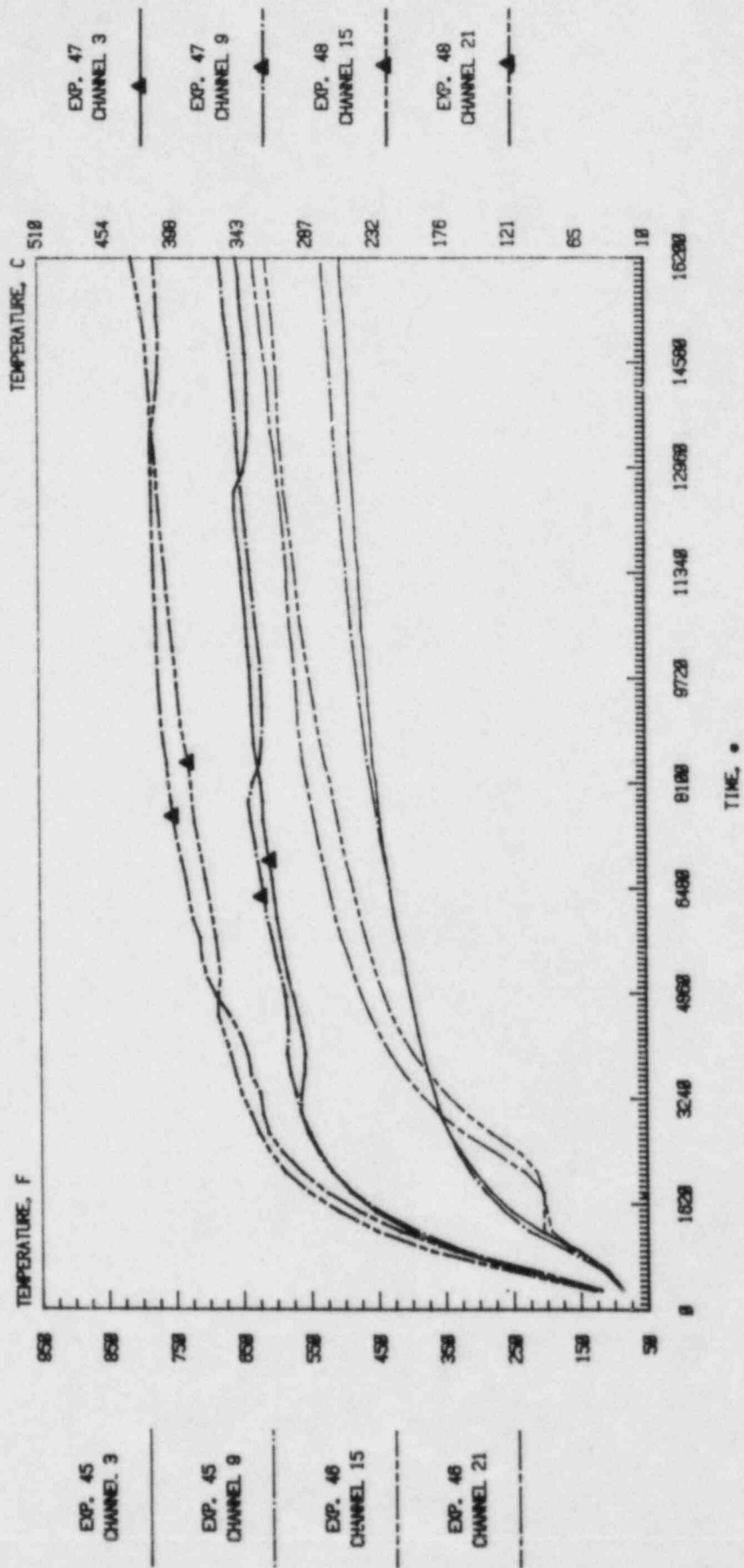
Figure 19 - Unexposed Surface Temperatures; Exps. 45, 46, 47 and 48
