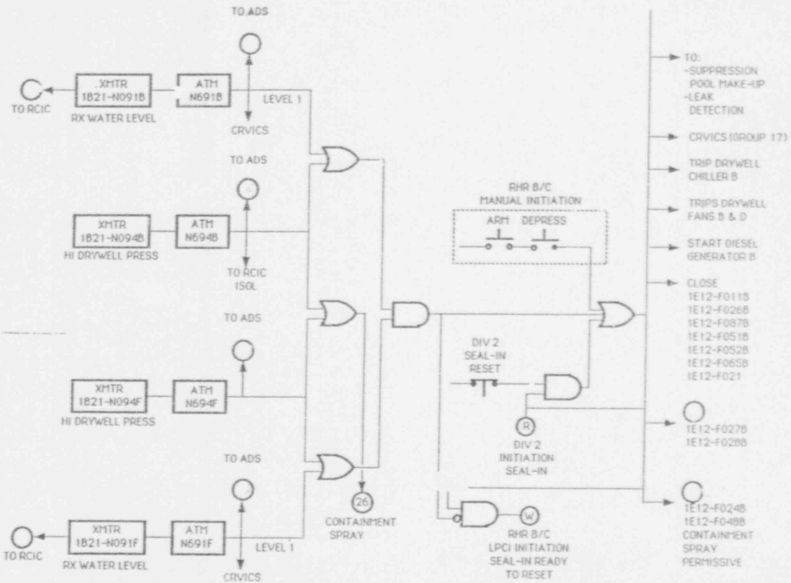
Figure 3.2-8 Division 2 Initiation Logic Sheet 1
