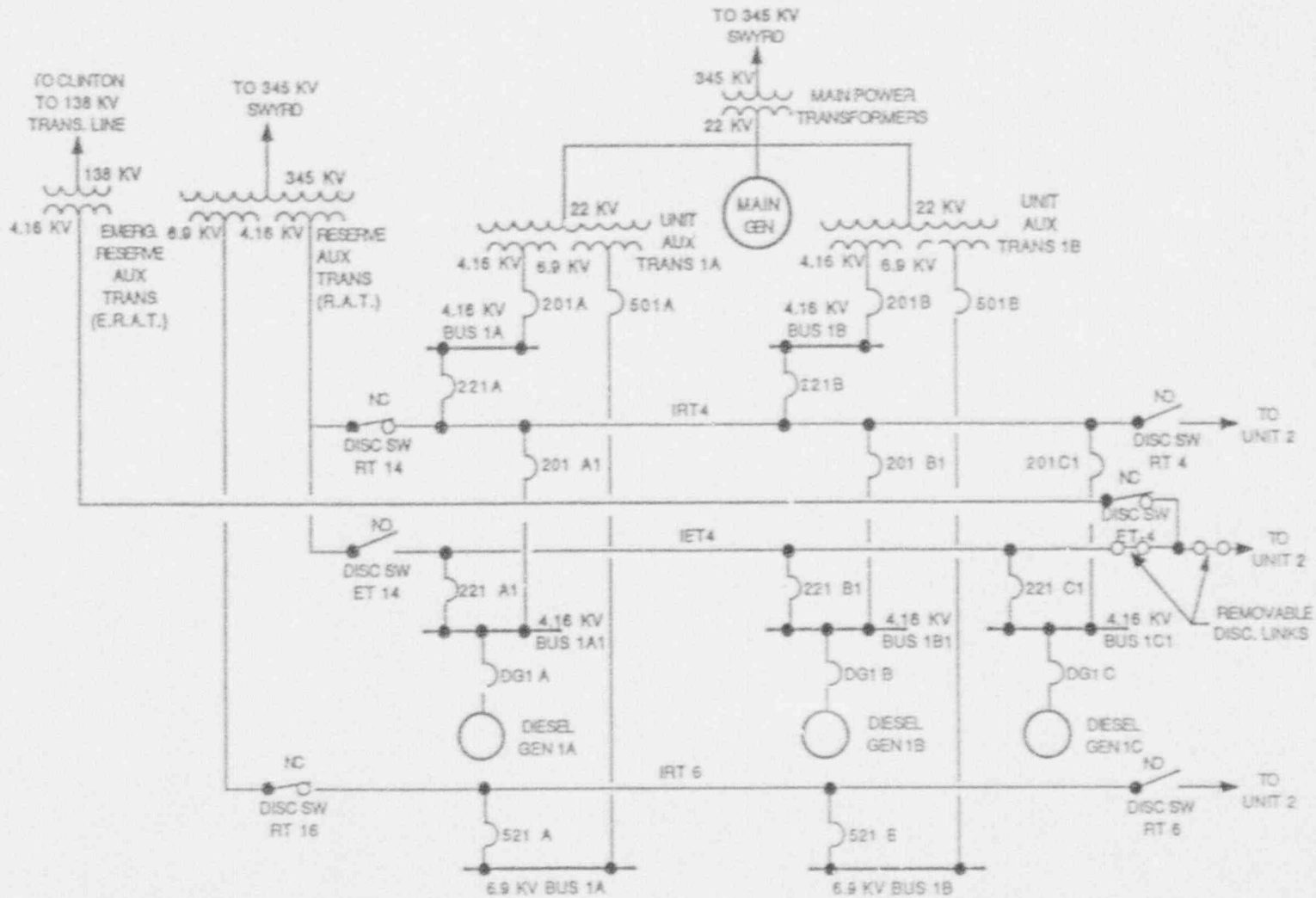
Figure 3.2-33 Auxiliary Power System Sheet 1
