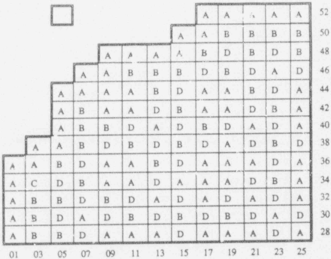
FIGURE 8.4.a CYCLE 11 LOADING PATTERN, UPPER LEFT QUADRANT, BUNDLE DESIGN
