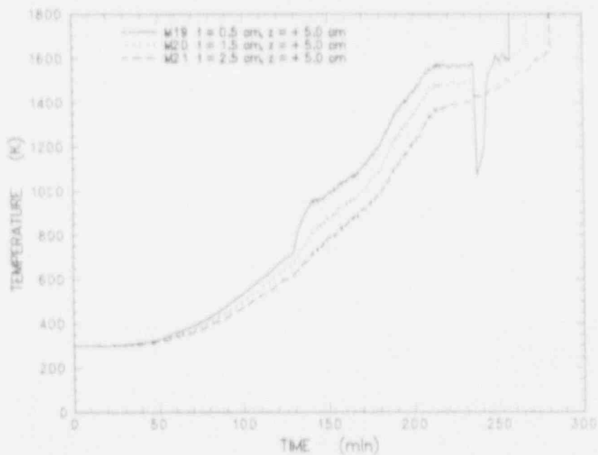
Figure C-21 MgO sidewall temperature data measured by thermocouples in the array located at z = +5.0 cm
