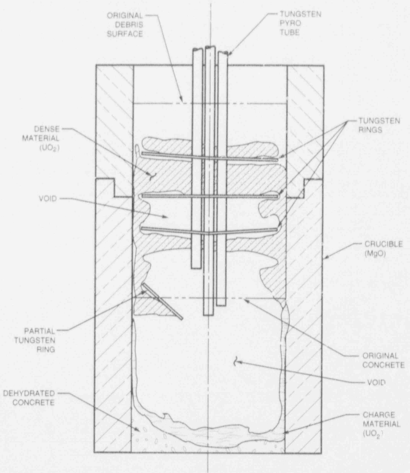
Figure 5.3 Drawing of posttest x-ray of SURC-2
