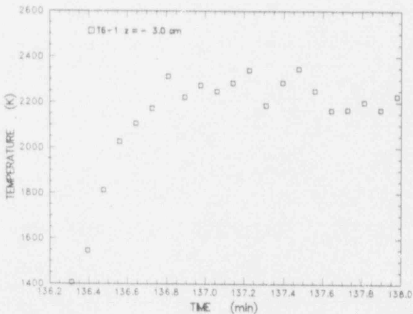
Figure D-20 Expansion of meltpool temperature data measured by a C type thermocouple installed in an alumina tube cast into the concrete at z = -3.0 cm
