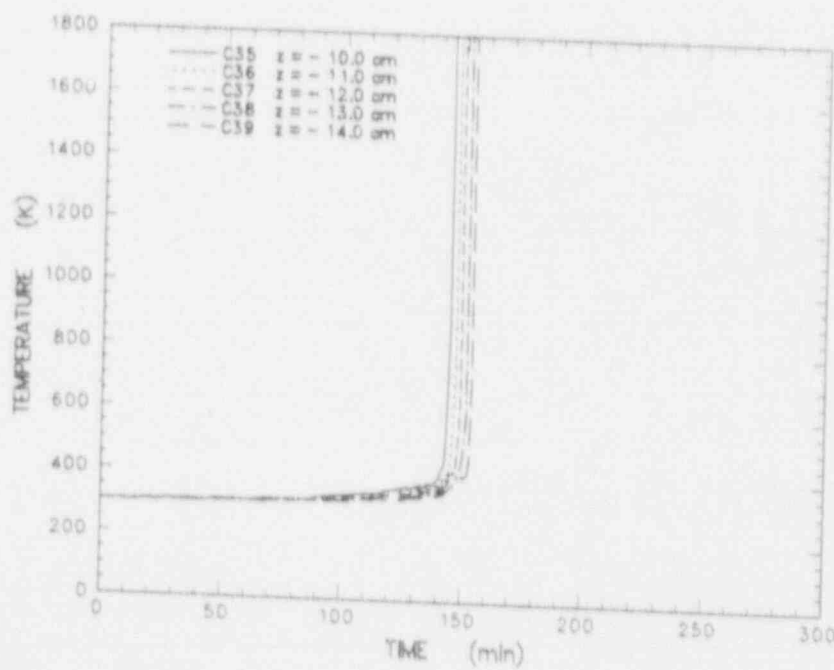
Figure C-8 Concrete temperature data measured by thermocouples located in the midradius array between z = -10.0 and -14.0 cm
