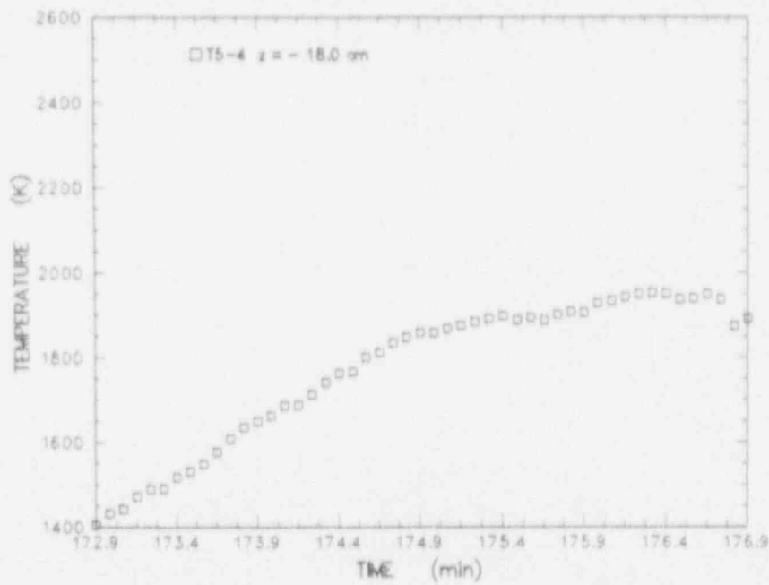
Figure D-19 Expansion of meltpool temperature data measured by a S type thermocouple installed in an alumina tube cast into the concrete at z = -18.0 cm
