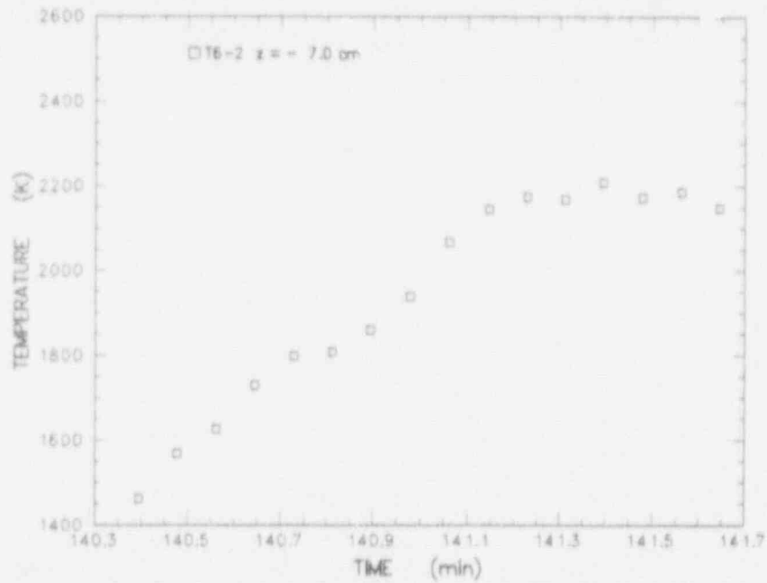
Figure D-21 Expansion of meltpool temperature data measured by a C type thermocouple installed in an alumina tube cast into the concrete at z = -7.0 cm
