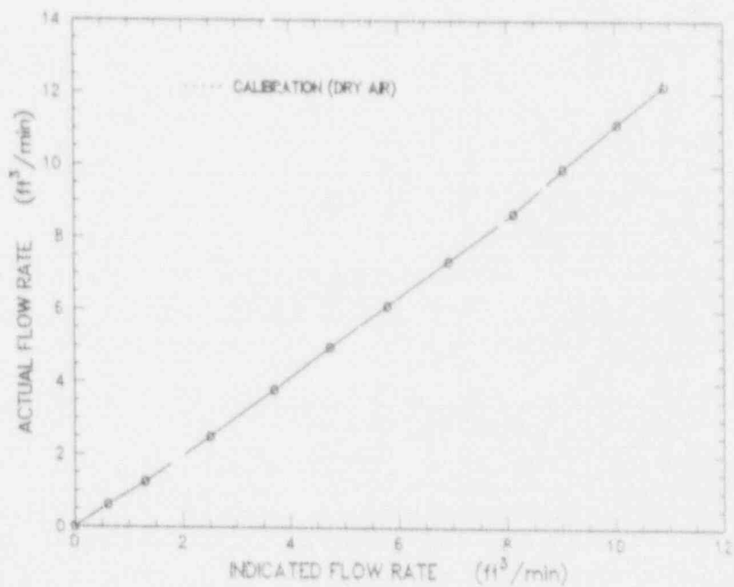
Figure F-14 Calibration of the Rockwell 415 positive displacement gas clock (meter)
