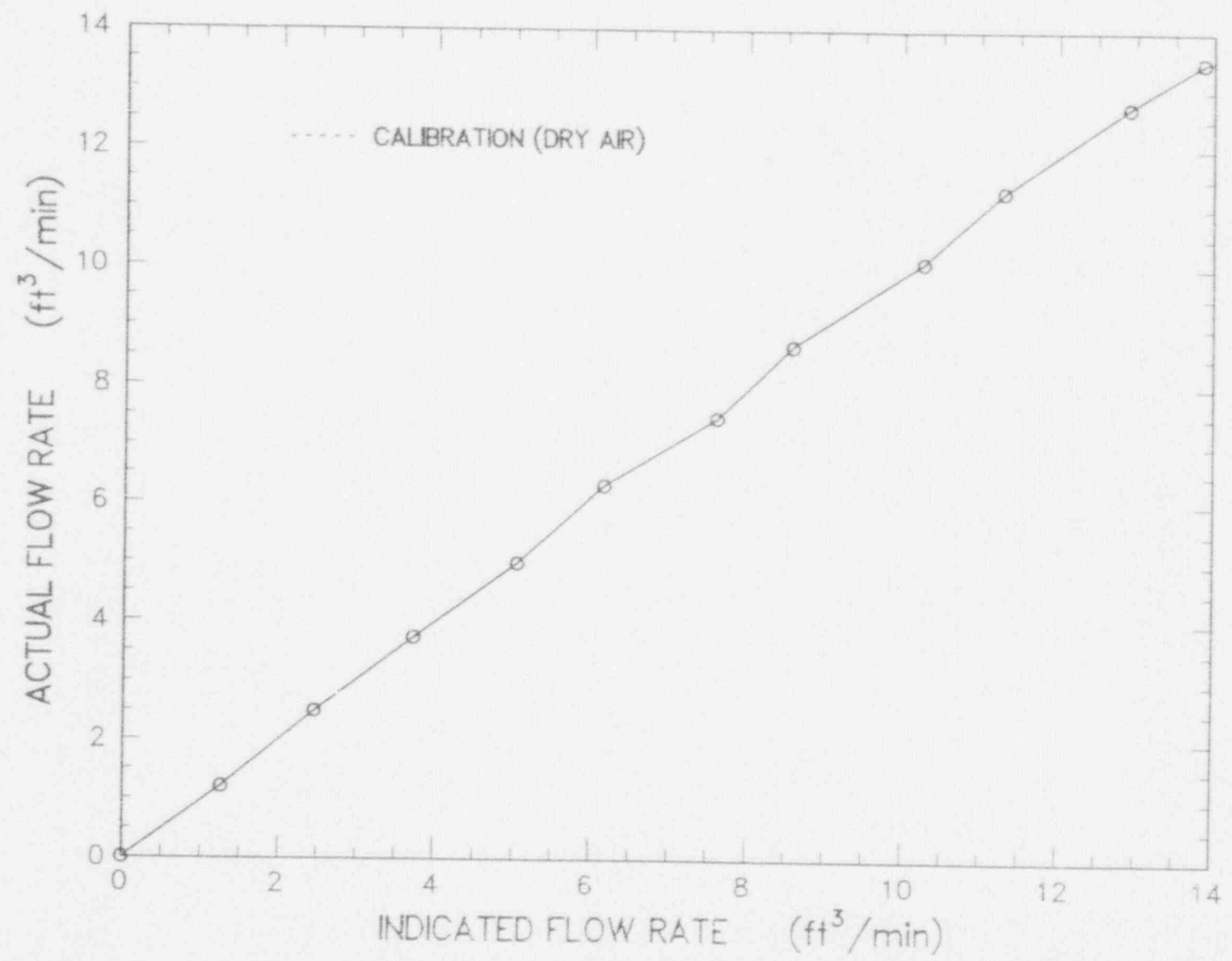
Figure 4.3.6 Rockwell 750 calibration
