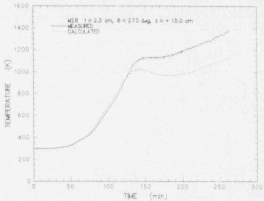
Figure E-37 Comparison of sidewall temperatures measured during the experiment and calculated from the heat flux code for thermocouple located at z = +15.0 cm and t = 2.5 cm
