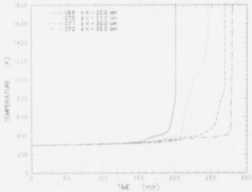
Figure C-15 Concrete temperature data measured by thermocouples in the perimeter array between z = -20.0 and -35.0 cm
