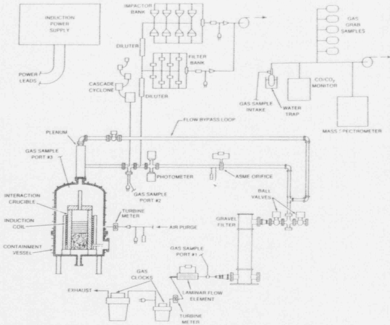
Figure 4.3.1 Flow train schematic
