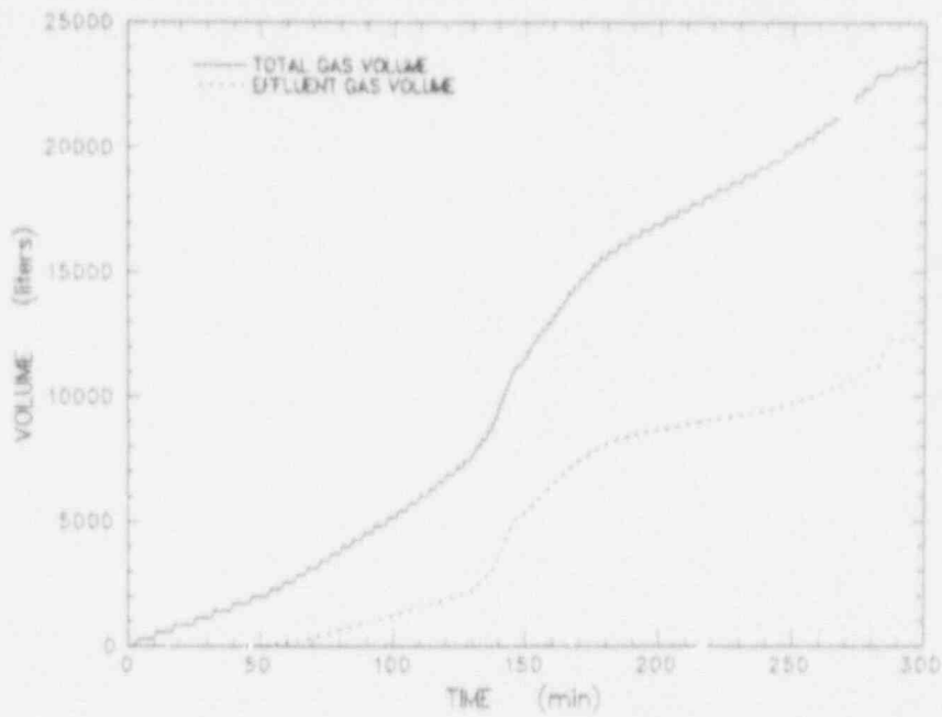
Figure G-7 Comparison of total gas volume measured by the Rockwell 750 gas meter and the reaction gas volume calculated from flow device data
