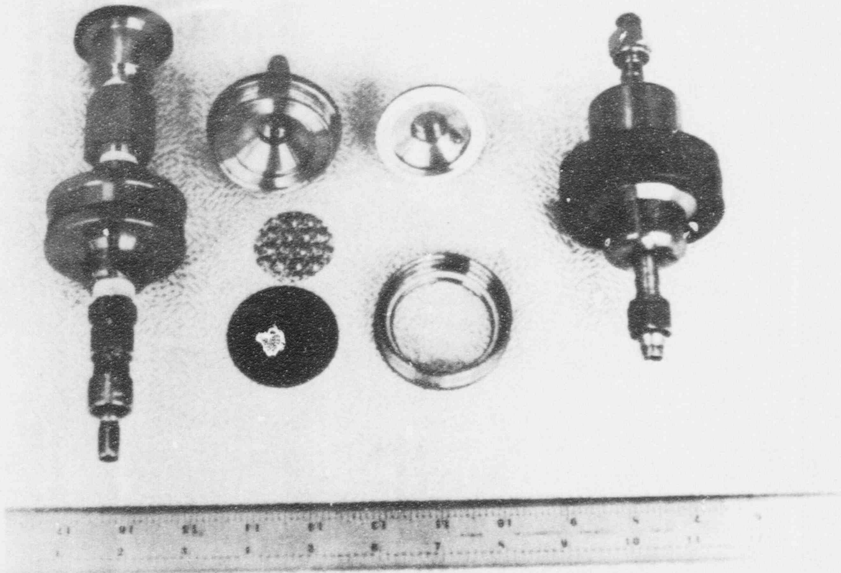
Figure 4.4.9 The Gelman high pressure filter holder shown disassembled with filter substrate support (left) and filter substrate and supports in place (right)
