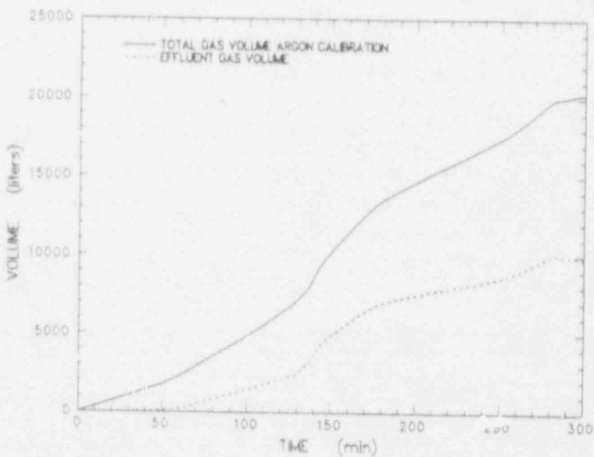
Figure G-8 Comparison of total gas volume calculated using laminar flow device data (argon cal.) and the reaction gas volume calculated from flow device data
