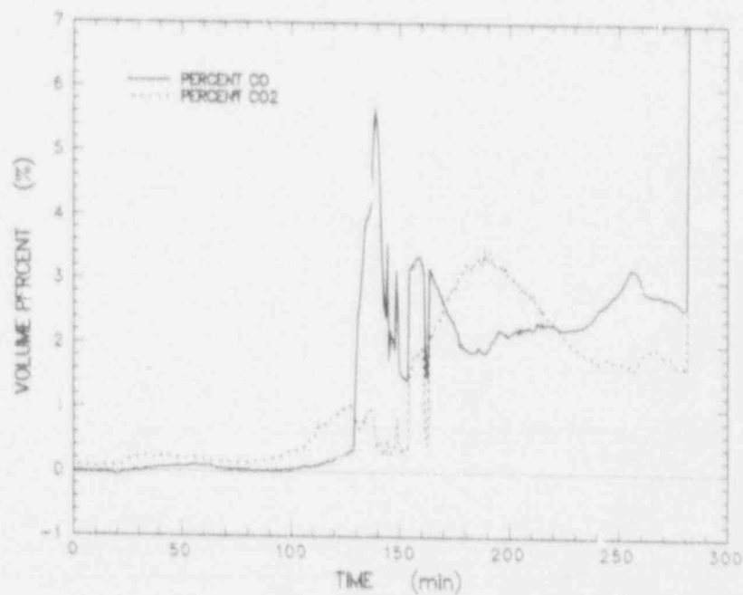
Figure G-16 Volume percent CO and CO 2 measured using the infrared gas monitor
