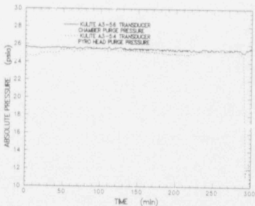
Figure G-12 Absolute pressure measured upstream of the 14 and 3 lpm critical orifice metering argon purge gas flowing into the containment vessel and tungsten pyrotubes
