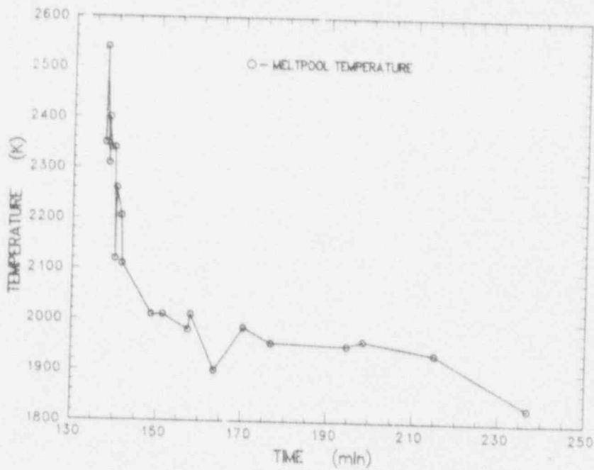
Figure D-28 Meltpool temperature summary
