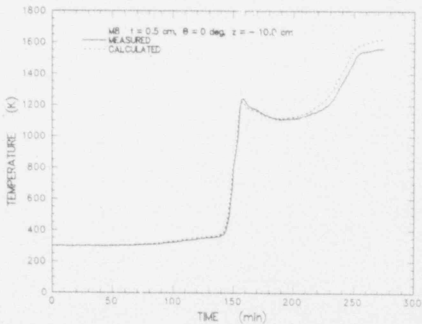
Figure E-20 Comparison of sidewall temperatures measured during the experiment and calculated from the heat flux code for the thermocouple located at z = -10.0 cm and t = 0.5 cm
