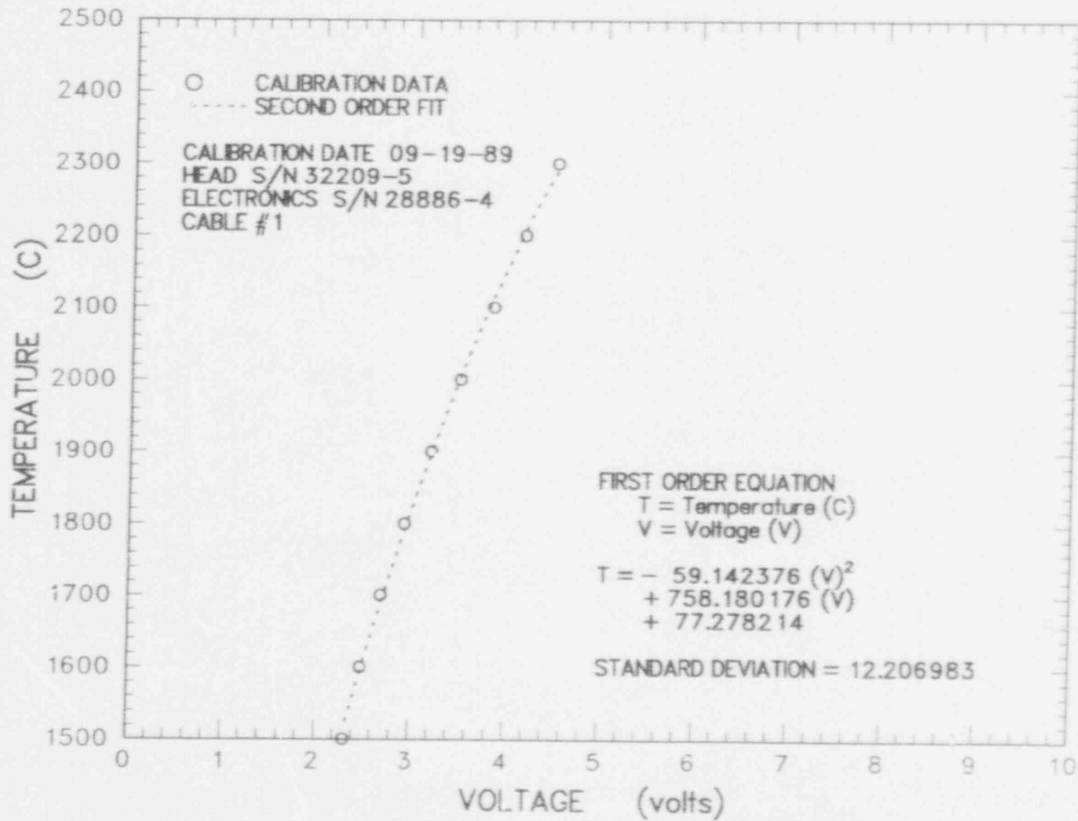
Figure 4.1.5 Micron fiber optic pyrometer calibration, pyrotube elevation Z = +0 cm
