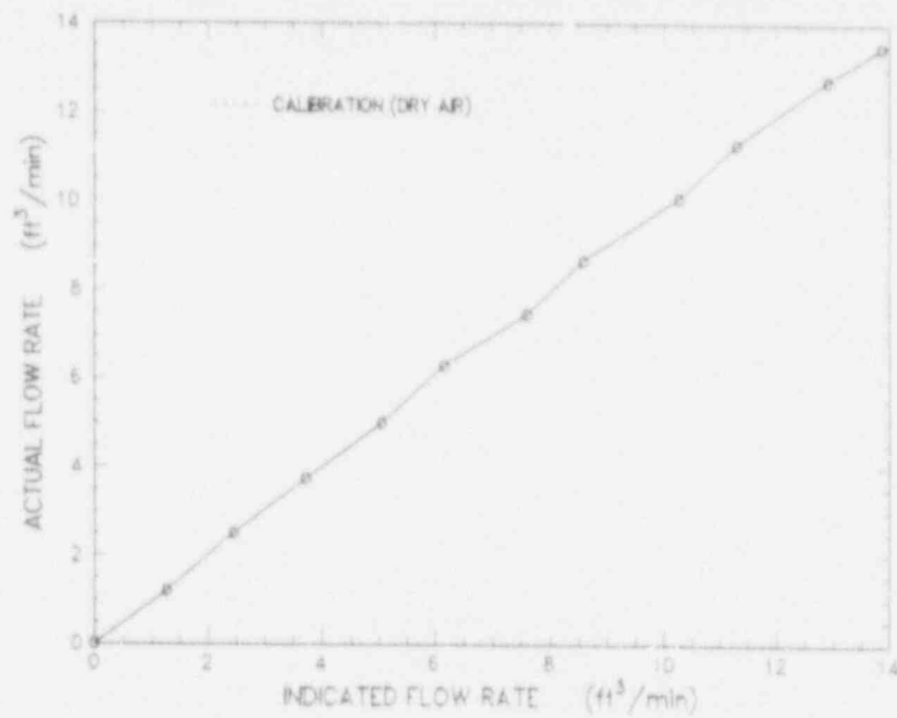
Figure F-15 Calibration of the Rockwell 750 positive displacement gas clock (meter)
