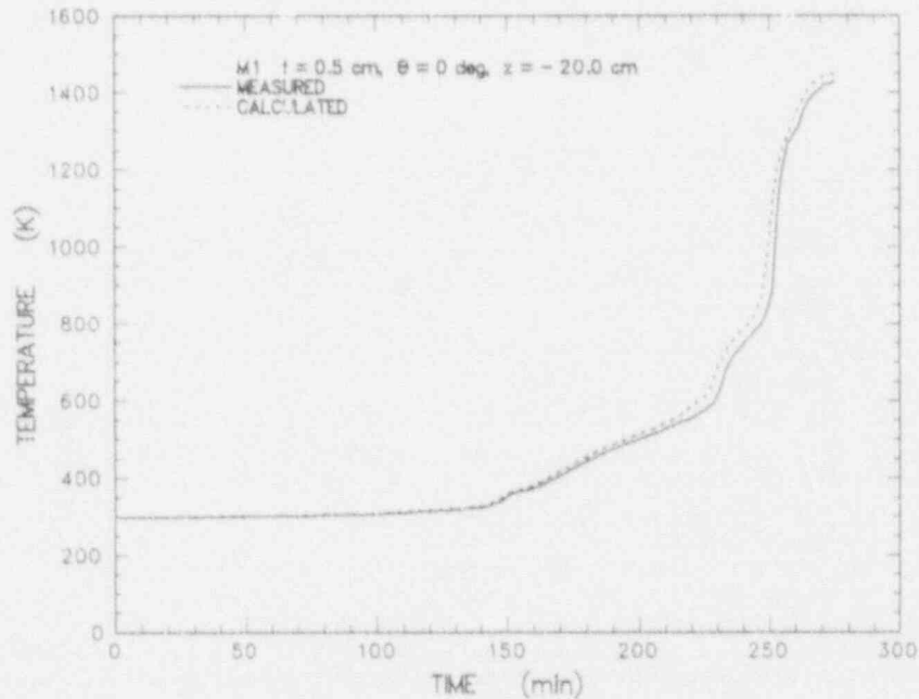
Figure E-14 Comparison of sidewall temperatures measured during the experiment and calculated from the heat flux code for the thermocouple located at z = -20.0 cm and t = 0.5 cm
