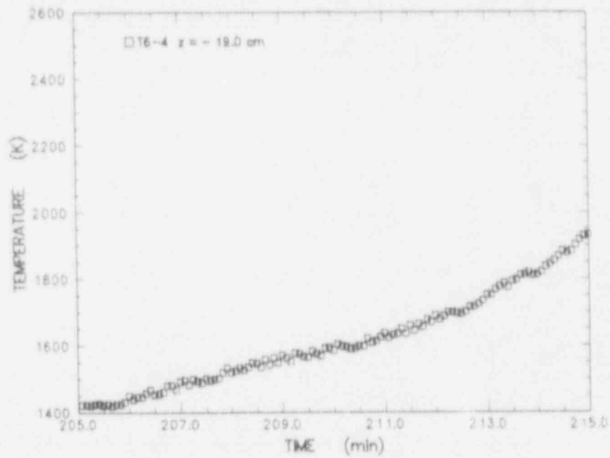
Figure D-23 Expansion of melt pool temperature data measured by a S type thermocouple installed in an Alumina tube cast into the concrete at z \approx -19.0 cm
