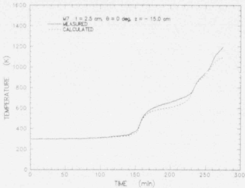
Figure E-19 Comparison of sidewall temperatures measured during the experiment and calculated from the heat flux code for thermocouple located at z = -15.0 cm and t = 2.5 cm
