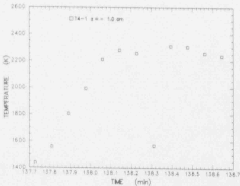
Figure D-12 Expansion of meltpool temperature data measured by a C type thermocouple installed in an alumina tube cast into the concrete at z = -1.0 cm
