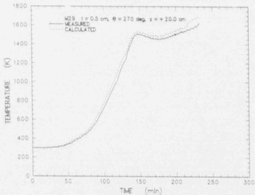
Figure E-38 Comparison of sidewall temperatures measured during the experiment and calculated from the heat flux code for the thermocouple located at z = +20.0 cm and t = 0.5 cm
