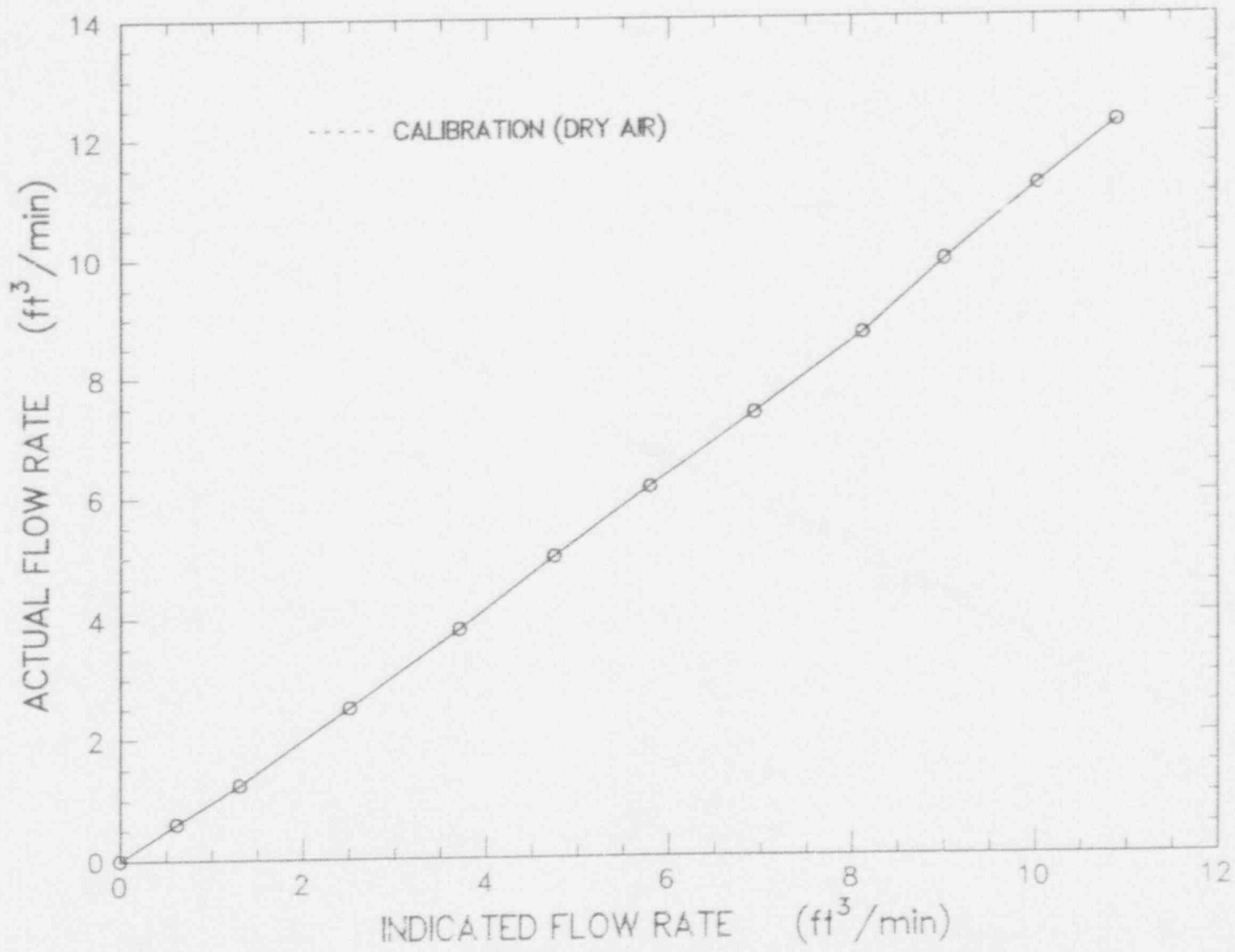
Figure 4.3.5 Rockwell 415 calibration
