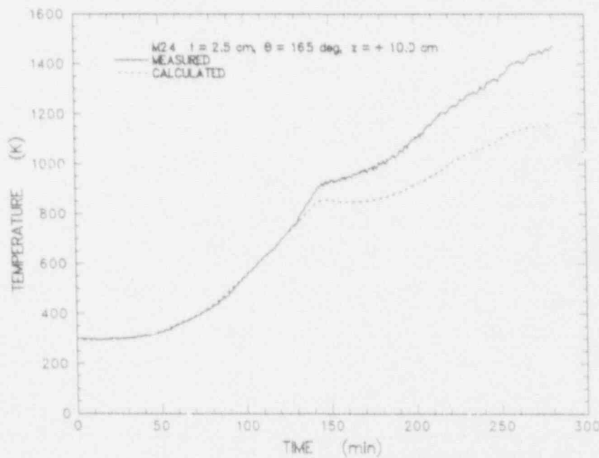
Figure E-34 Comparison of sidewall temperatures measured during the experiment and calculated from the heat flux code for the thermocouple located at z = +10.0 cm and t = 2.5 cm
