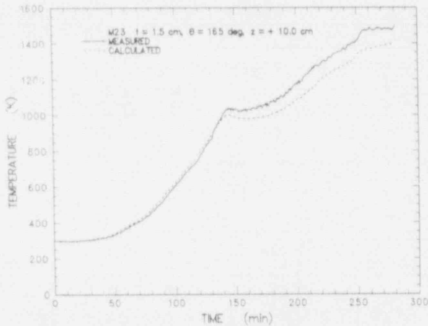
Figure E-33 Comparison of sidewall temperatures measured during the experiment and calculated from the heat flux code for thermocouple located at z = +10.0 cm and t = 1.5 cm
