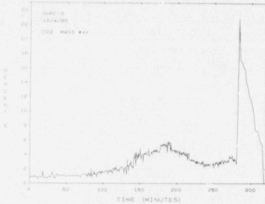
Figure G-33 Volume percent of carbon dioxide measured by the mass spectrometer
