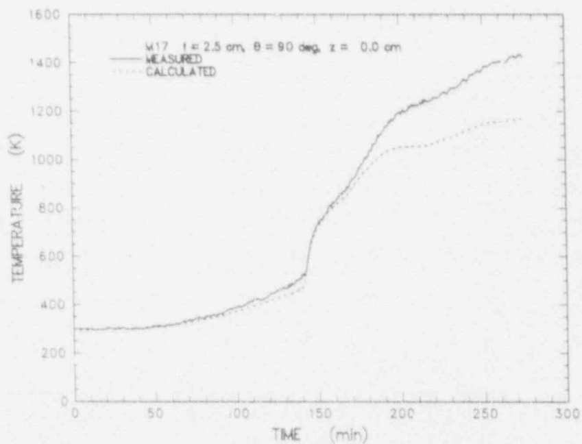
Figure E-28 Comparison of sidewall temperatures measured during the experiment and calculated from the heat flux code for the thermocouple located at z = 0.0 cm and t = 2.5 cm
