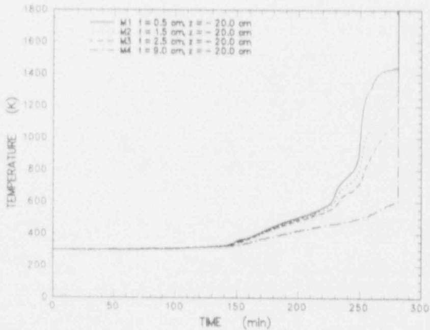
Figure C-16 MgO sidewall temperature data measured by thermocouples in the array located at z = -20.0 cm
