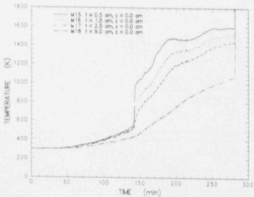
Figure C-20 MgO sidewall temperature data measured by thermocouples in the array located at z = 0.0 cm
