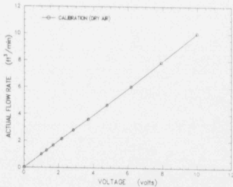
Figure F-16 Turbine meter calibration installed downstream of the laminar flow element near the exit of the flow circuit
