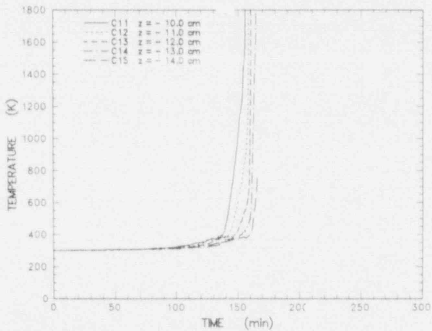
Figure C-3 Concrete temperature data measured by thermocouples located in the axial centerline array between z = -10.0 and -14.0 cm
