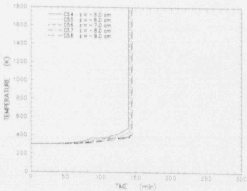
Figure C-12 Concrete temperature data measured by thermocouples located in the perimeter array between z = -5.0 and -9.0 cm
