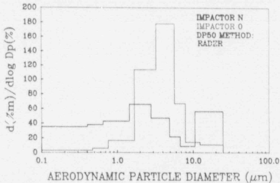
Figure G-43 Normalized aerosol mass distribution from impactors N and O taken between 164.0 and 164.5 minutes
