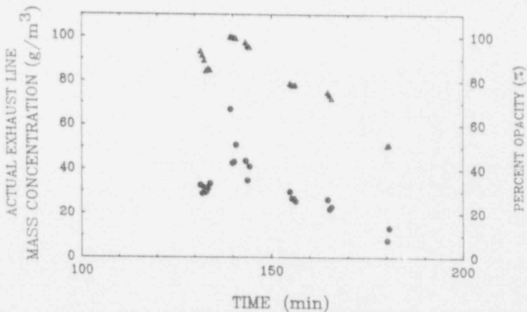
Figure G-46 Filter data comparing percent opacity with actual exhaust line mass concentration
