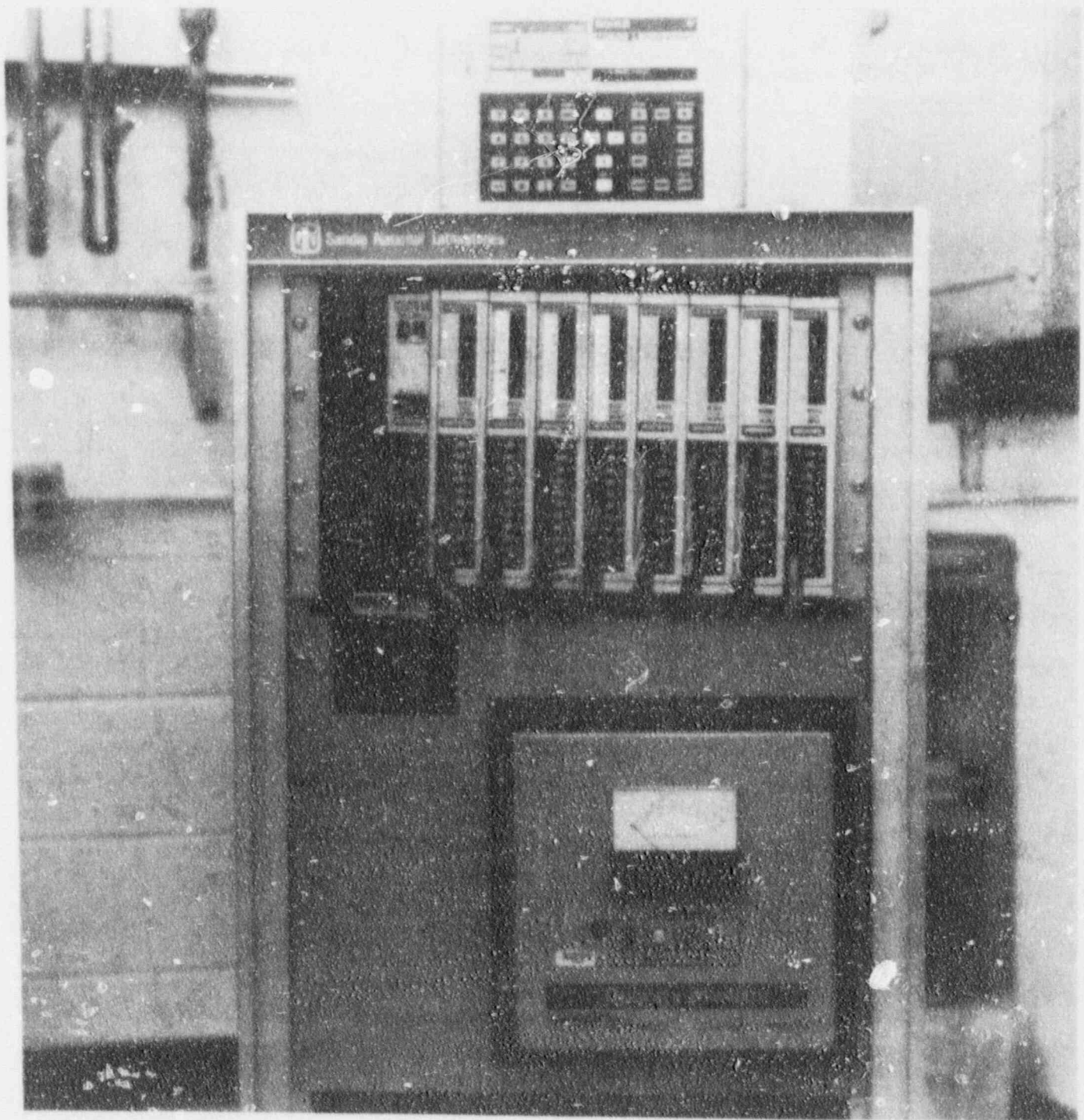
Figure 4.4.5 Modicon Micro 84 programmable controller shown with the control/programming unit sitting atop the switching section
