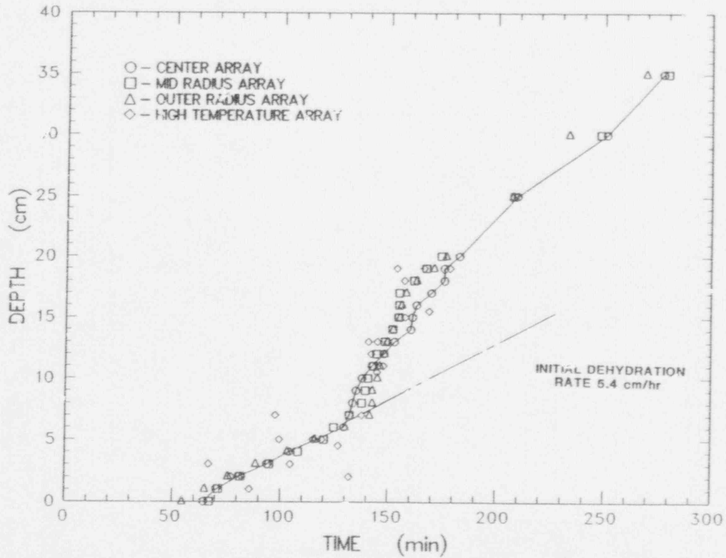
Figure 3.4 Location of the dehydration front for SURC-2
