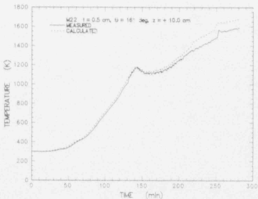
Figure E-32 Comparison of sidewall temperatures measured during the experiment and calculated from the heat flux code for the thermocouple located at z = +10.0 cm and r = 0.5 cm
