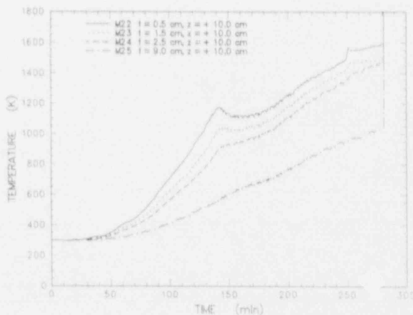
Figure C-22 MgO sidewall temperature data measured by thermocouples in the array located at z = +10.0 cm
