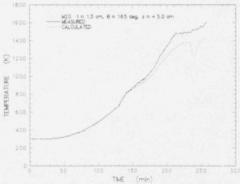
Figure E-30 Comparison of sidewall temperatures measured during the experiment and calculated from the heat flux code for the thermocouple located at z = +5.0 cm and t = 1.5 cm
