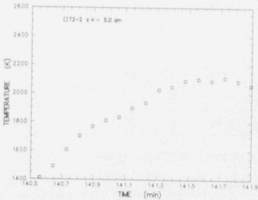
Figure D-6 Expansion of meltpool temperature data measured by a C type thermocouple installed in an alumina tube cast into the concrete at z = -5.0 cm
