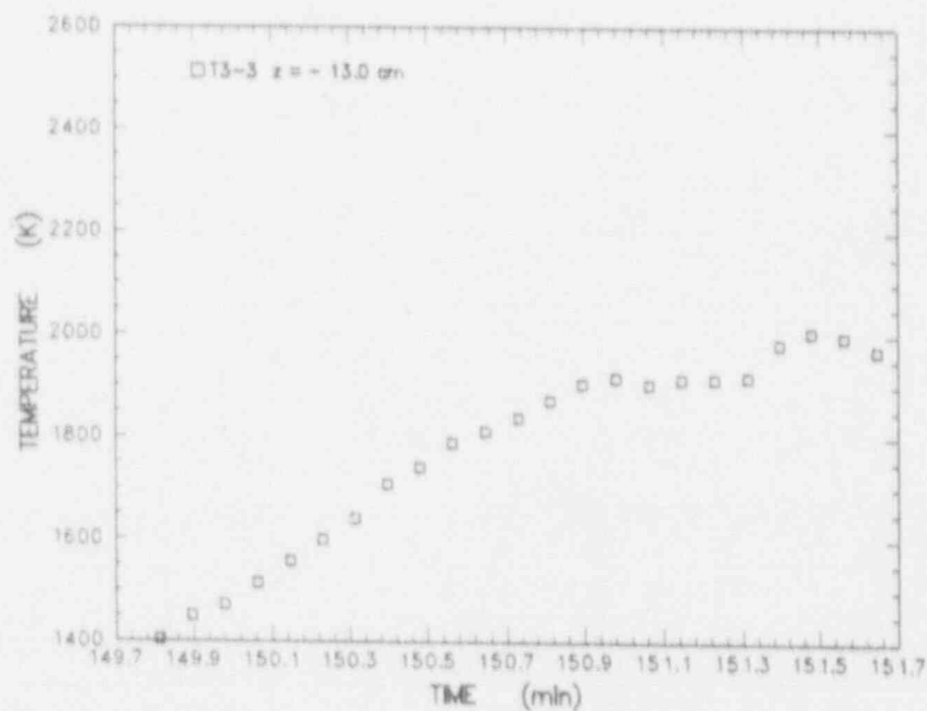
Figure D-10 Expansion of melt pool temperature data measured by a S type thermocouple installed in an alumina tube cast into the concrete at z = -13.0 cm
