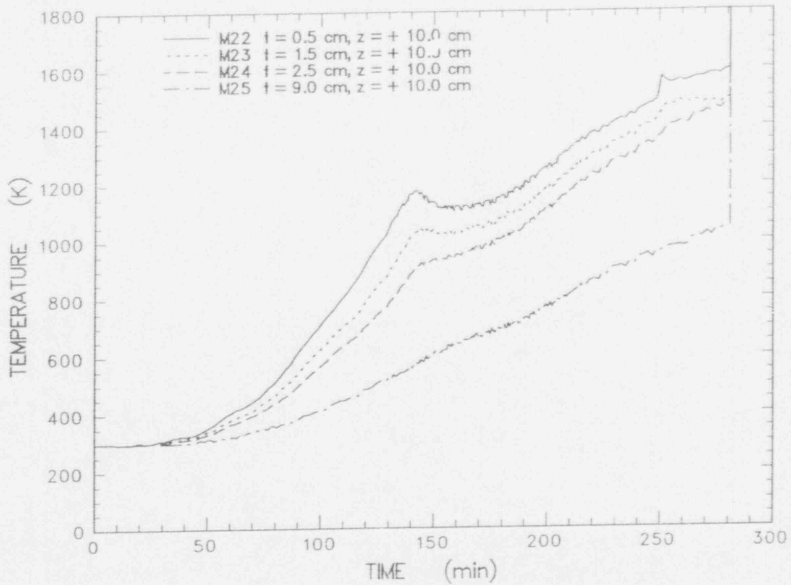
Figure 6.1.14 Typical SURC-2 MgO thermocouple response
