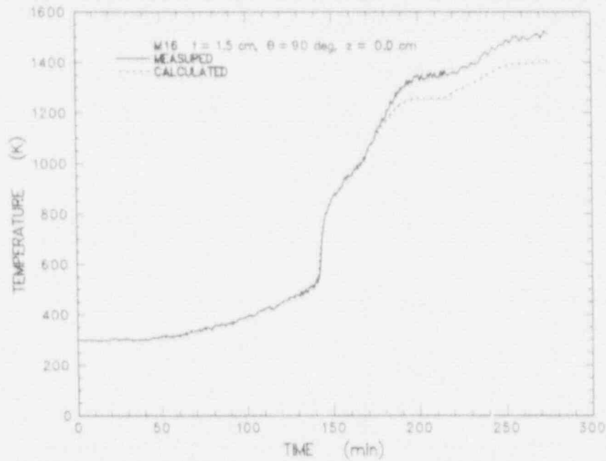
Figure E-27 Comparison of sidewall temperatures measured during the experiment and calculated from the heat flux code for thermocouple located at z = 0.0 cm and t = 1.5 cm
