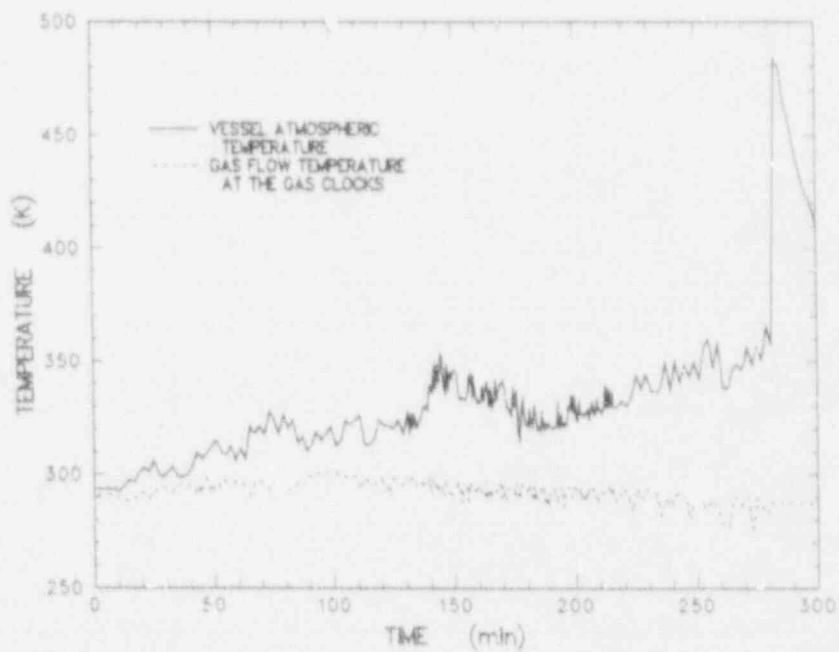
Figure G-14 Atmospheric temperature measured in the containment and in the flow circuit at the 413 positive displacement gas meter
