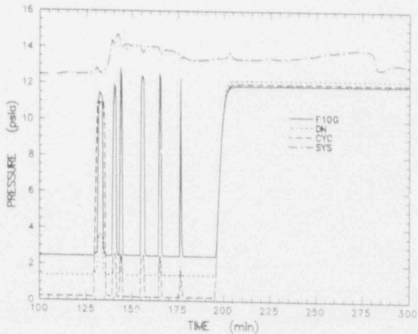
Figure G-38 Absolute pressure measured upstream of critical orifices installed in the aerosol sample line for the filters and cyclone
