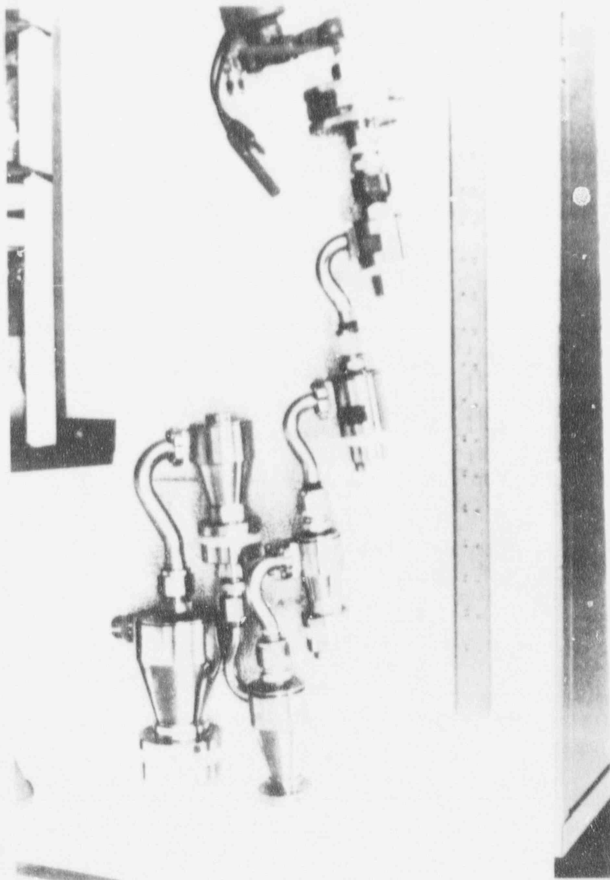
Figure 4.12 Sierra cascade cyclone shown assembled with its six constituent cyclones and backup filter
