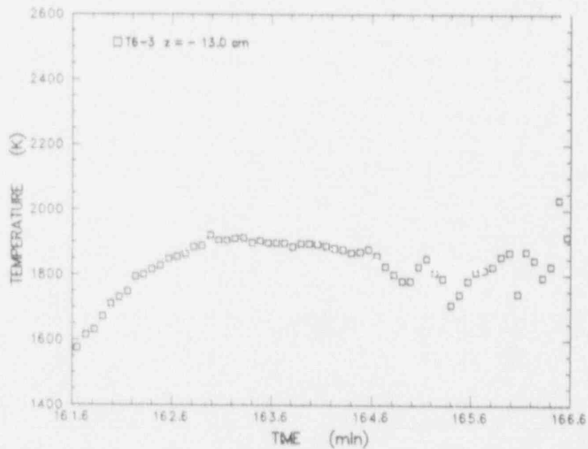
Figure D-22 Expansion of meltpool temperature data measured by a S type thermocouple installed in an alumina tube cast into the concrete at z = -13.0 cm
