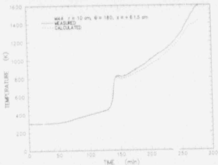
Figure E-51 Comparison of sidewall temperatures measured during the experiment and calculated from the heat flux code for thermocouple located at r = 10.0 cm, \theta = 180 , z = +60.0 cm and t = 1.5 cm
