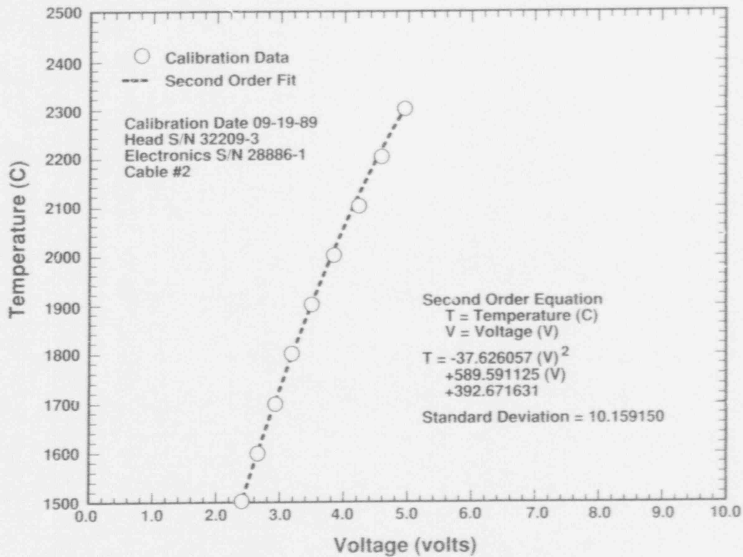
Figure 4.1.4 Micron fiber optic pyrometer calibration, pyrotube elevation Z = +15 c.
