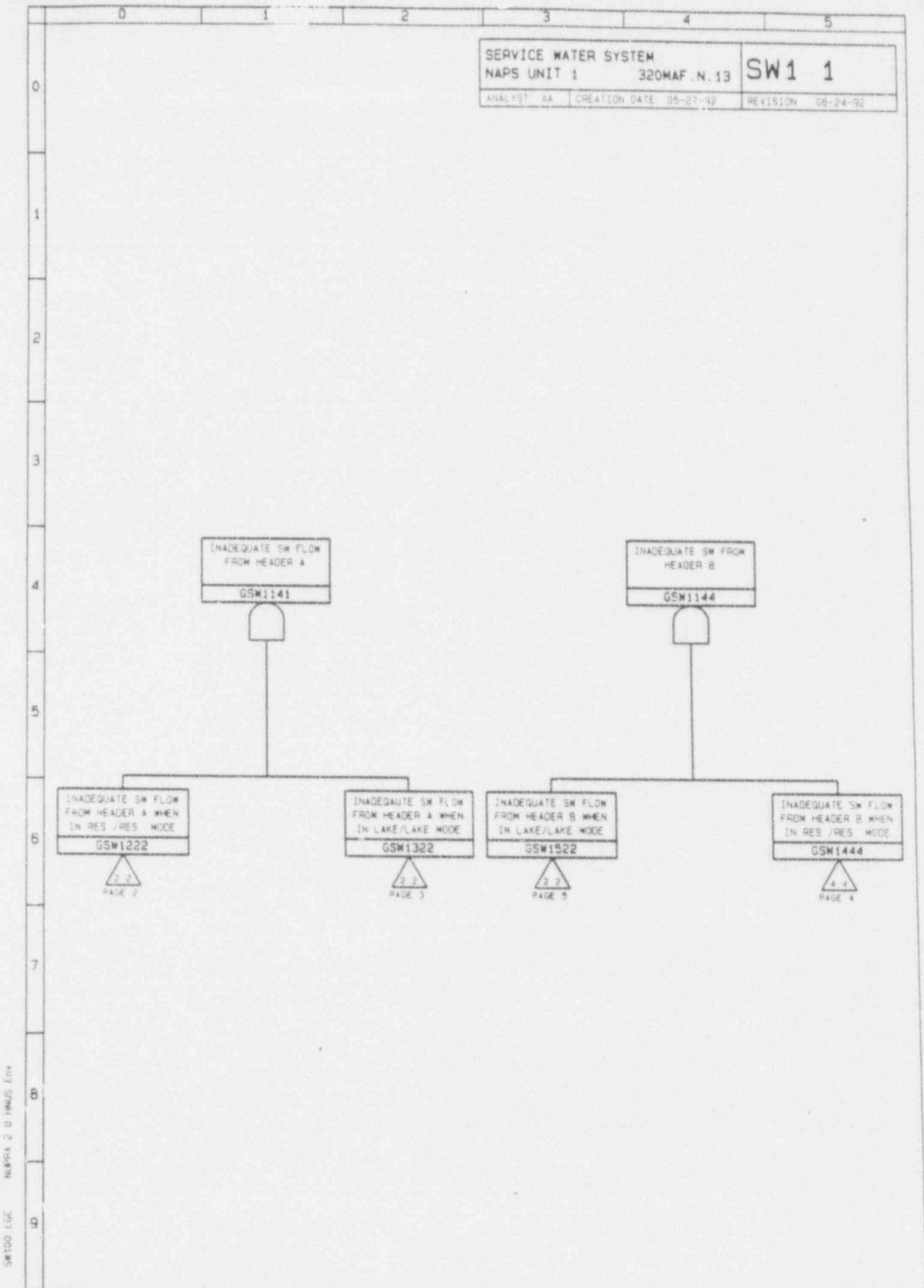
Figure C-2 SW Fault TRee Model
