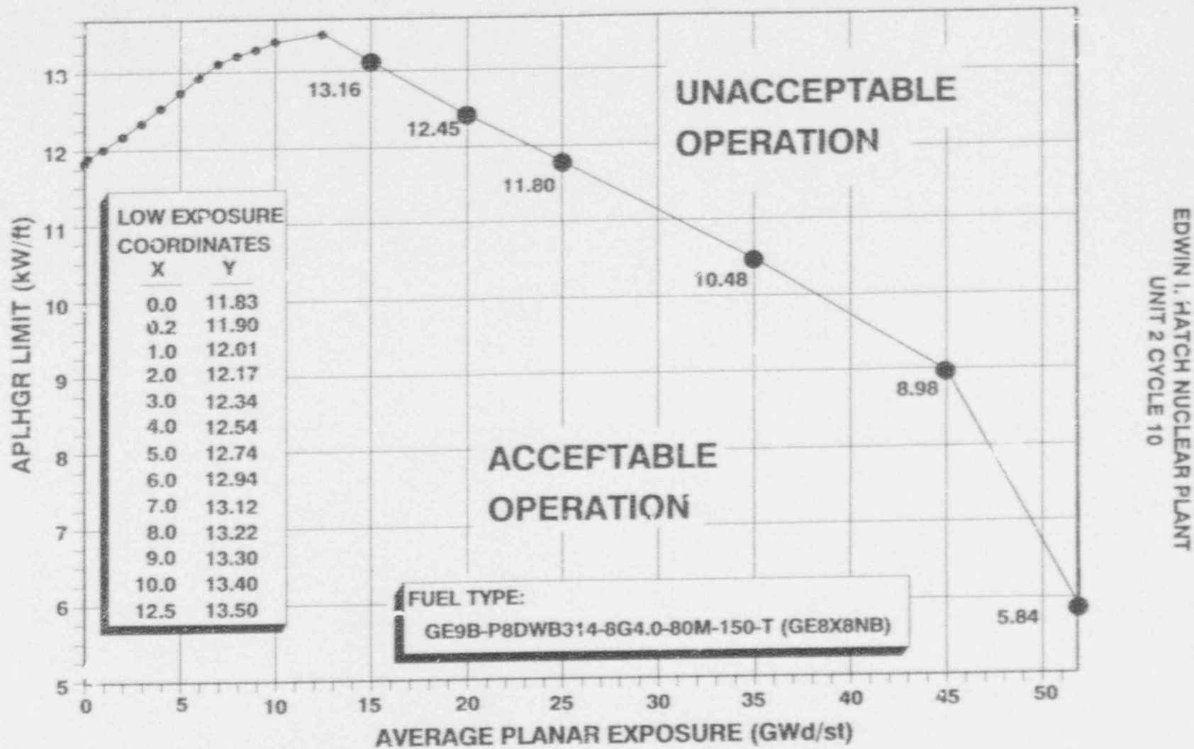
FIGURE 3-6 AVERAGE PLANAR LINEAR HEAT GENERATION RATE LIMIT vs. AVERAGE PLANAR EXPOSURE
