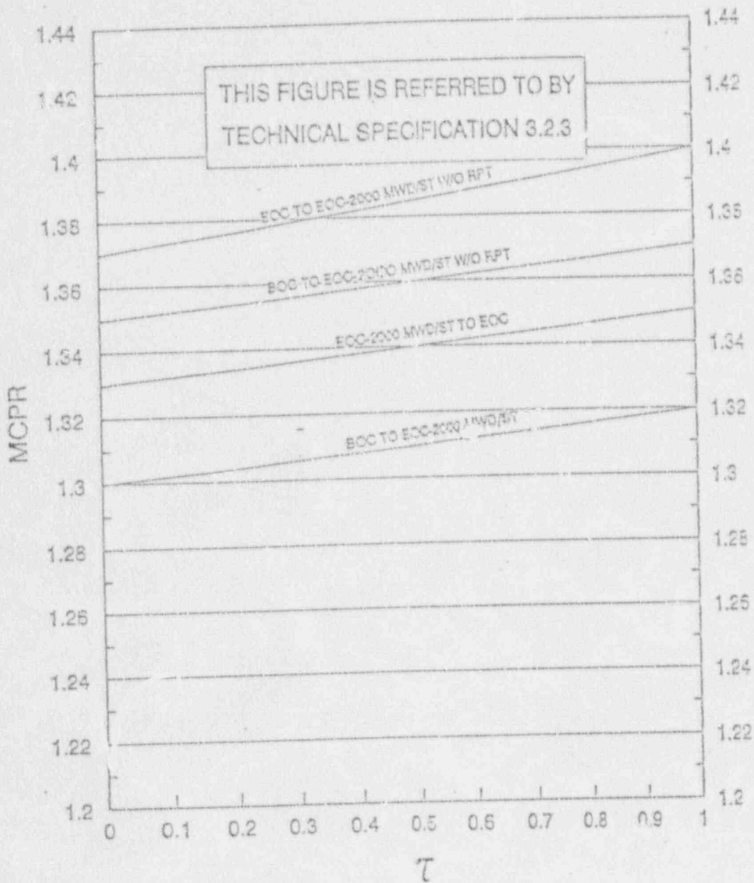
MCPR VS TAU FUEL TYPES GE8X8NB
