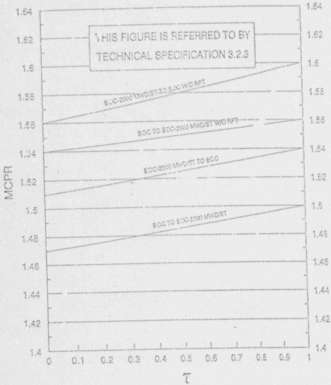
MCPR VS T(A) I FUEL TYPE ABB QFB
