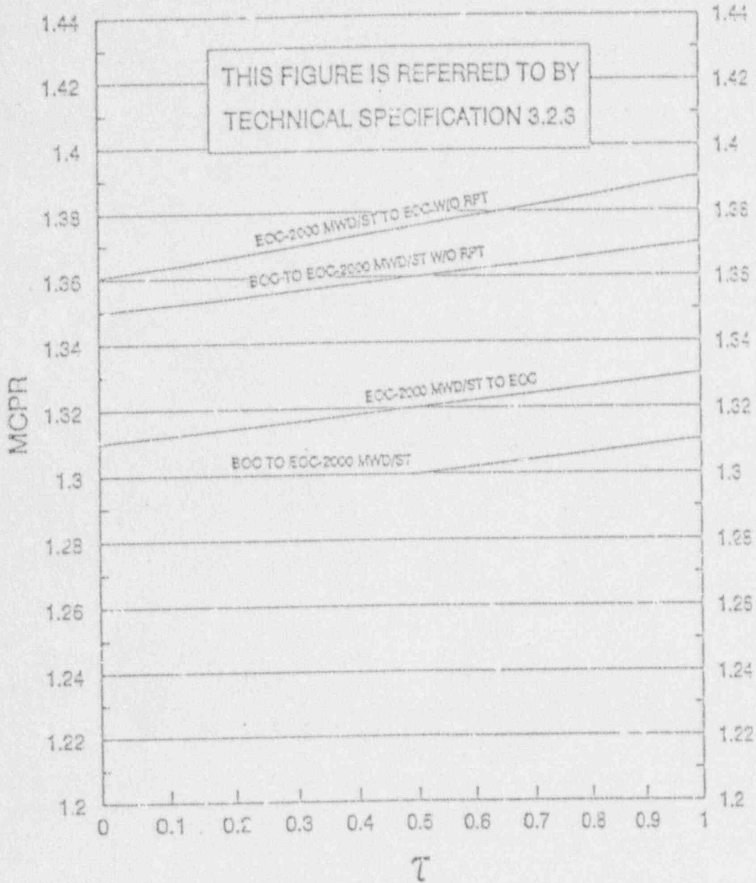
MCPR VS TAU FUEL TYPES BF8X8R
