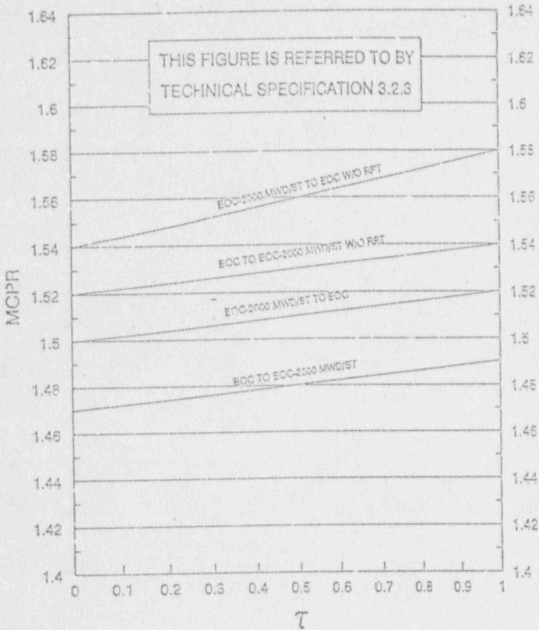
MCPR VS TAU FUEL TYPE ANF QFB
