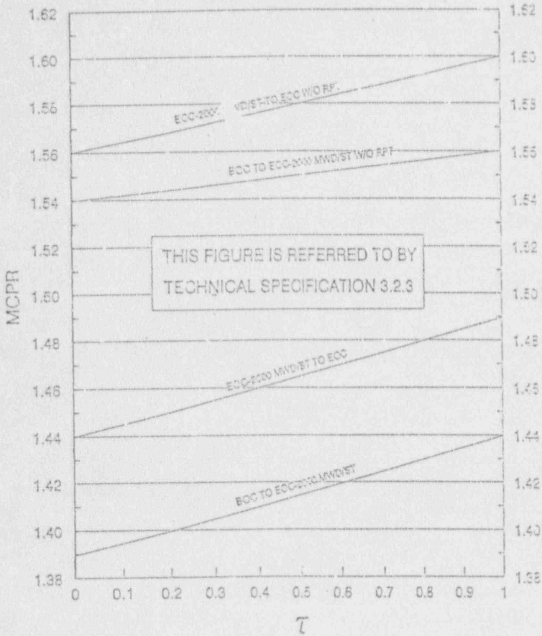
MCPR VS TAU FUEL TYPE ABB QFB
