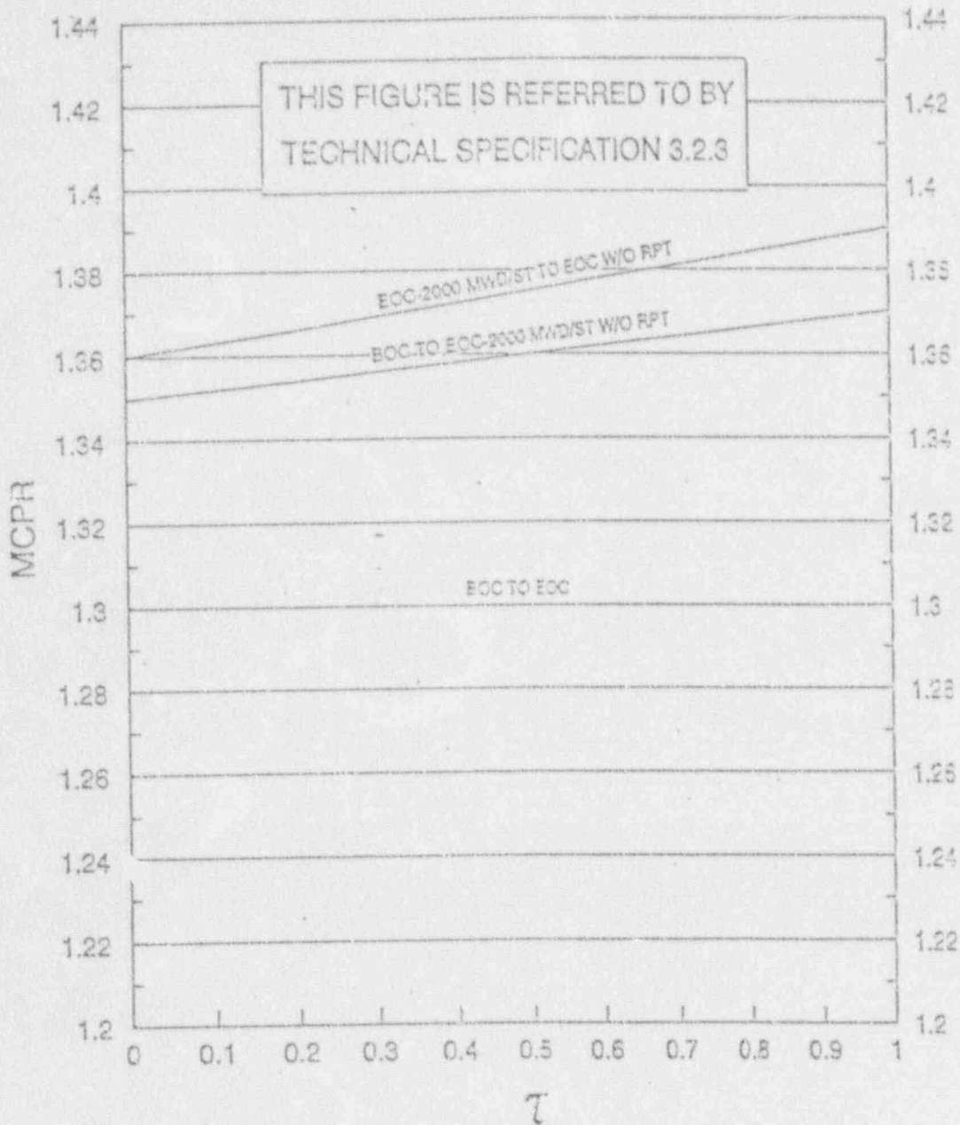
MCPR VS TAU FUEL TYPES BP8X8R
