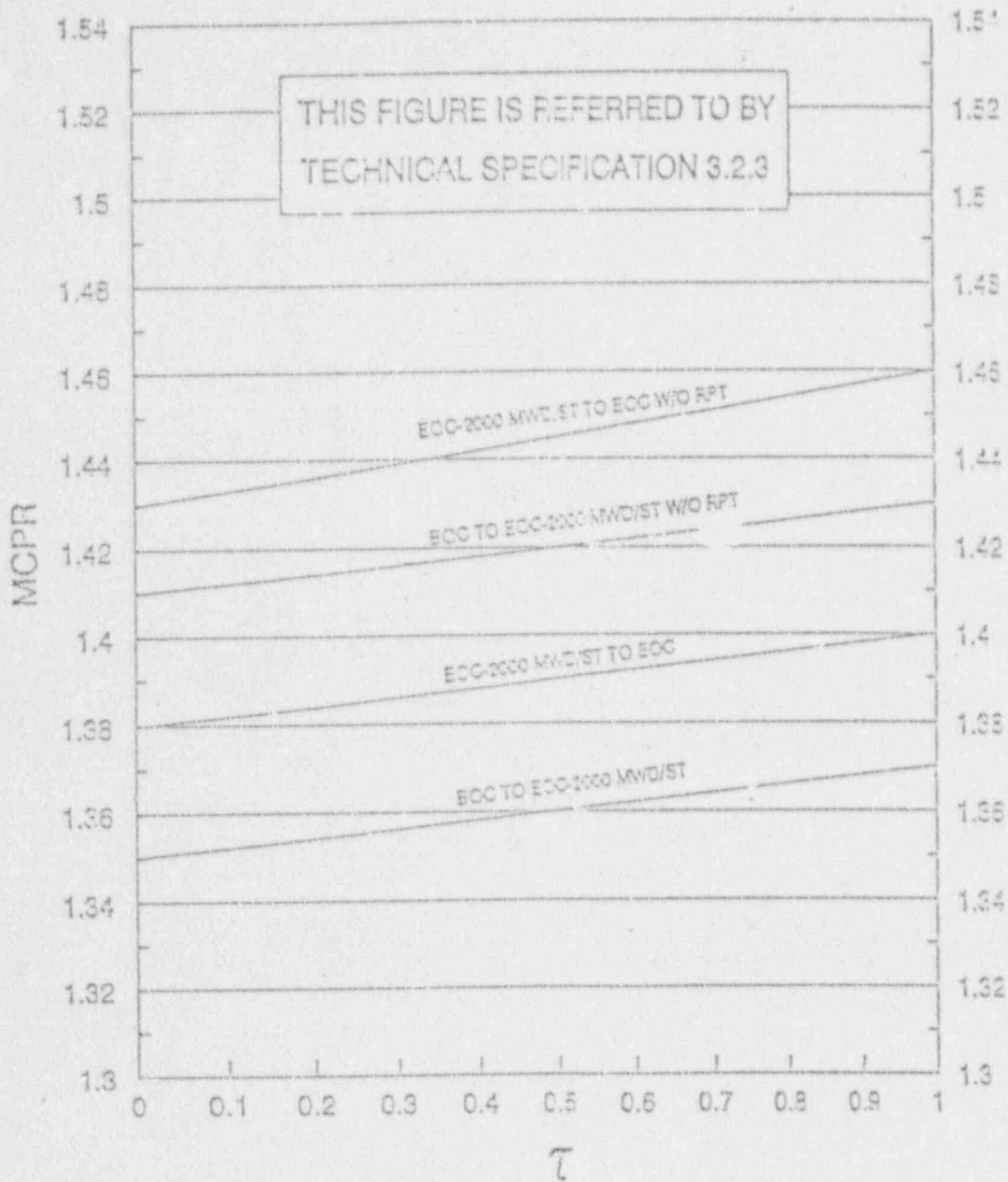
MCPR VS TAU FUEL TYPE GE11
