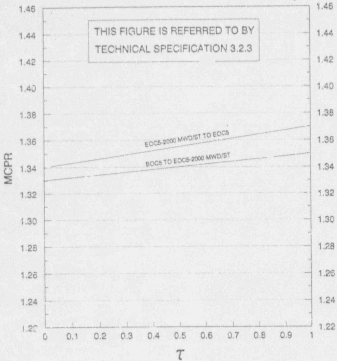
MCPR VS TAU FUEL TYPES GE82WR and BP8x8R (WITHOUT RPT, or WITHOUT RPT and TBVOCS)
