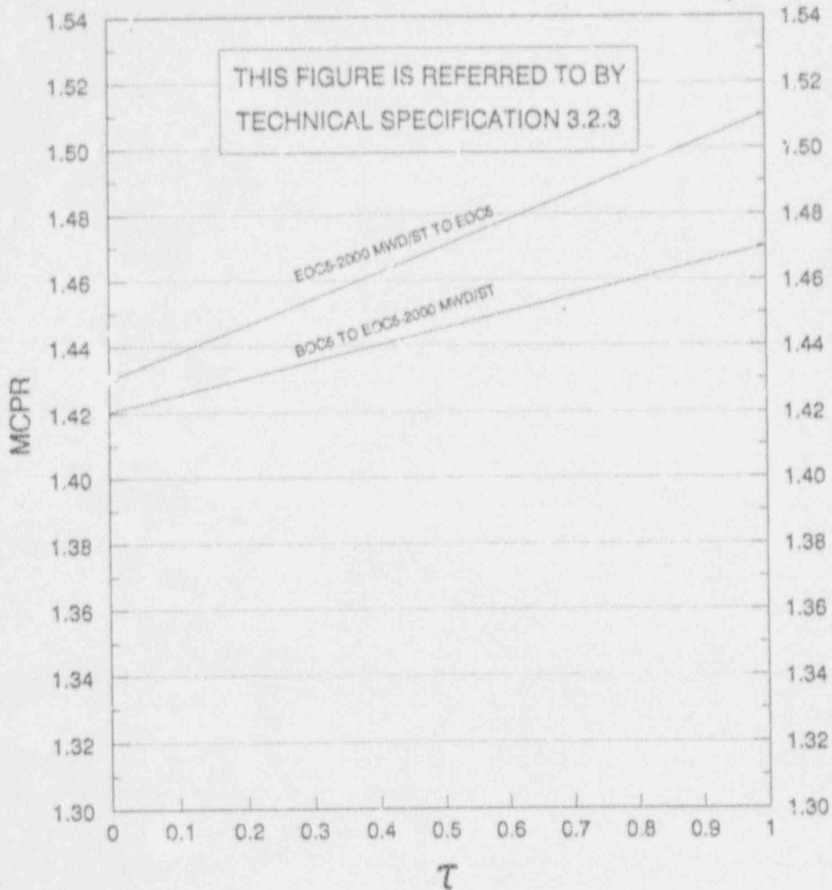
MOPR VS TAU FUEL TYPE GE11
