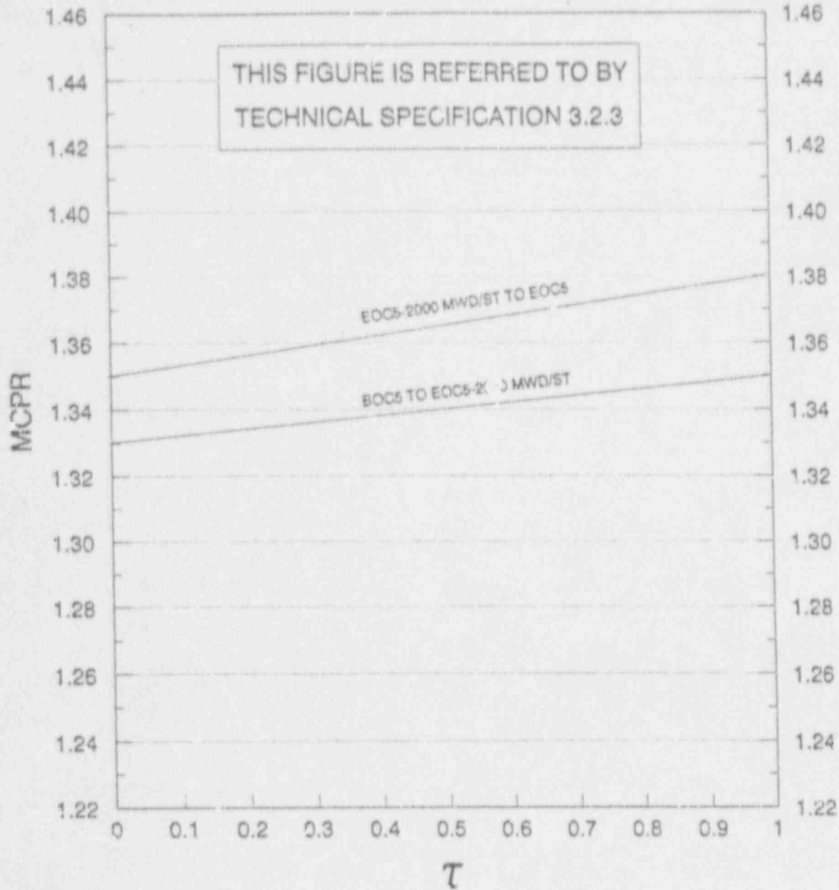
MCPR VS TAU FUEL TYPE GE84WR
