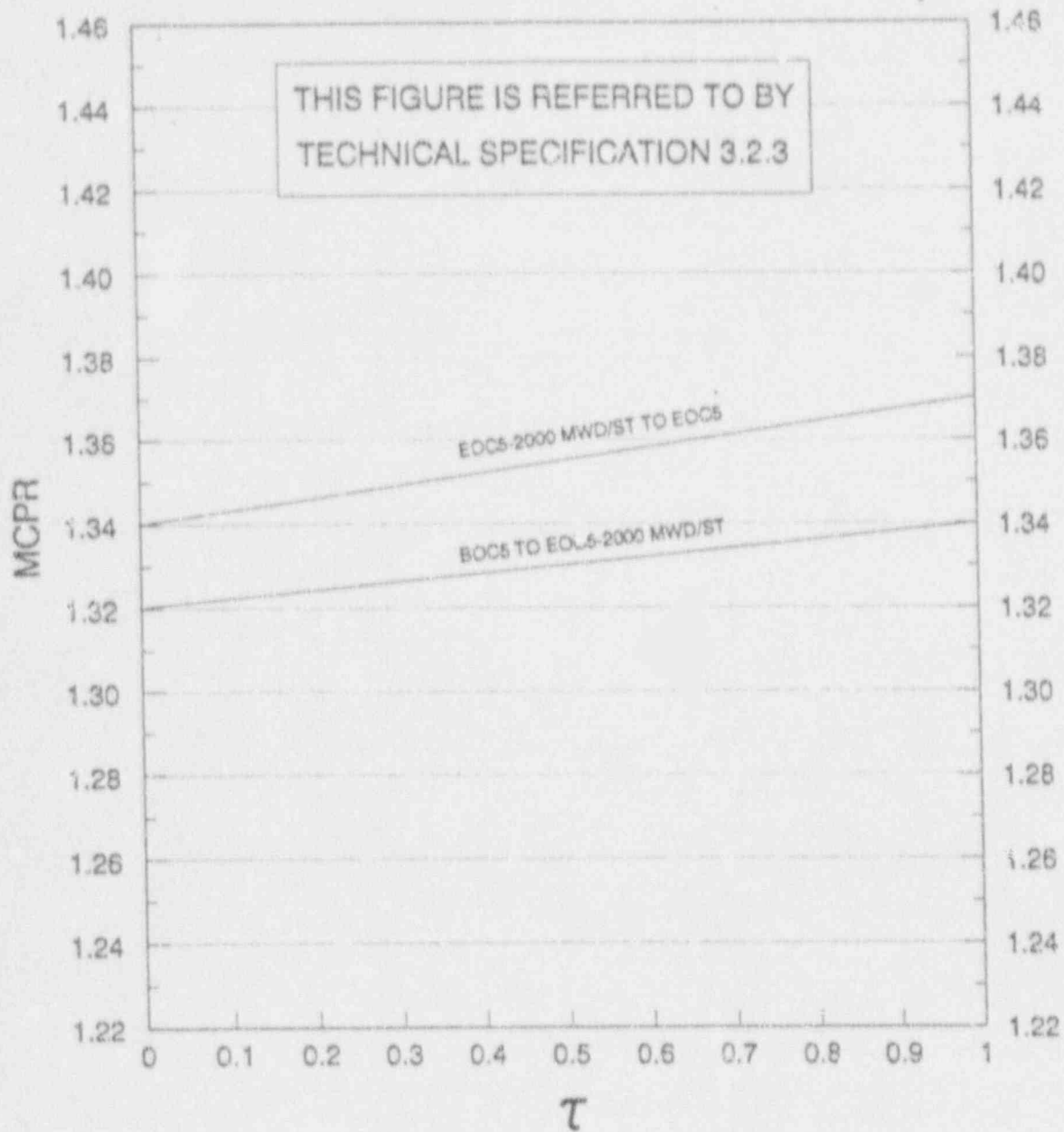
MCPR VS TAU FUEL TYPE GE9B
