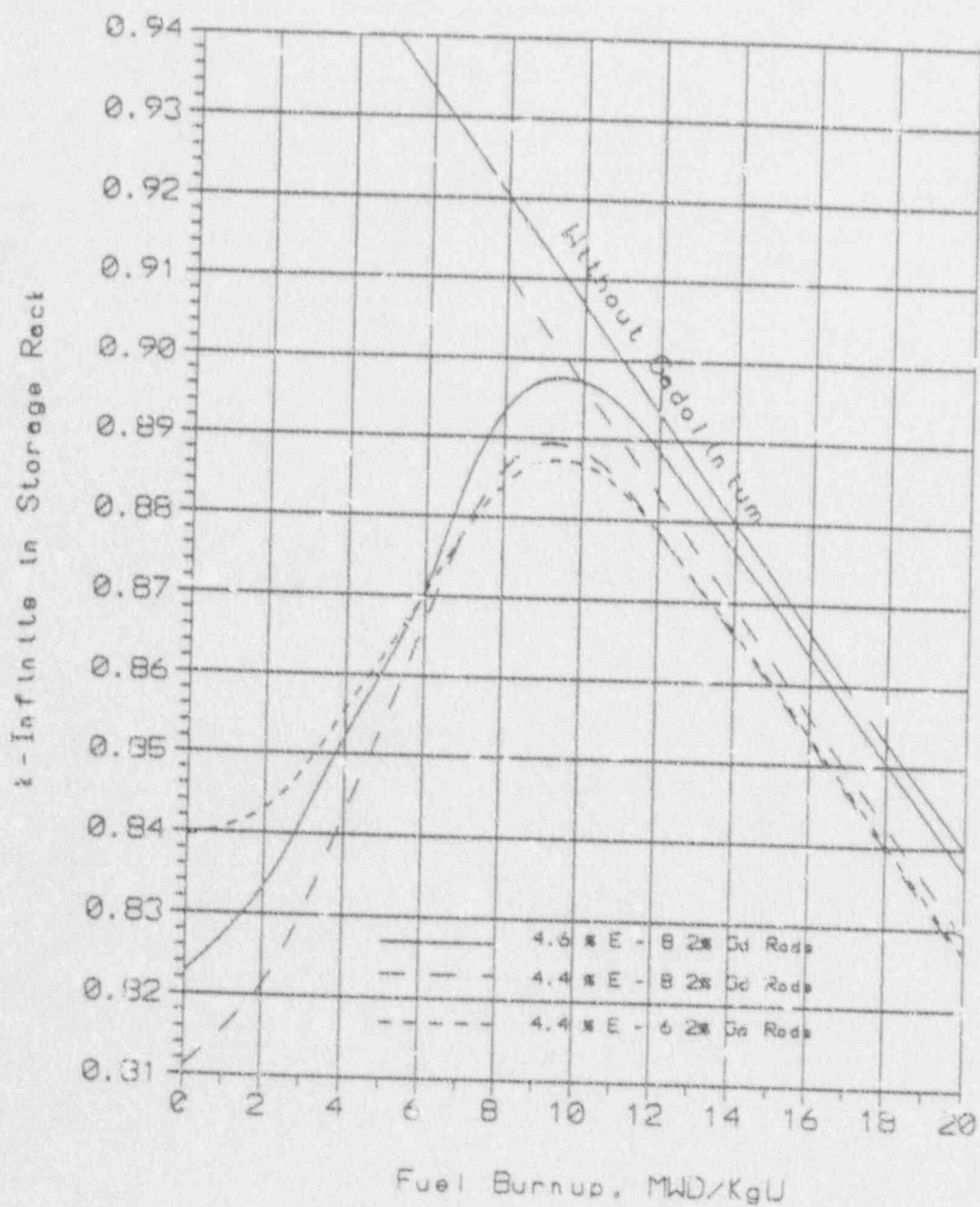
Figure 4.6.1 Reactivities in the Storage React with 4.4% and 4.6% Enriched Fuel
