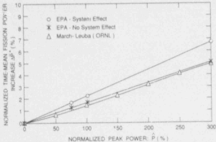
Figure 6. Dependence of Time-Mean Fission Power on Amplitude of Fission Power. Circles: EPA result with dynamic simulation of feedwater flow and temperature and of steam flow. Stars: EPA results, without system effects. Deltas: ORNL result, without system effects.
