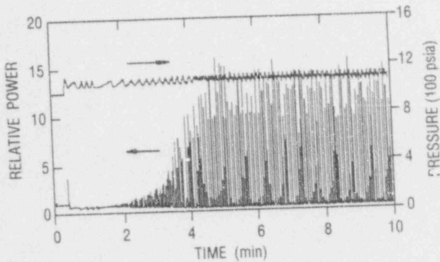
Figure 2. Fission Power and Pressure for ATWS With Simultaneous Turbine and Recirculation Pump Trips, starting from steady-state, no operator interventions (Event Tree Code No. 1, Fig. 5.)
