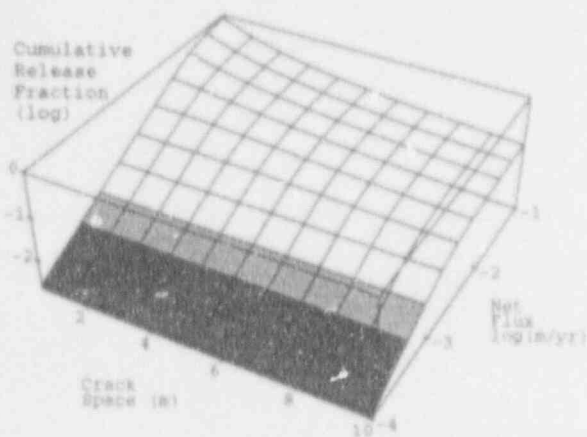
Figure 9. Cumulative release of technetium-99 over 500 years.
