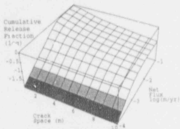
Figure 6. Cumulative release fraction of nitrate over 500 years as a function of crack spacing and water flux through vault.
