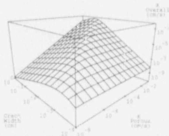
Figure 1. Relationship between crack width, hydraulic conductivity of adjacent porous material, and effective hydraulic conductivity of a vault roof.
