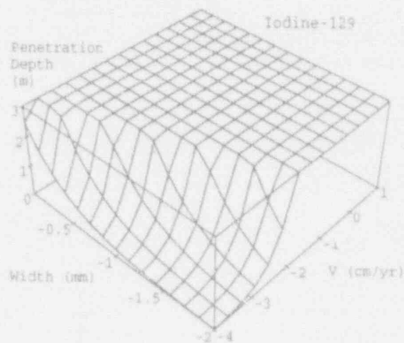
Figure 17. Performance of concrete barriers in attenuating iodine-129 transport.
