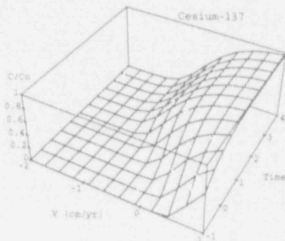
Figure 24. Dimensionless concentration of cesium-137 as a function of Darcy flux through the vault and time.
