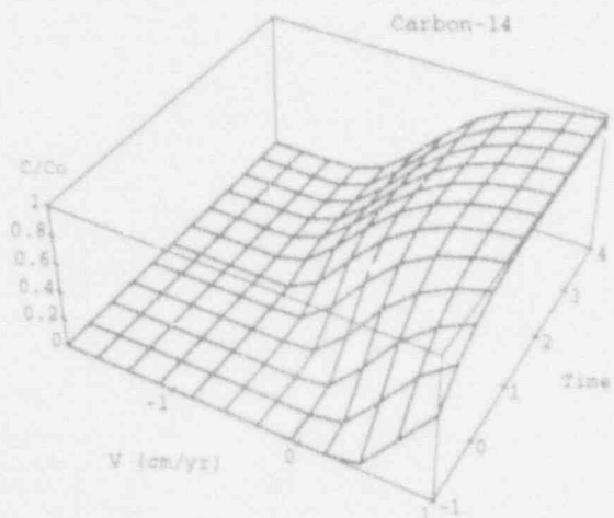
Figure 23. Dimensionless concentration of carbon-14 as a function of Darcy flux through the vault and time.
