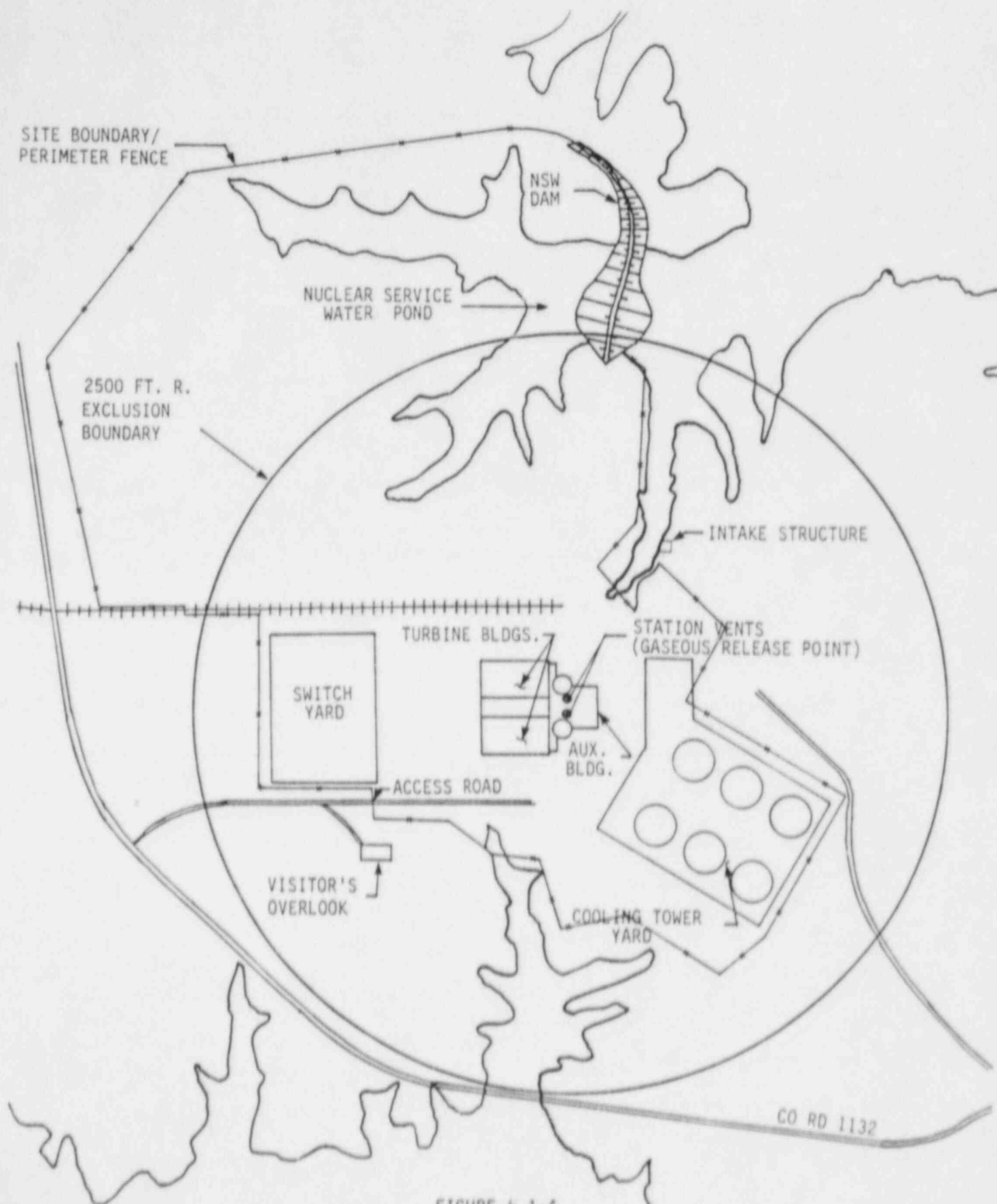
FIGURE 5.1-4 UNRESTRICTED AREA AND SITE BOUNDARY FOR RADIOACTIVE GASEOUS EFFLUENTS CATAWBA - UNIT 1
