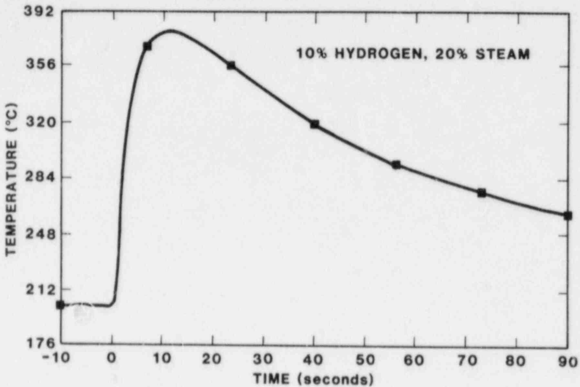
Figure 15. Typical Temperature Response for Flat-Plate Calorimeter
