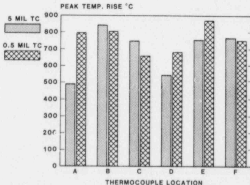
Figure 13. Thermocouple Response Comparison
