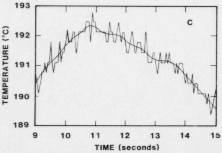
Figure 11. Comparison of Unsmoothed Data and Data after Smoothing with Butterworth Filter
