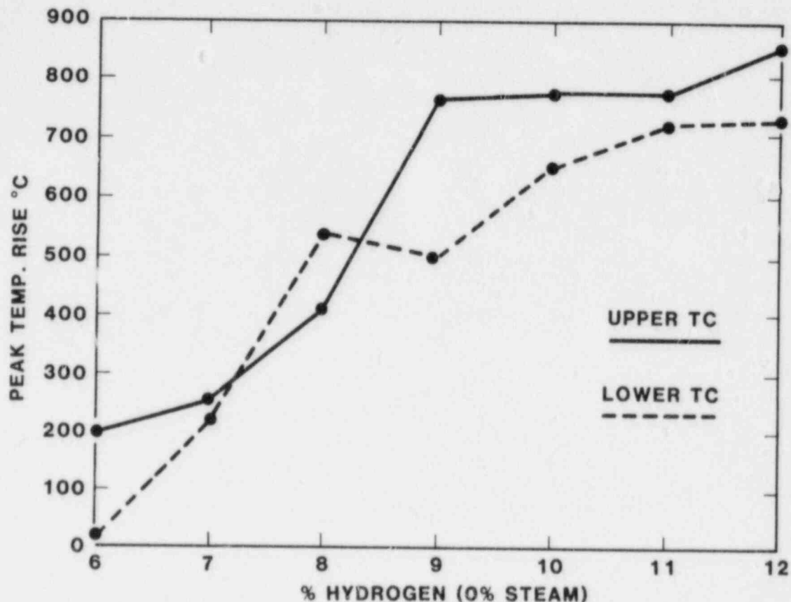
Figure 14. Effect of Hydrogen Concentration on Peak Temperature Rise
