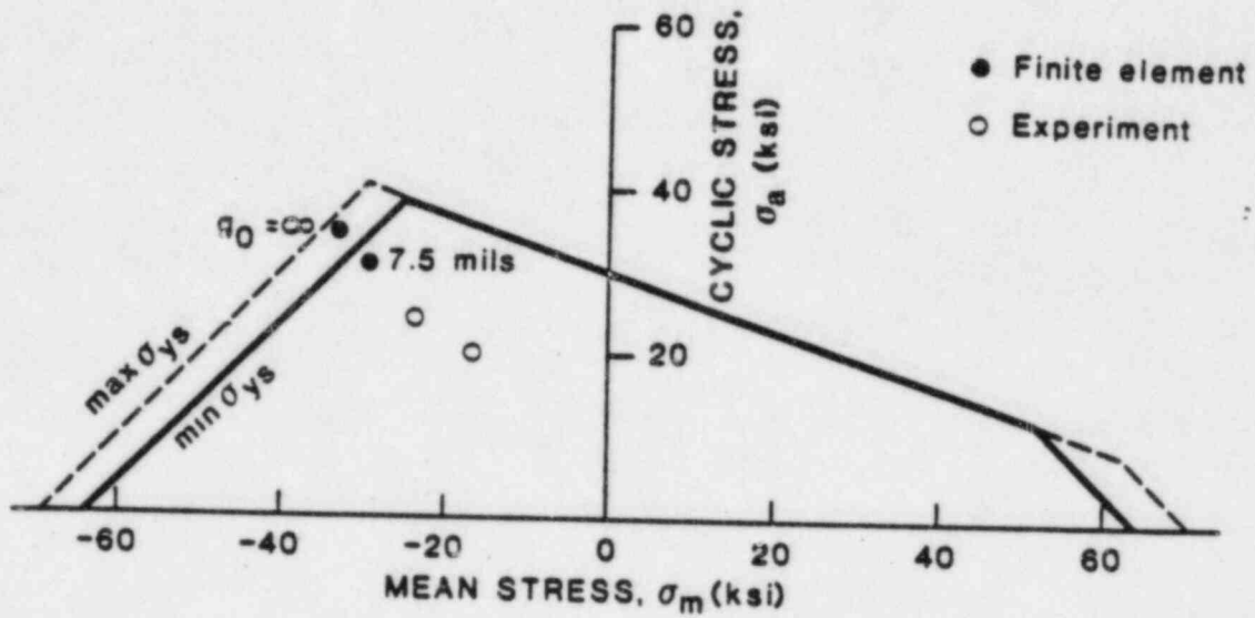
Stress states for isothermeal AE piston skirt for various gap sizes plotted on graph of allowable stress amplitude as a function of mean stress.
