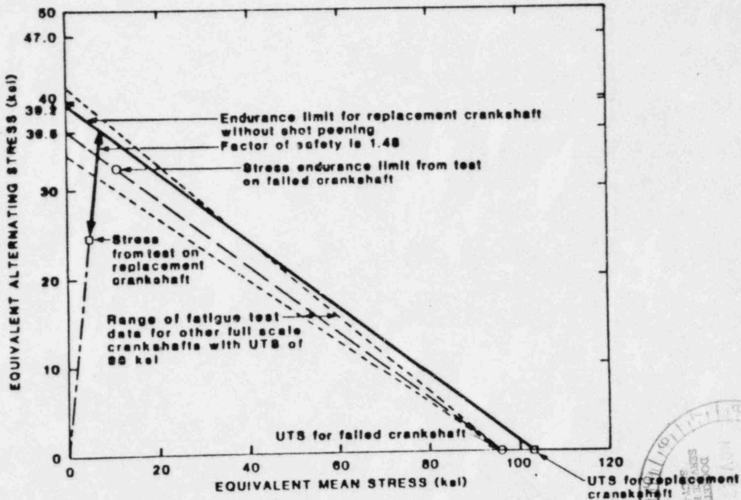
Figure 3-13. Goodman diagram for replacement crankshafts.
