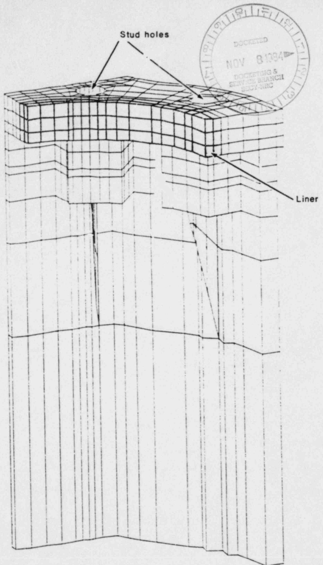
Perspective view of three-dimensional block top model.
