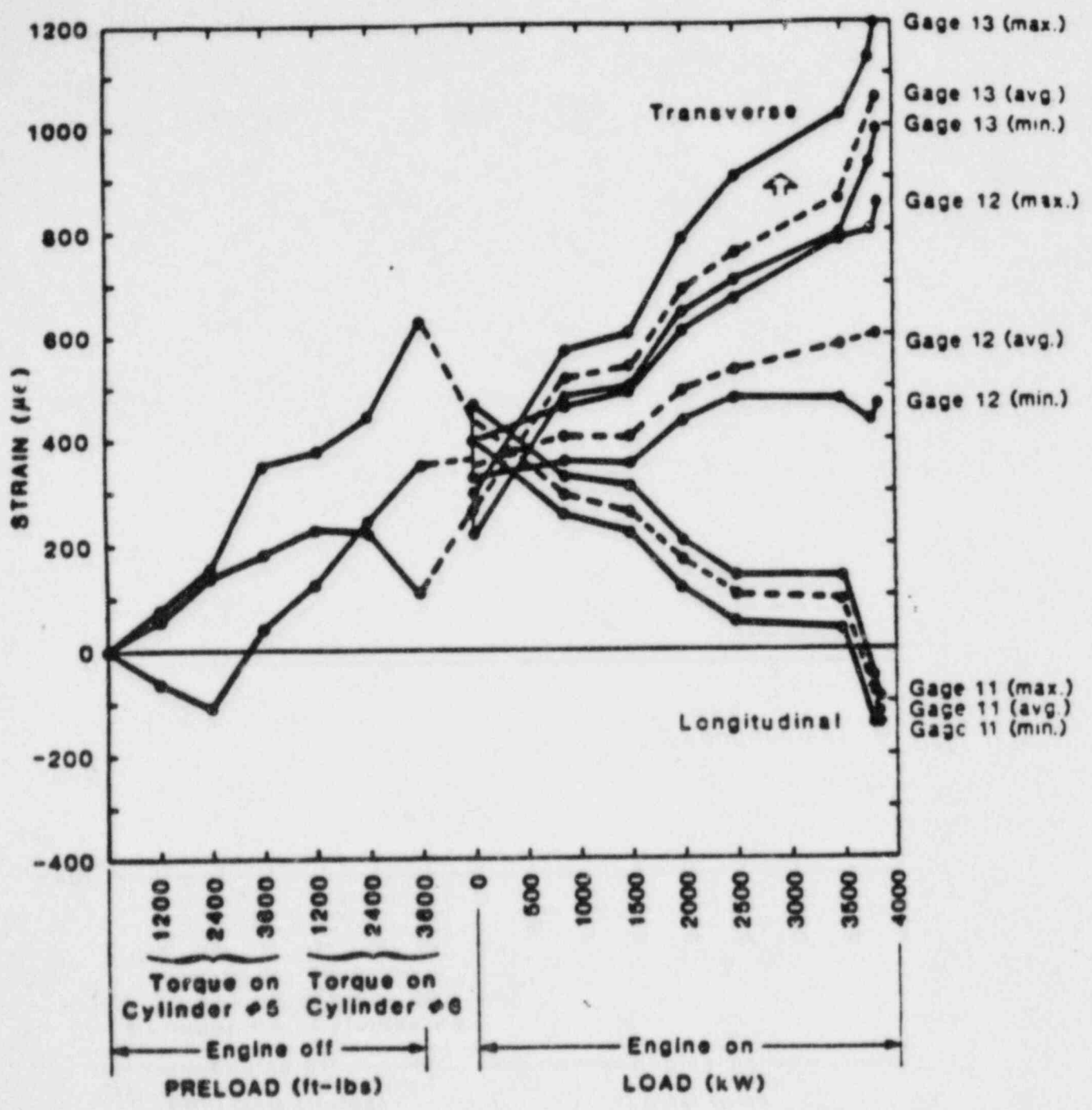
Strain vs. load for Gages 11, 12 and 13 (located between studs).
