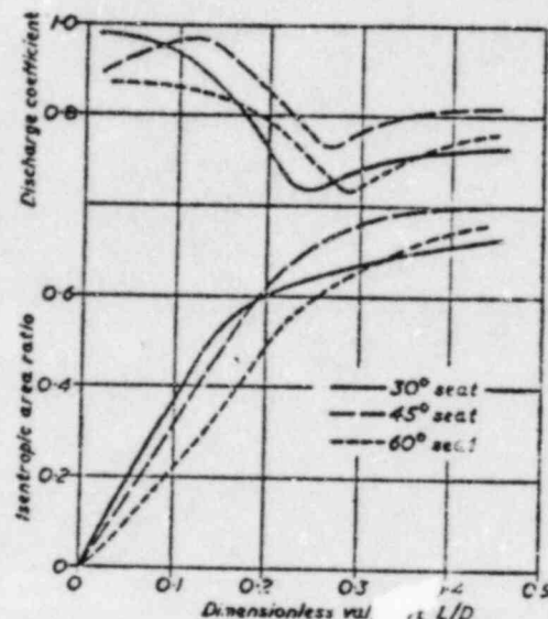
FIG. 8—Flow characteristics of valves with 30-degree, 45-degree and 60-degree seats
