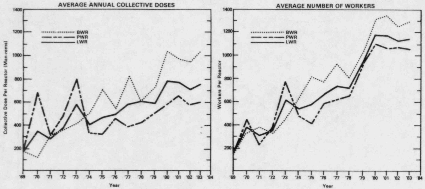
FIGURE 1 COMMERCIAL LIGHT WATER COOLED REACTORS 1969 - 1983
