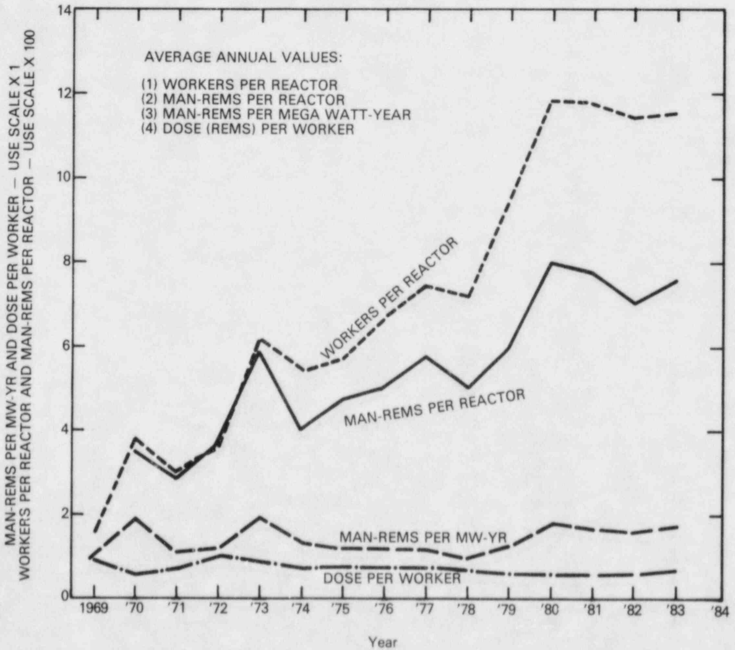
FIGURE 3 AVERAGE ANNUAL VALUES AT LIGHT WATER COOLED REACTORS 1969 - 1983
