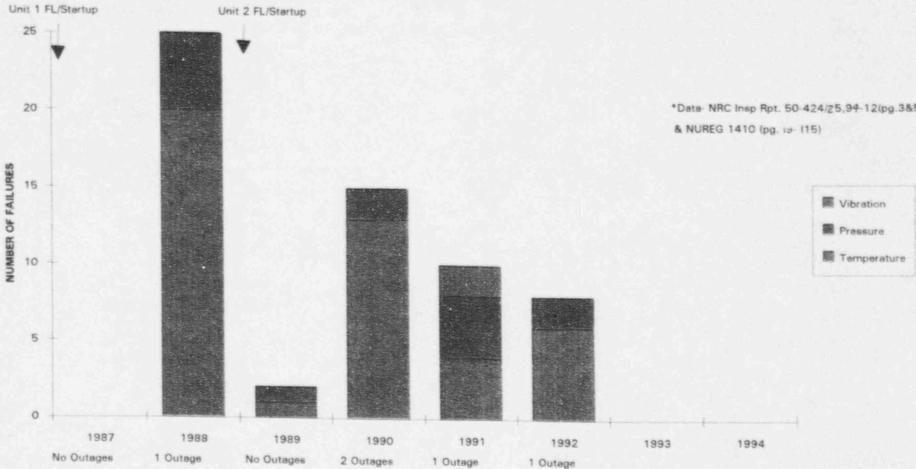
"POST OL" VOGTLE UNITS 1 & 2 CALCON SENSOR FAILURES*
