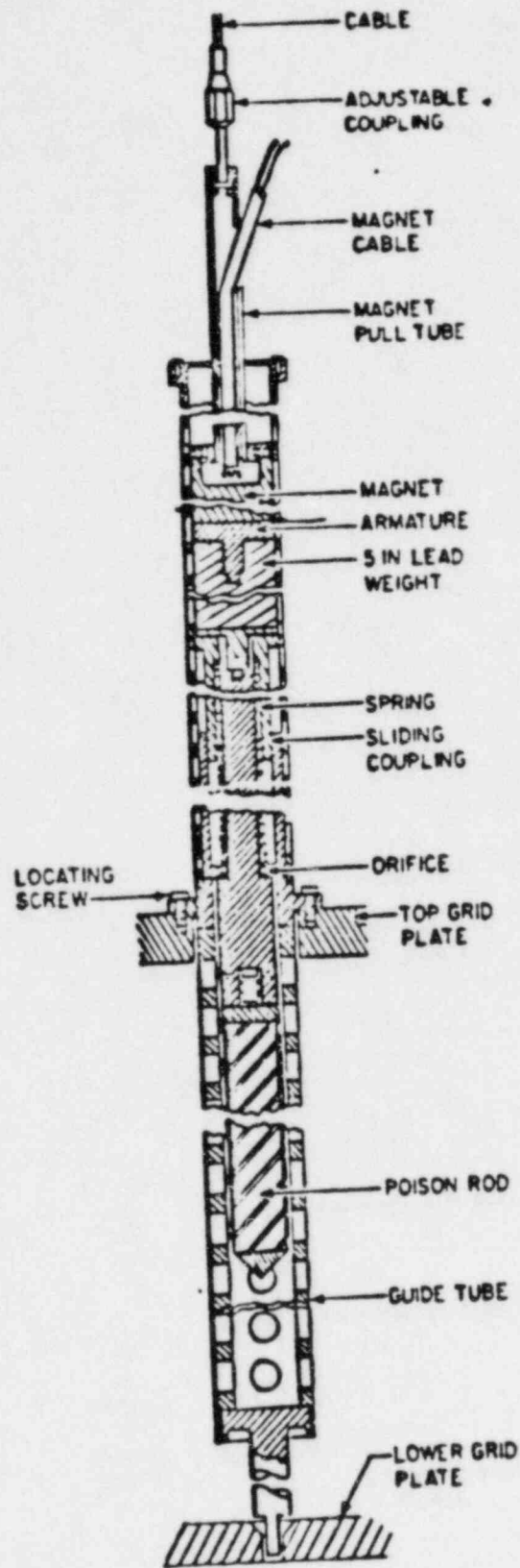
Fig. 7.1. UTR control rod assembly.
