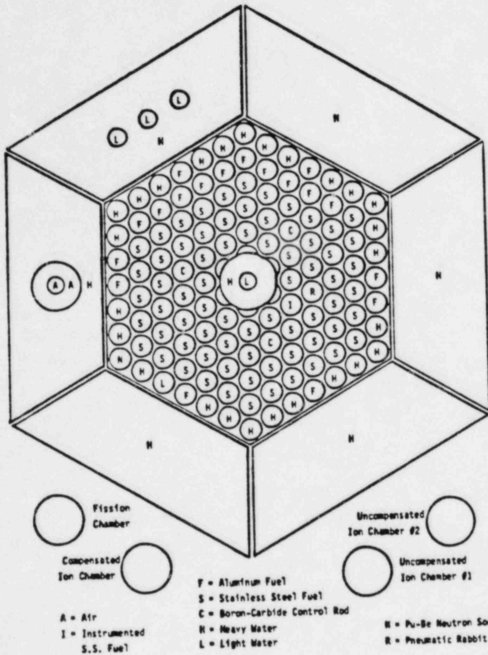
Fig. 4.3. UUTR core configuration.
