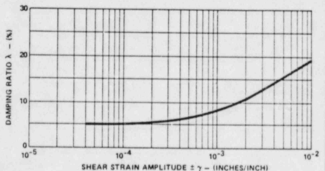
TAKEN FROM SEED, H. BOLTON AND IDRIS I.M. (1969) "THE INFLUENCE OF SOIL CONDITIONS ON GROUND MOTIONS DURING EARTHQUAKES"
