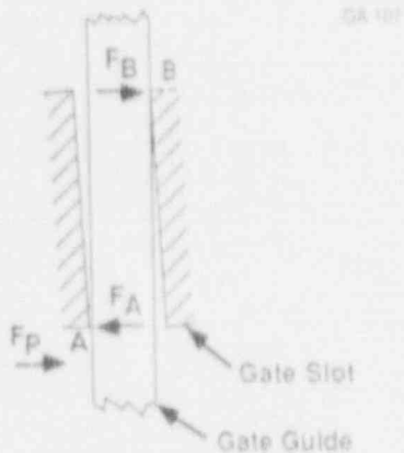
Figure 2.17 Tilted Gate Contacting Guides
