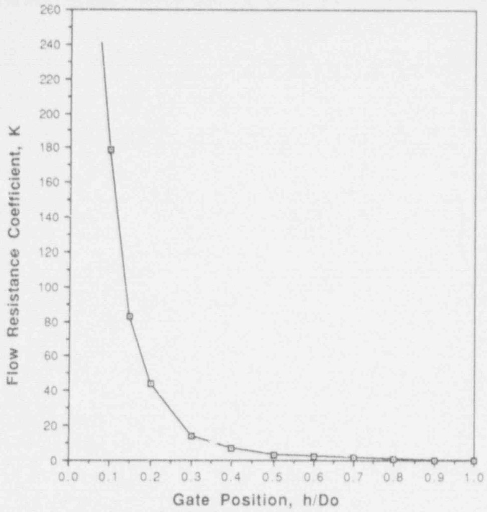
Figure B.1 Average Flow Resistance Coefficient Variation as a Function of Disc Travel for Gate Valves
