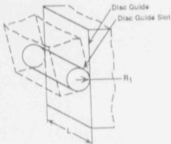
Figure C.3 Math Model for Line Contact between Disc and Guide
