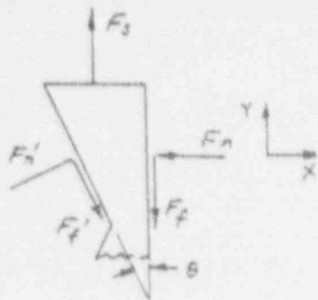
Figure 2.8 Gate Equilibrium Under Unwedging Load During Opening
