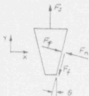
Figure 2.3 Gate Equilibrium Under \Delta P Load During Opening
