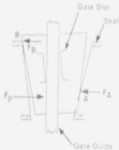
Figure 2.18 Tilted Gate Contacting Seat
