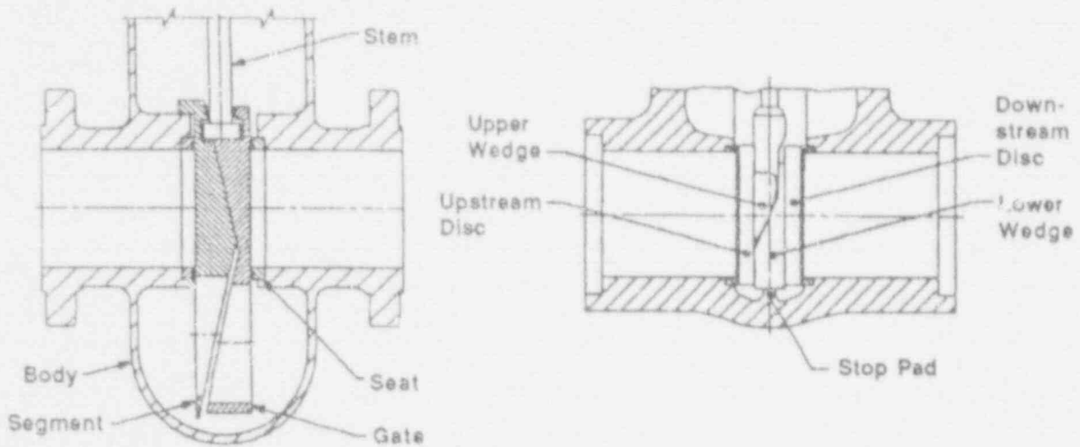
Figure 2.1b Parallel Expanding Gate Valves
