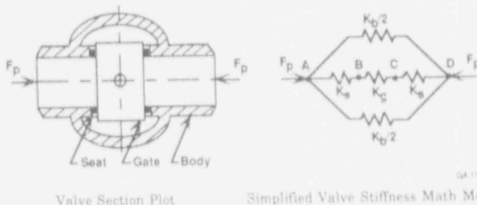
Figure E.1 Simplified Math Model for Gate Valve Stiffness
