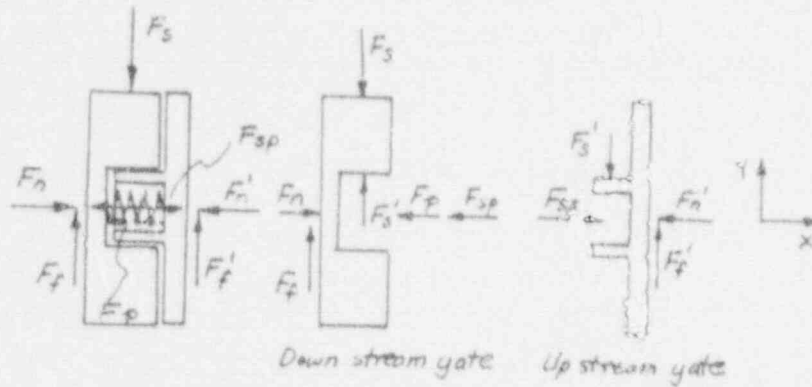
Figure A.8 Gate Equilibrium under \Delta P Load During Closing
