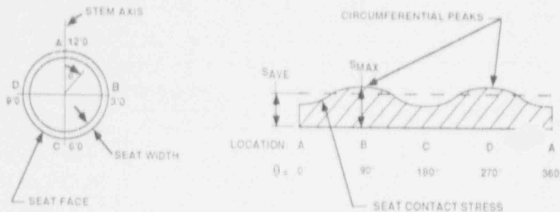
Figure 3.1b Circumferential Seat Contact Stress Variation
