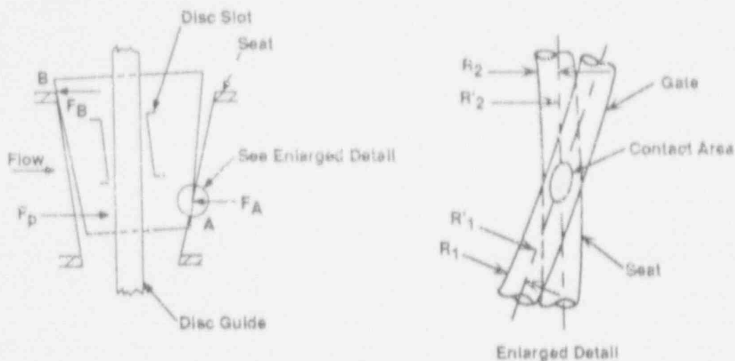
Figure C.2 Tilted Disc Contacting Seat
