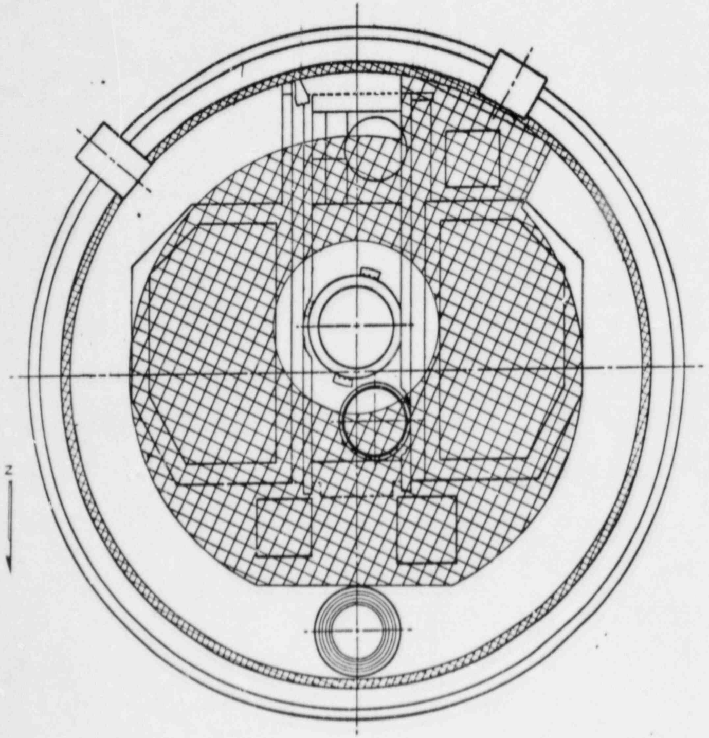
FIGURE 25 CONTAINMENT ARRANGEMENT
