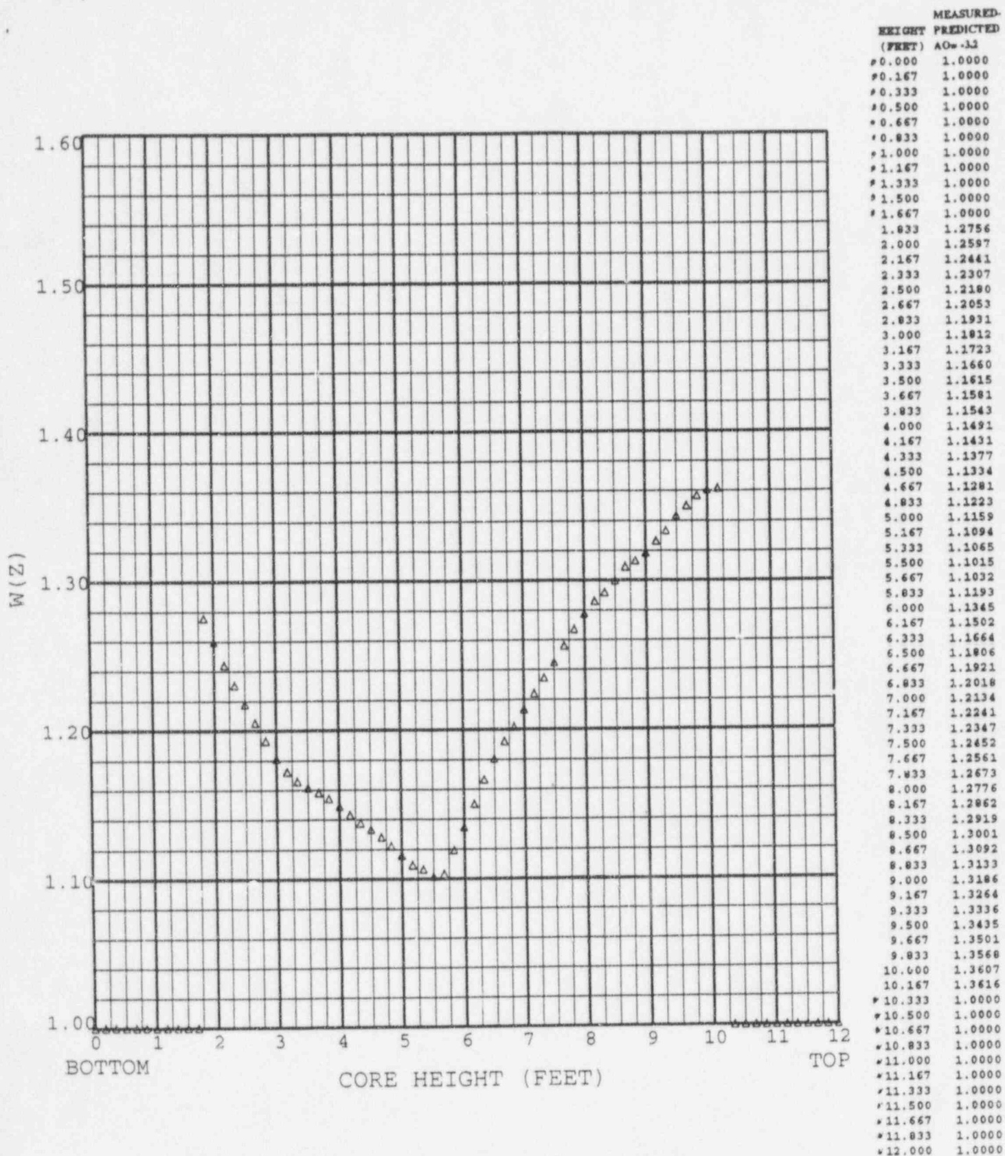
Figure 11 Callaway Unit 1 Cycle 8 W(z)_{no} at 10000 MWD/MTU
