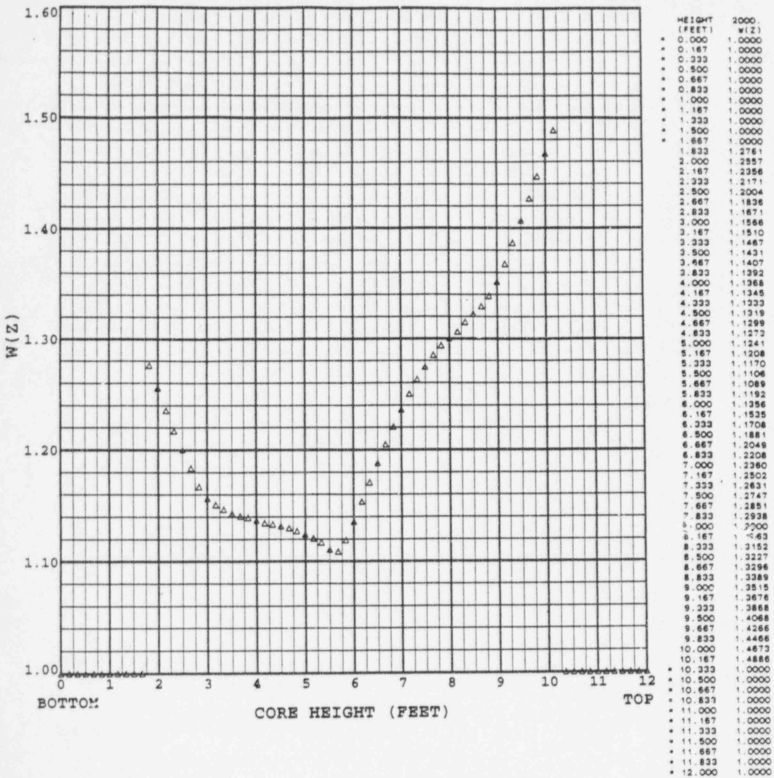
Figure 6 Callaway Unit 1 Cycle 8 W(z)no at 2000 MWD/MTU
