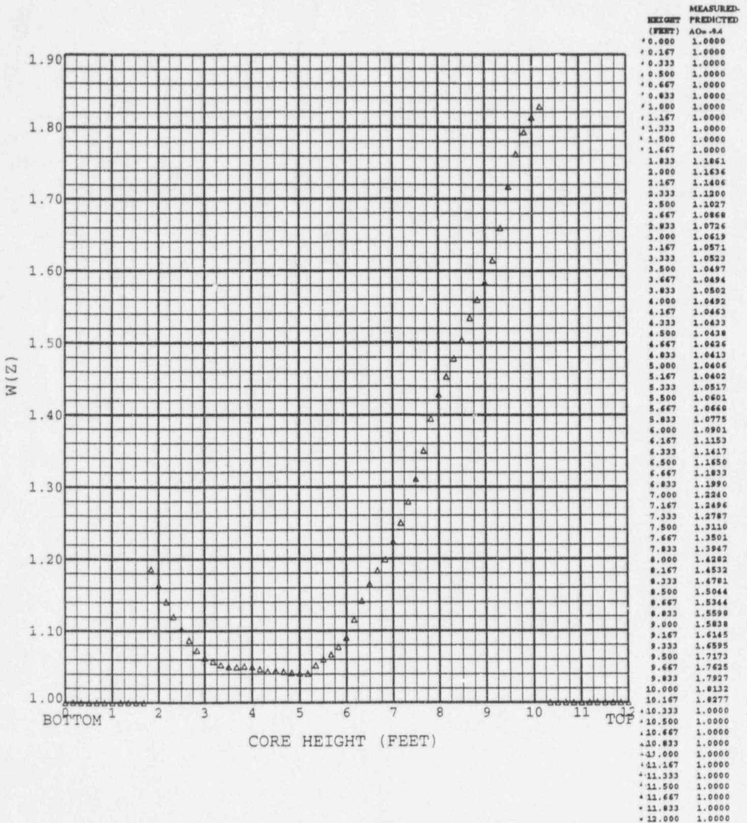
Figure 16 Callaway Unit 1 Cycle 8 W(z)_{no} at 2000 MWD/MTU
