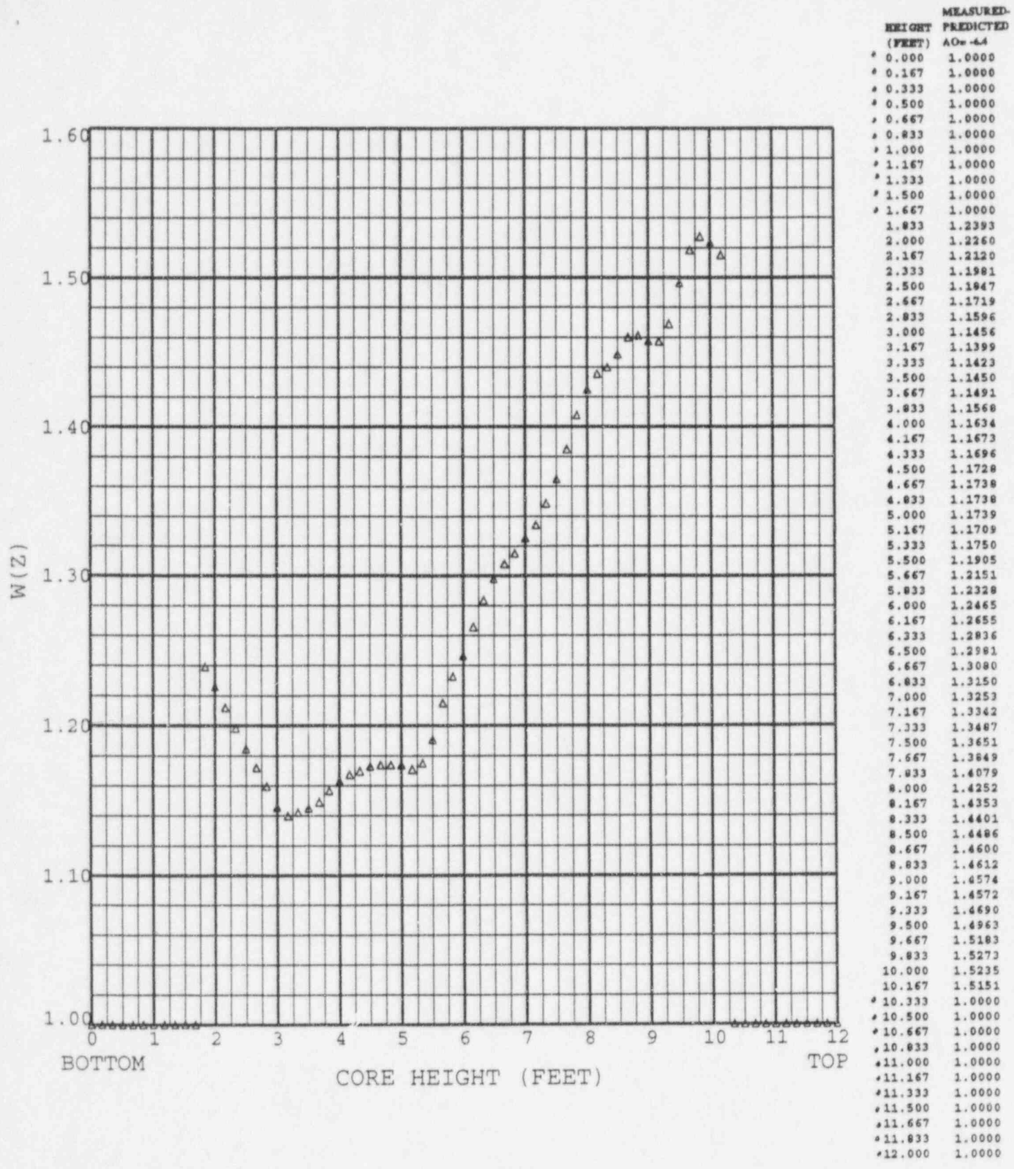
Figure 15 Callaway Unit 1 Cycle 8 W(z) DC at 18000 MWD/MTU
