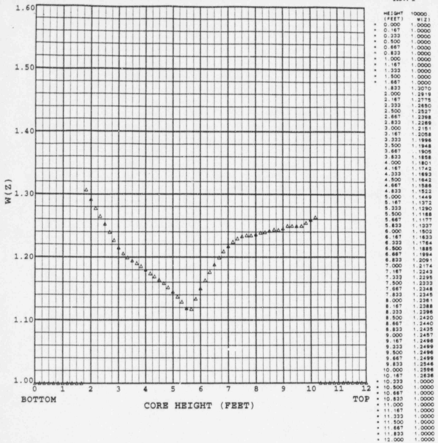
Figure 7 Callaway Unit 1 Cycle 8 W(z)no at 10000 MWD/MTU
