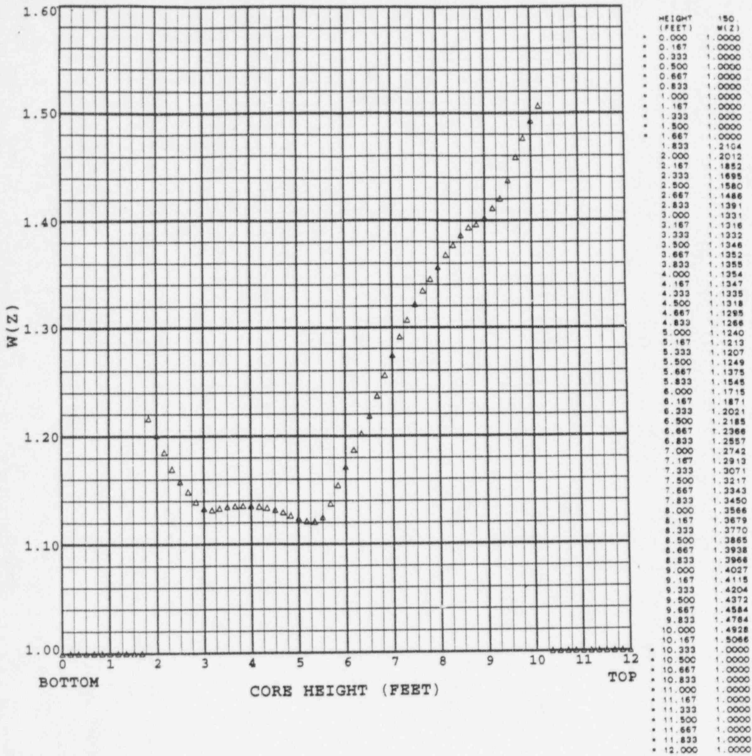
Figure 5 Callaway Unit 1 Cycle 8 W(z)no at 150 MWD/MTU
