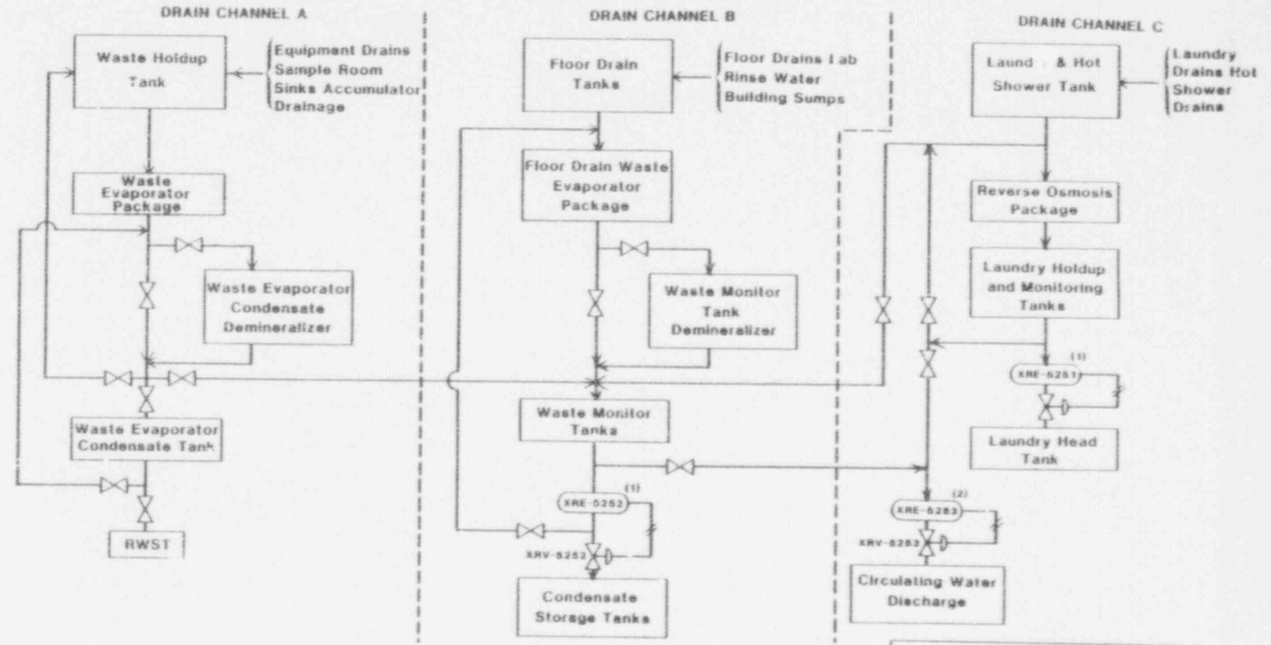
FIGURE 1.1 (page 2 of 2) LIQUID EFFLUENT DISCHARGE PATHWAYS NOTES: (1) Spared in place (2) Discharge valve closes on monitor Hi-rad, loss of flow, or channel out-of-service alarms.
