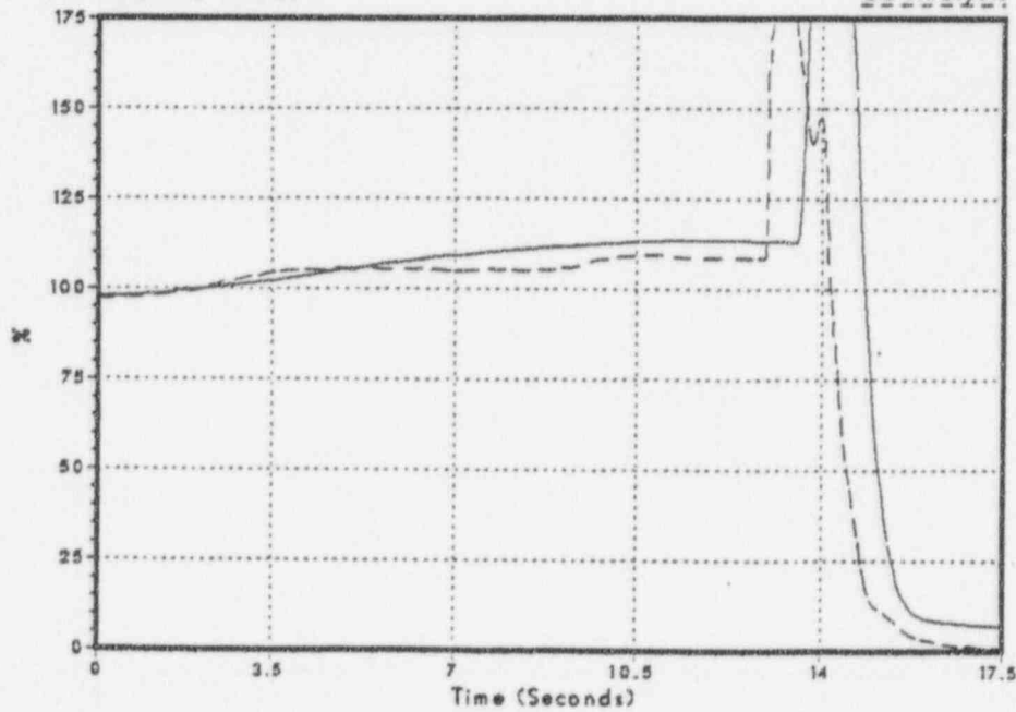
Figure 3.2-100 Relative Power
