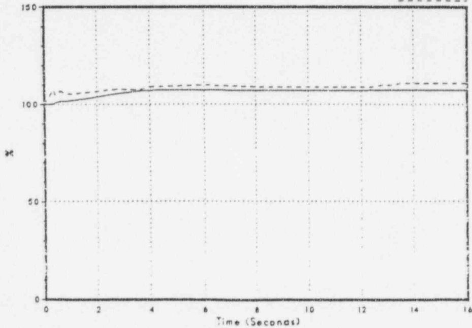
Figure 3.2-4 Core Inlet Flow
