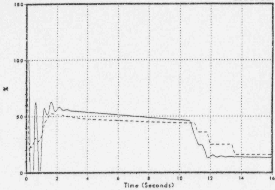
Figure 3.2-12 Main Steam Line Flow
