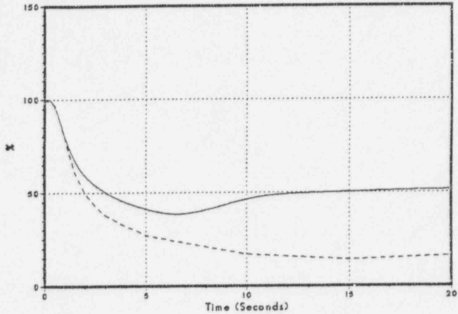
Figure 3.2-68 Relative Power
