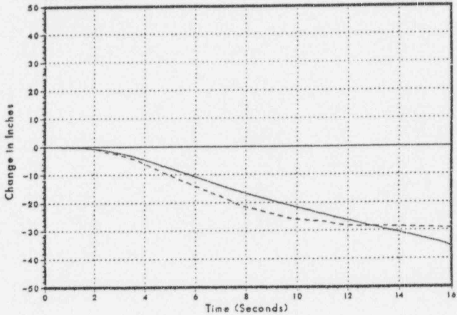
Figure 3.2-36 Sensed Level
