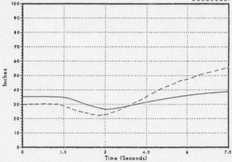
Figure 3.2-112 Sensed Reactor Water Level
