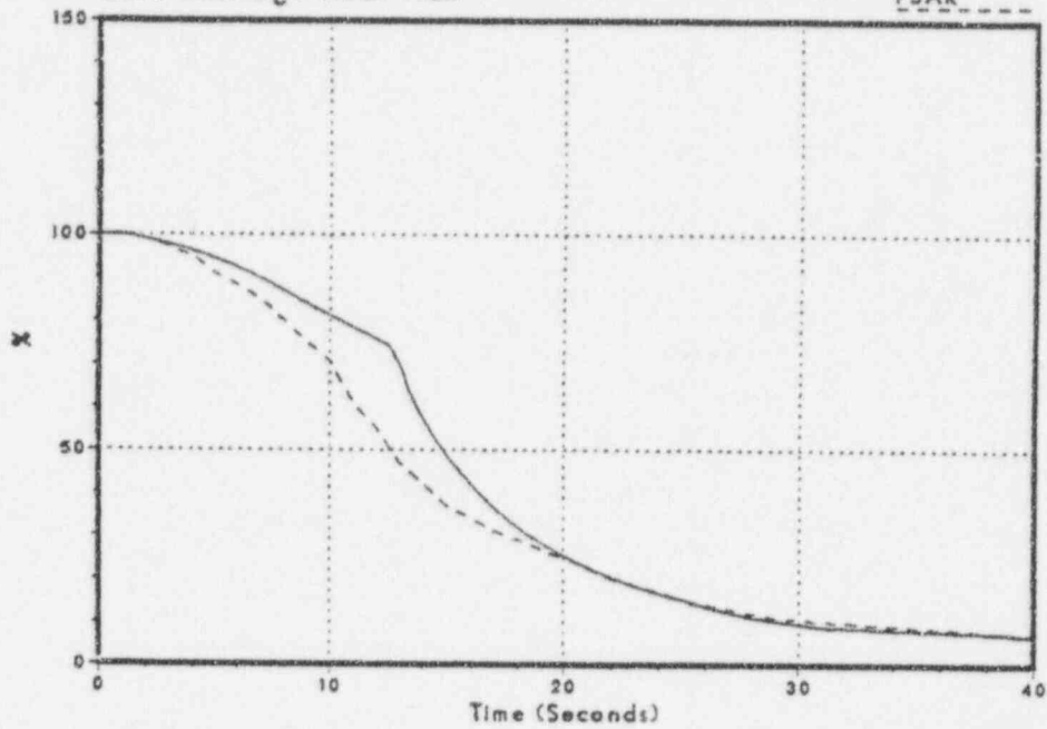
Figure 3.2-52 Core Average Heat Flux
