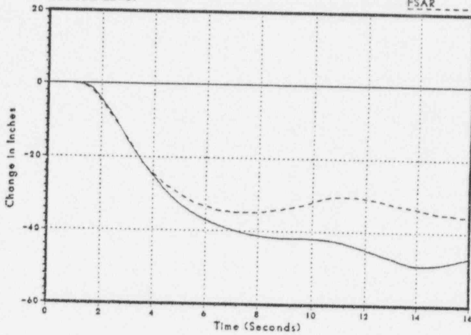
Figure 3.2-28 Sensed Level
