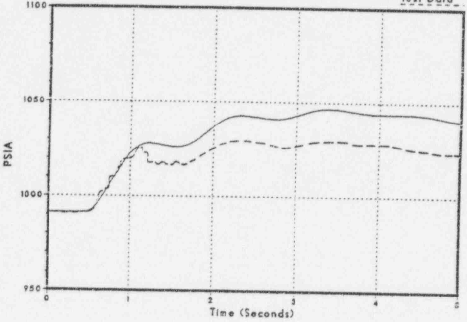
Figure 3.2-113 Steam Dome Pressure
