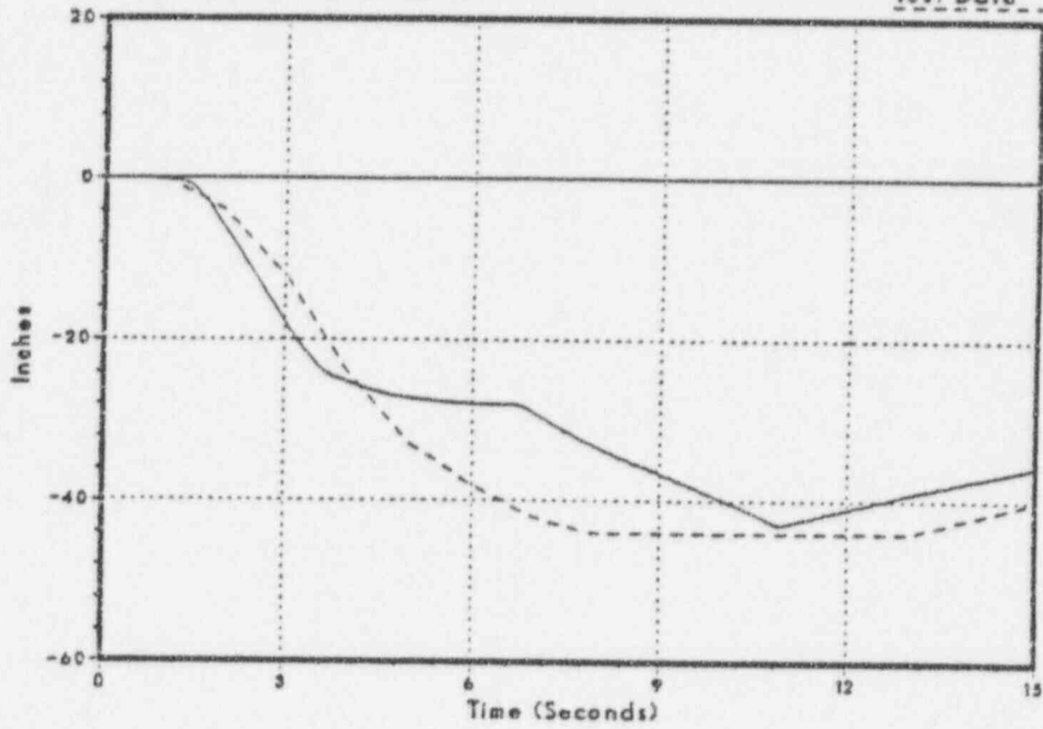
Figure 3.2-130 Steam Dome Water Level
