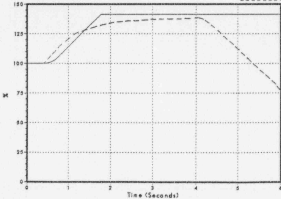
Figure 3.2-97 Feedwater Flow
