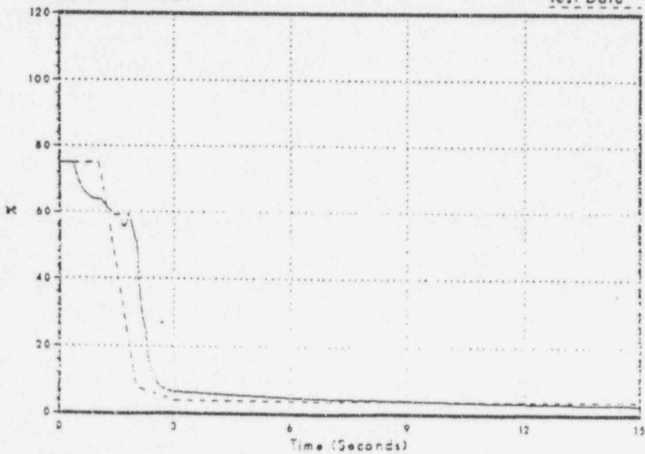
Figure 3.2-129 Relative Power
