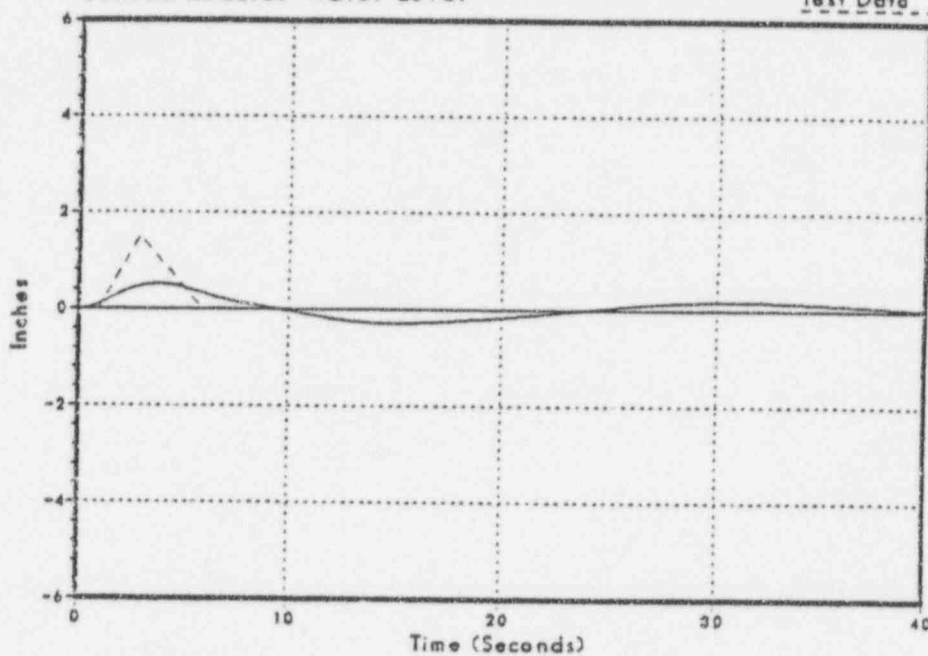
Figure 3.2-145 Sensed Reactor Water Level
