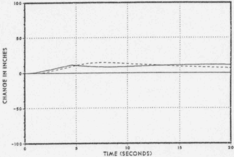
Figure 3.2-64 Sensed Level
