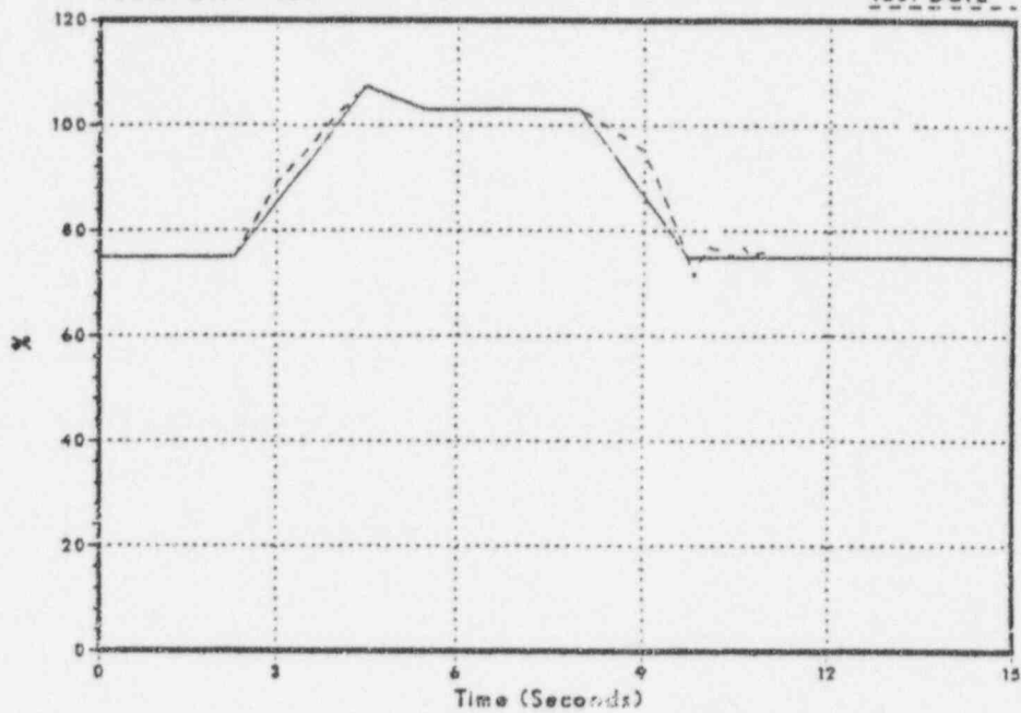
Figure 3.2-132 Feedwater Flow
