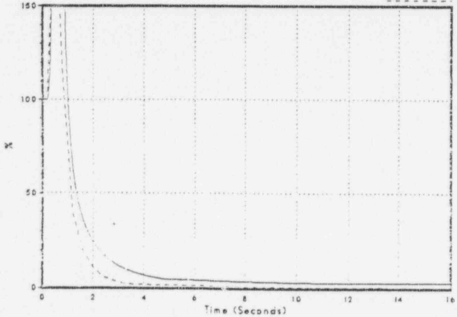
Figure 3.2-9 Relative Power
