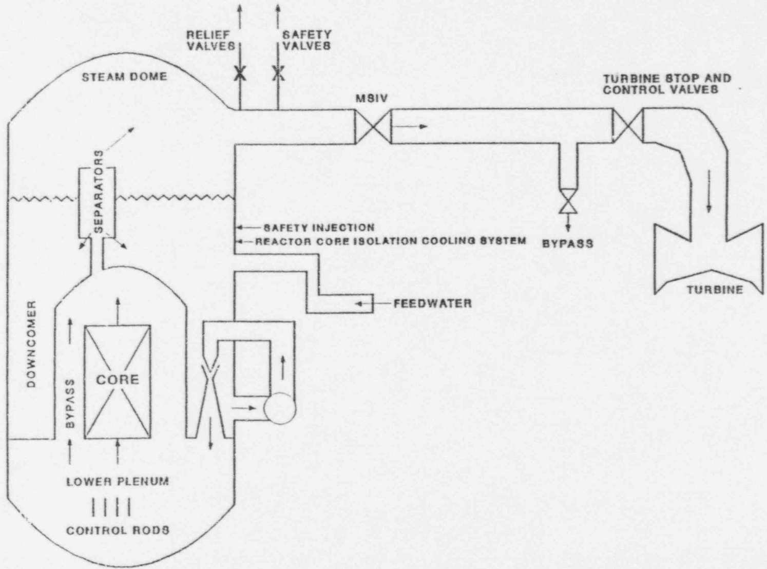
Figure 2.1-1 Schematic of BWR NSSS Representation
