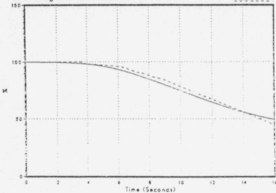
Figure 3.2-39 Average Surface Heat Flux
