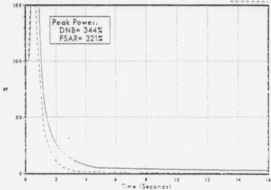
Figure 3.2-2 Relative Power
