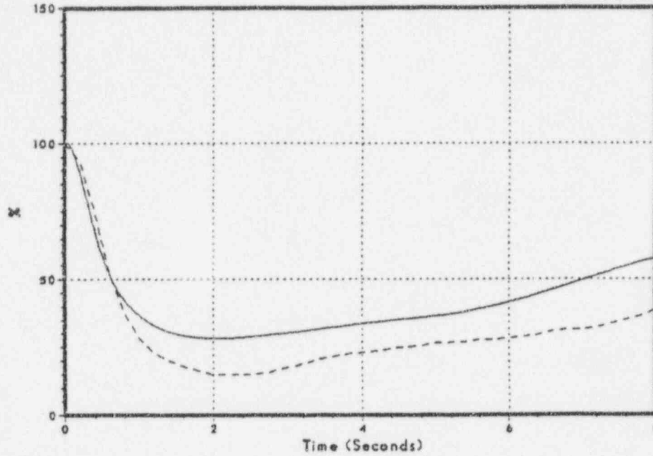
Figure 3.2-61 Relative Power
