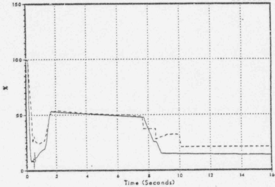
Figure 3.2-21 Vessel Steam Flow
