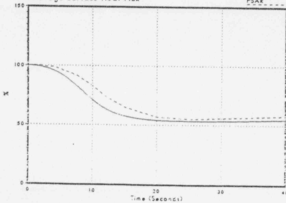
Figure 3.2-81 Average Surface Heat Flux
