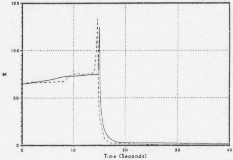
Figure 3.2-33 Relative Power
