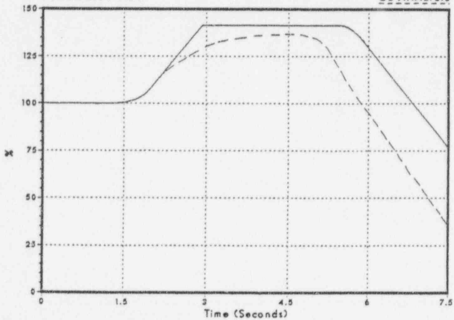
Figure 3.2-111 Feedwater Flow
