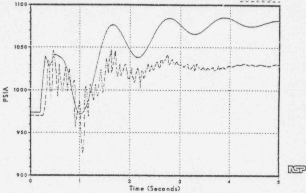
Figure 3.2-121 Turbine Throttle Pressure
