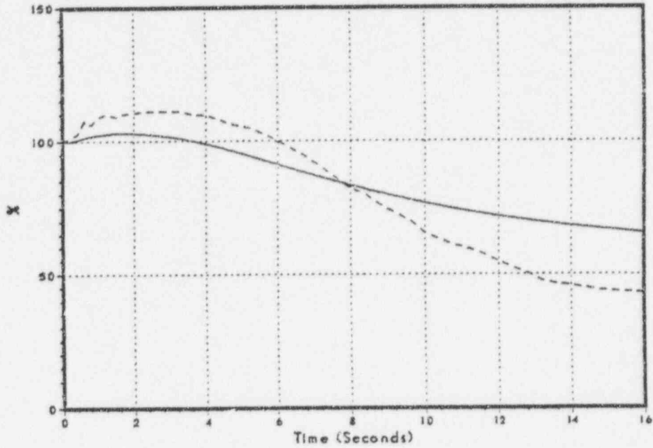
Figure 3.2-17 Core Inlet Flow
