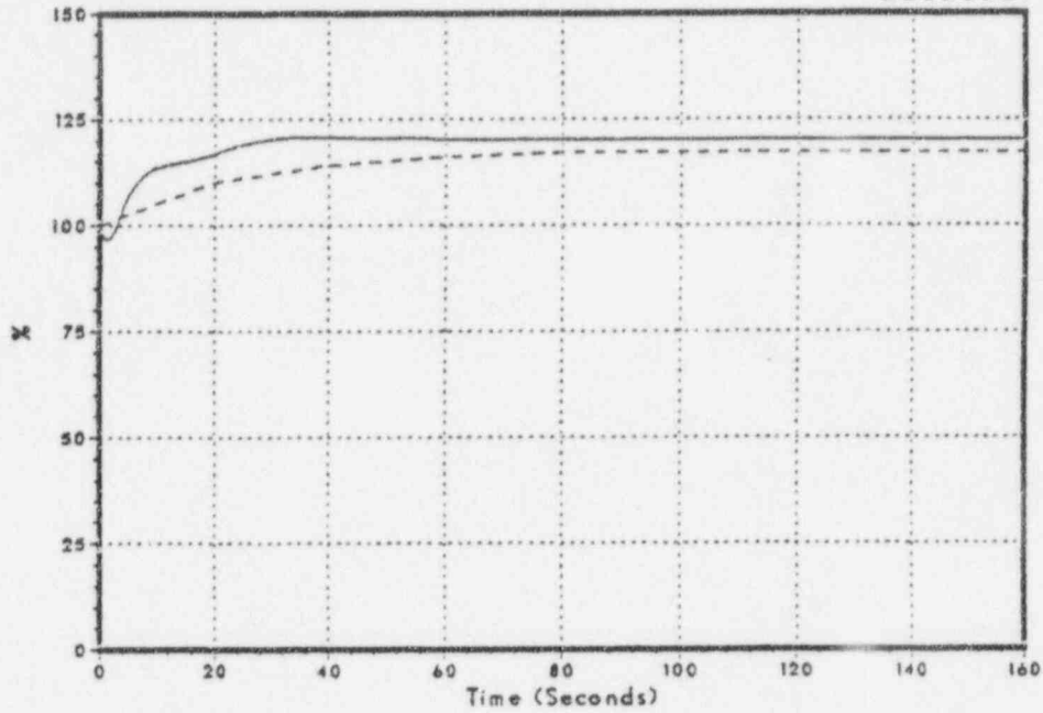
Figure 3.2-47 Relative Power
