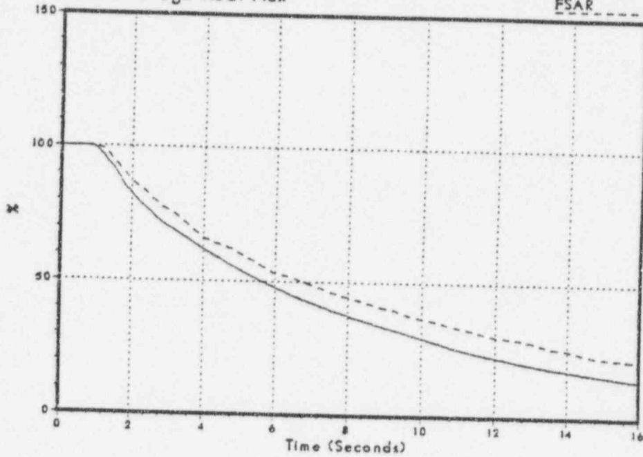
Figure 3.2-24 Core Average Heat Flux
