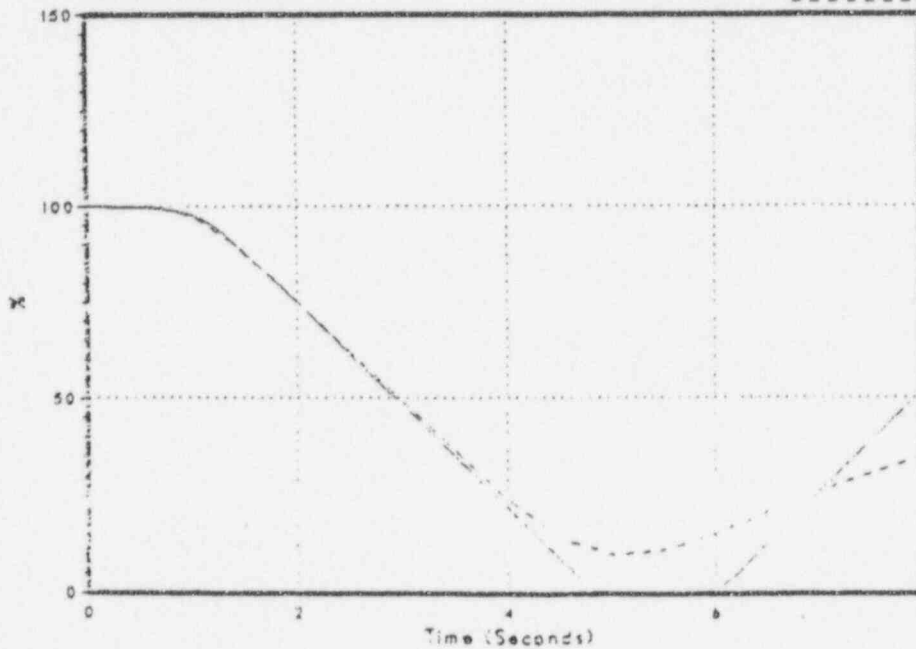
Figure 3.2-62 Feedwater Flow
