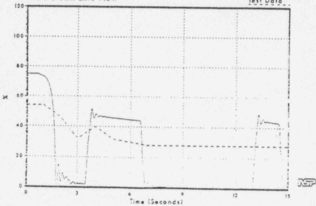
Figure 3.2-131 Main Steam Line Flow
