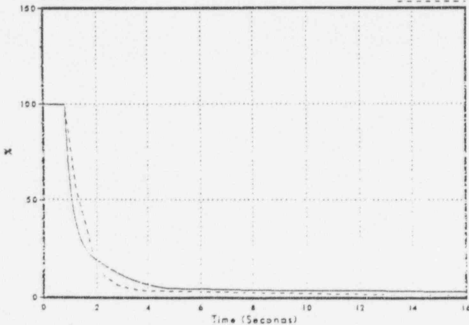
Figure 3.2-23 Relative Power
