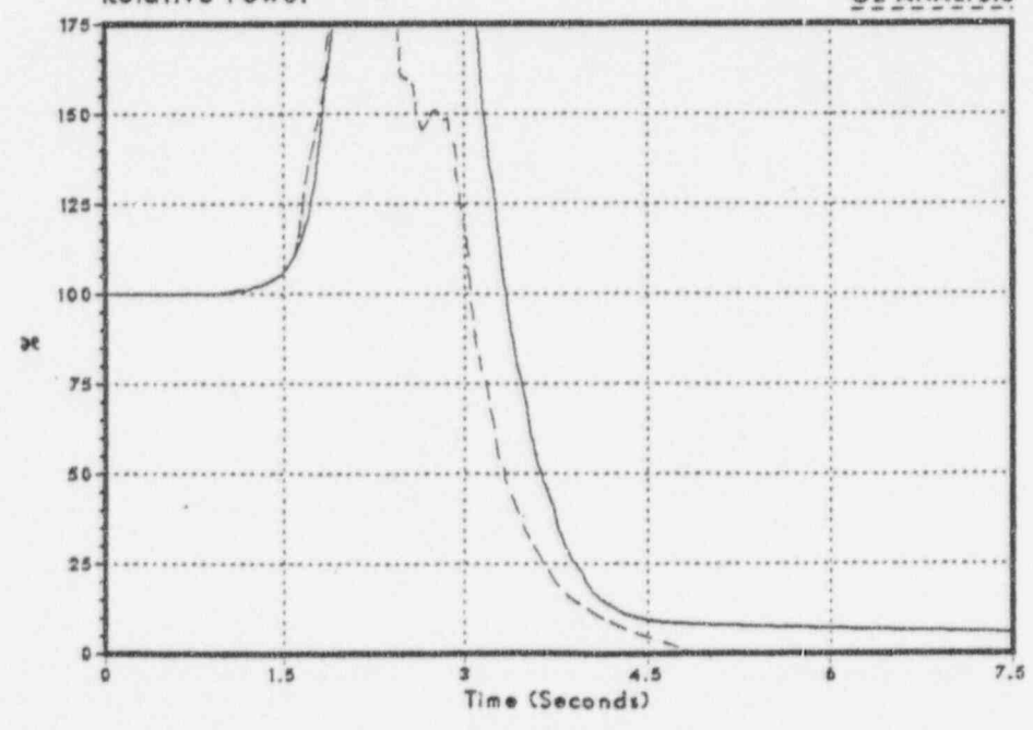
Figure 3.2-107 Relative Power
