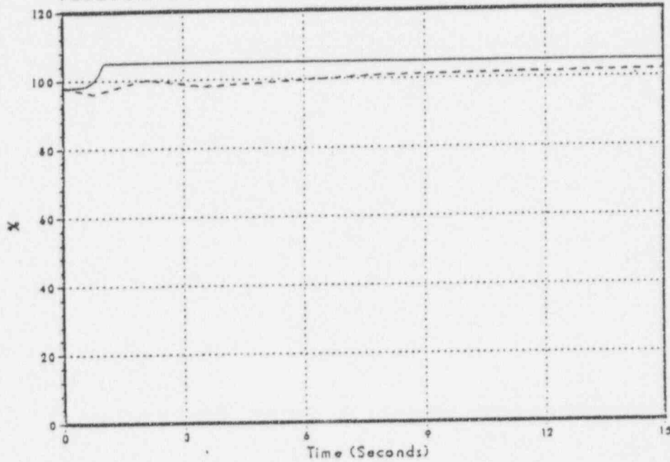
Figure 3.2-126 Feedwater Flow
