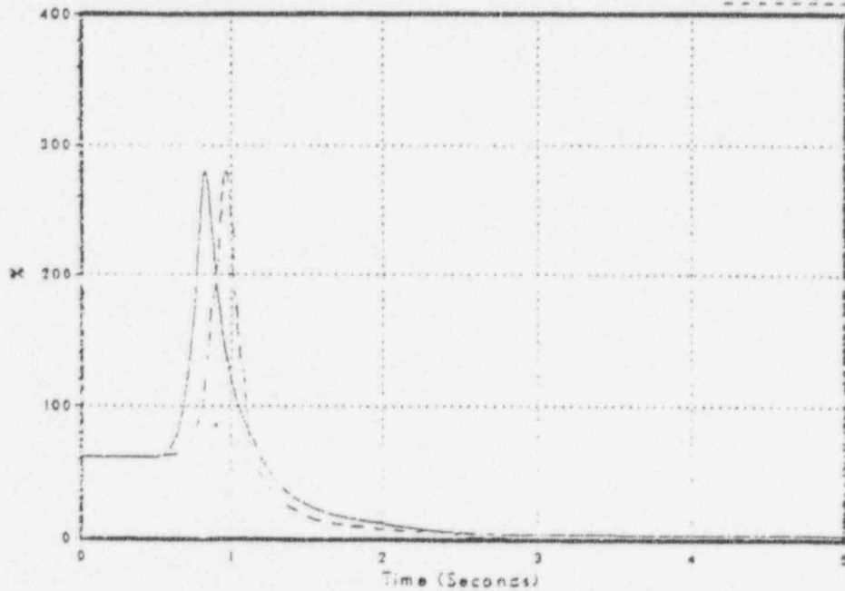
Figure 3.2-117 Relative Power
