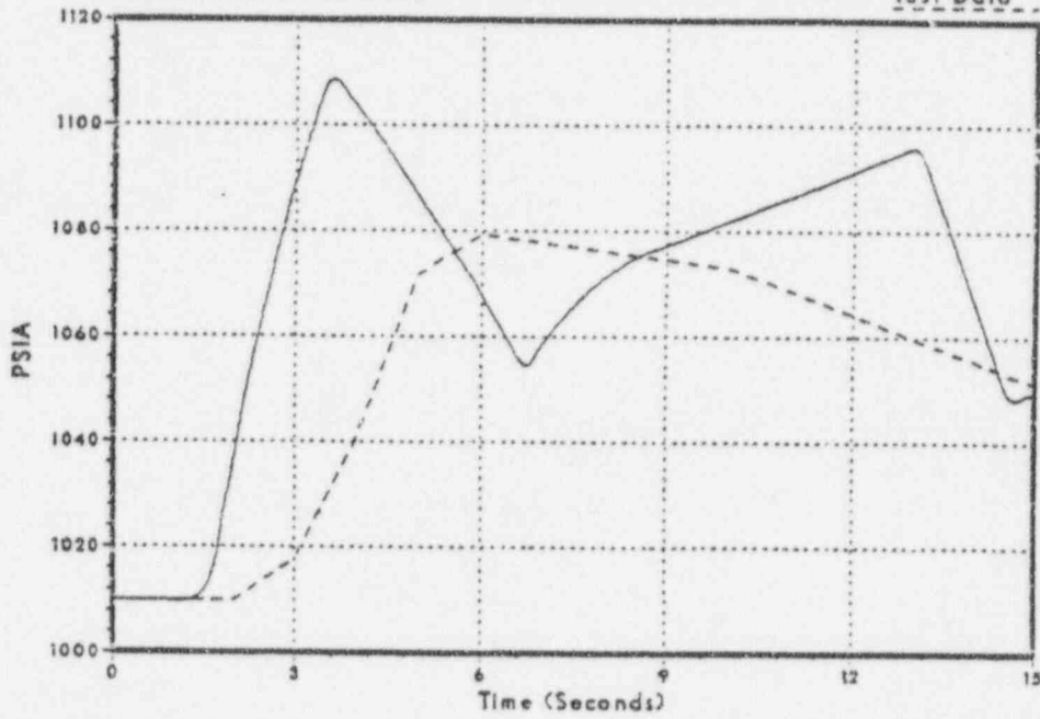
Figure 3.2-128 Steam Dome Pressure
