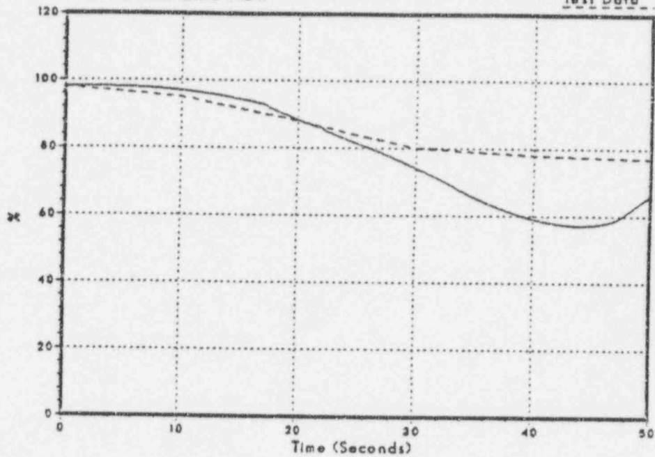
Figure 3.2-137 Main Steam Line Flow
