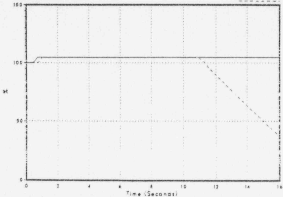
Figure 3.2-20 Feedwater Flow
