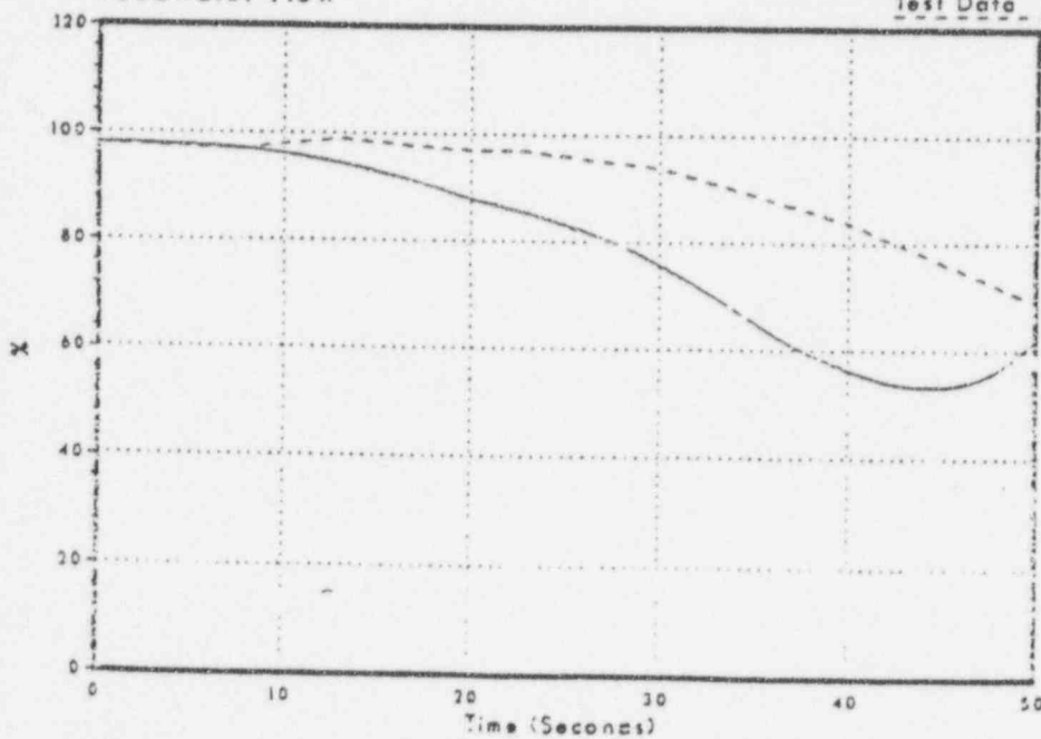
Figure 3.2-138 Feedwater Flow
