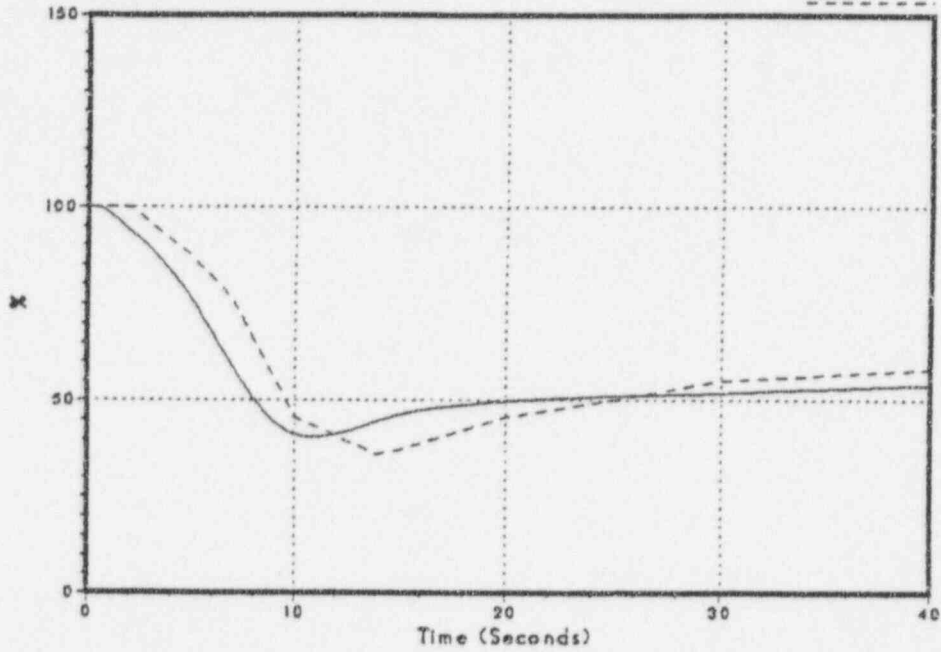
Figure 3.2-82 Relative Power
