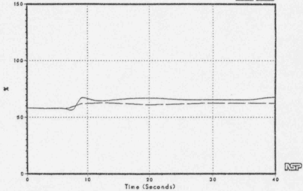
Figure 3.2-91 Vessel Steam Flow
