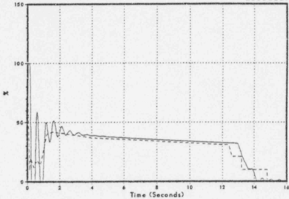
Figure 3.2-5 Main Steam Line Flow
