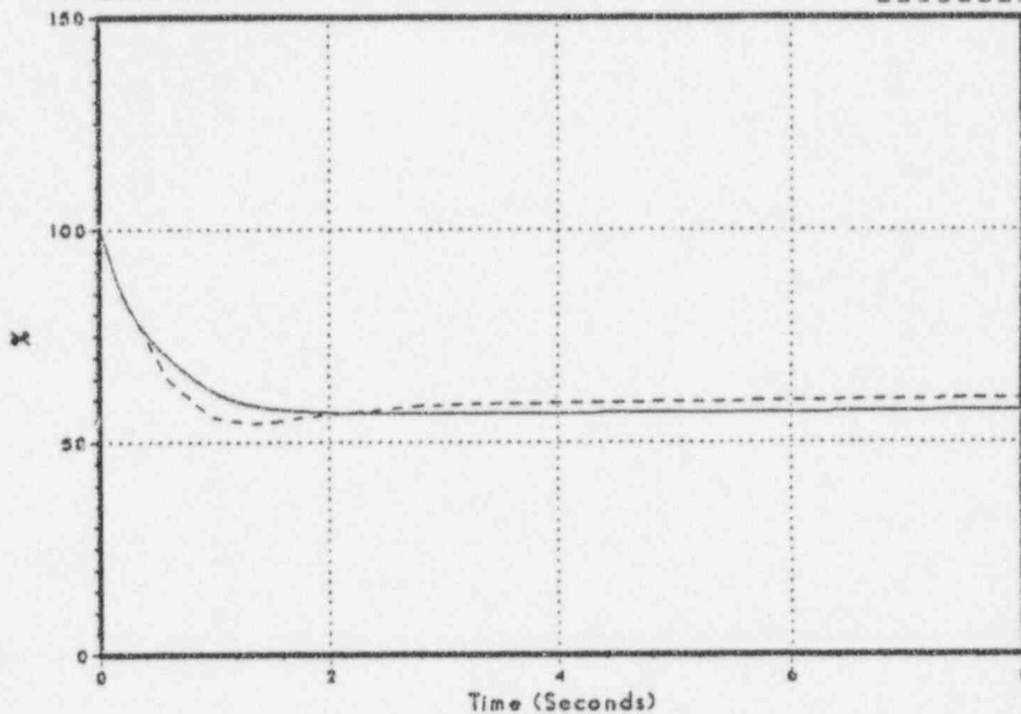
Figure 3.2-59 Core Inlet Flow
