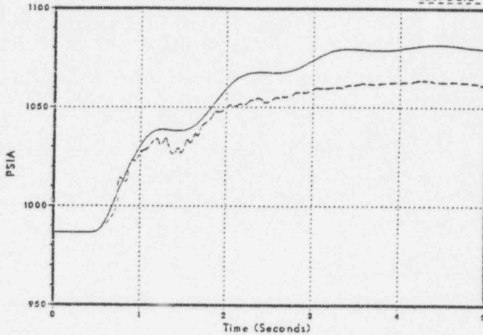
Figure 3.2-119 Steam Dome Pressure
