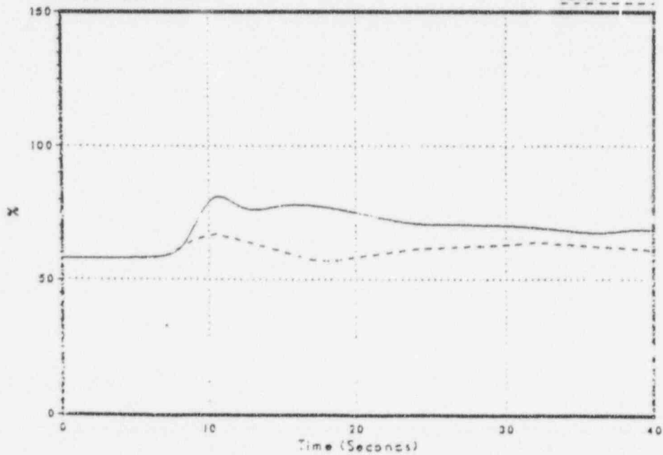
Figure 3.2-90 Feedwater Flow
