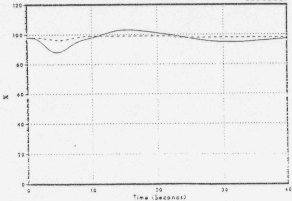
Figure 3.2-144 Feedwater Flow
