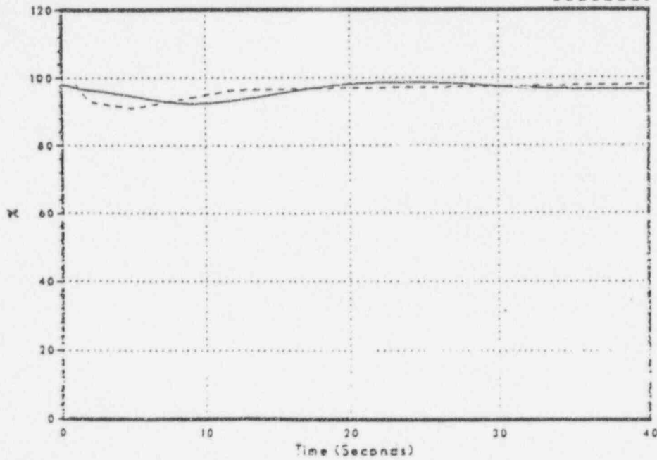
Figure 3.2-142 Relative Power
