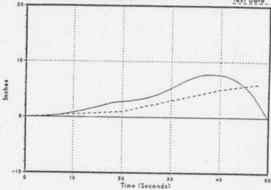
Figure 3.2-139 Sensed Reactor Water Level
