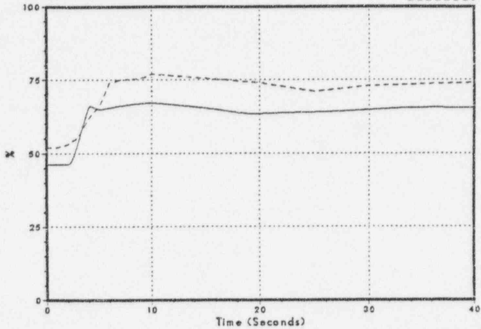
Figure 3.2-73 Core Inlet Flow
