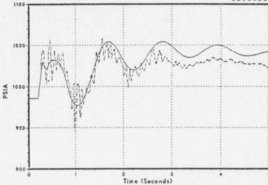
Figure 3.2-115 Turbine Throttle Pressure
