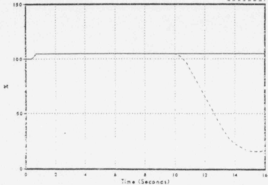
Figure 3.2-13 Feedwater Flow
