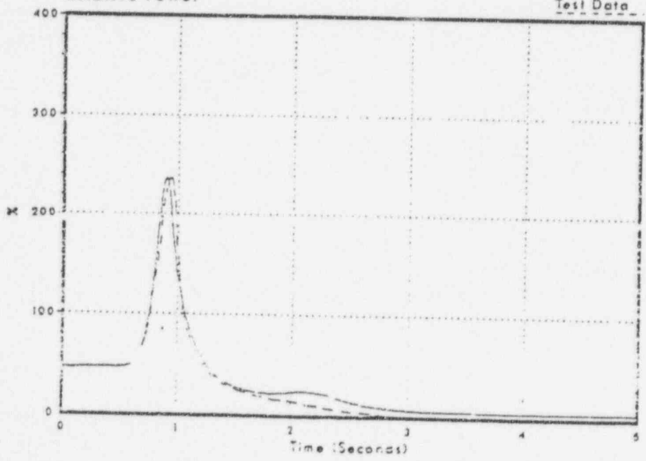
Figure 3.2-114 Relative Power
