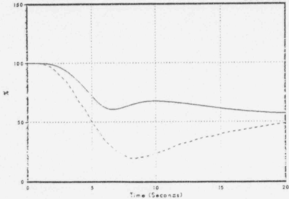
Figure 3.2-69 Feedwater Flow
