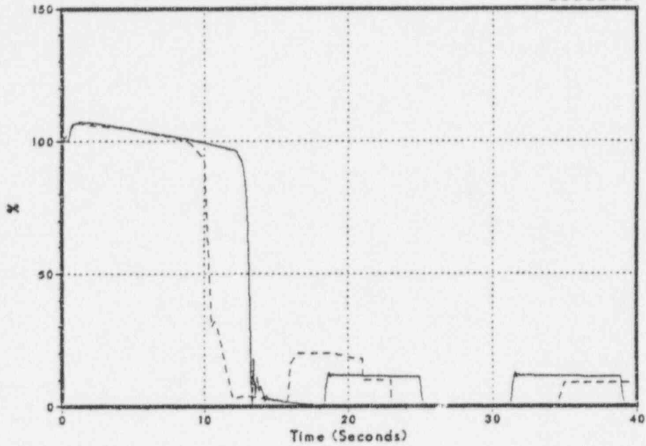
Figure 3.2-54 Main Steam Line Flow
