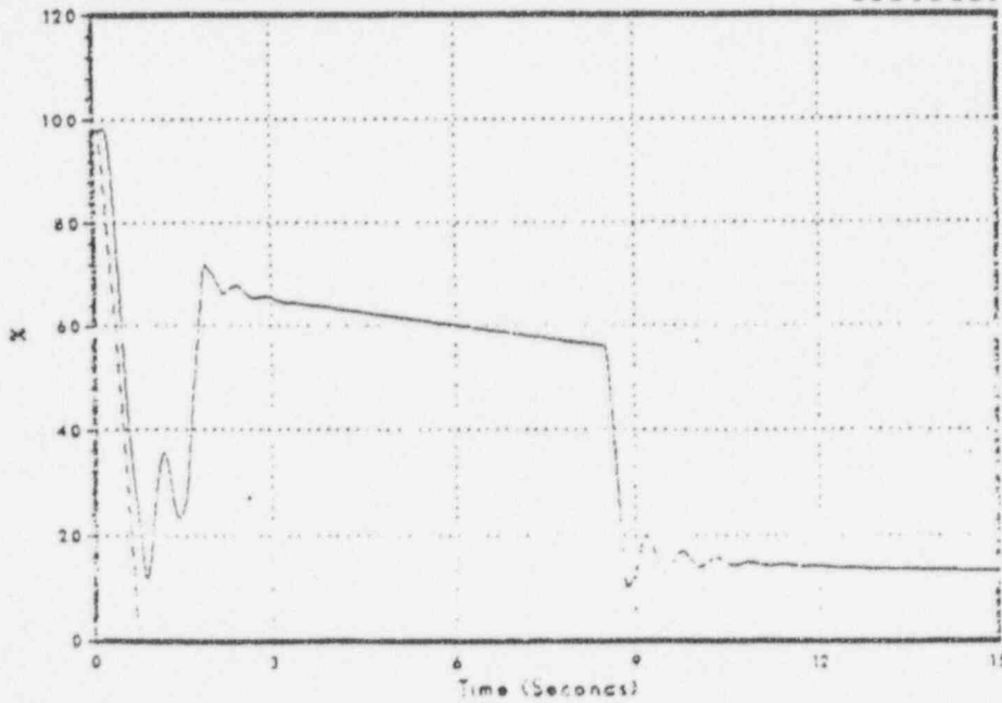
Figure 3.2-125 Main Steam Line Flow
