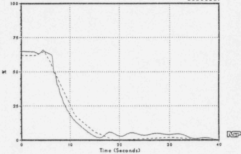
Figure 3.2-77 Vessel Steam Flow
