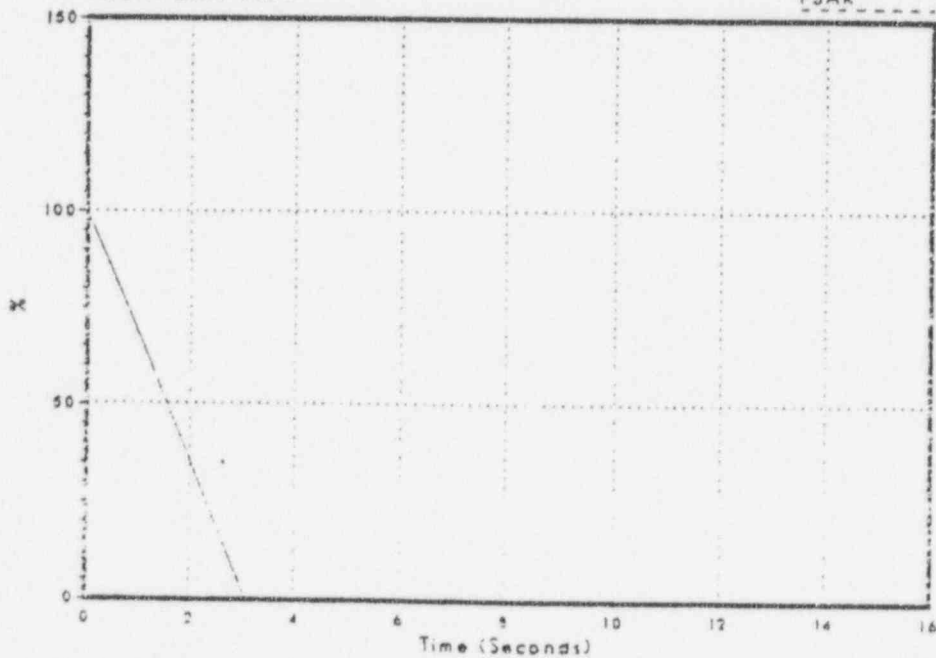
Figure 3.2-41 Feedwater Flow
