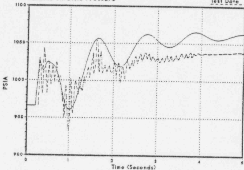
Figure 3.2-118 Turbine Throttle Pressure
