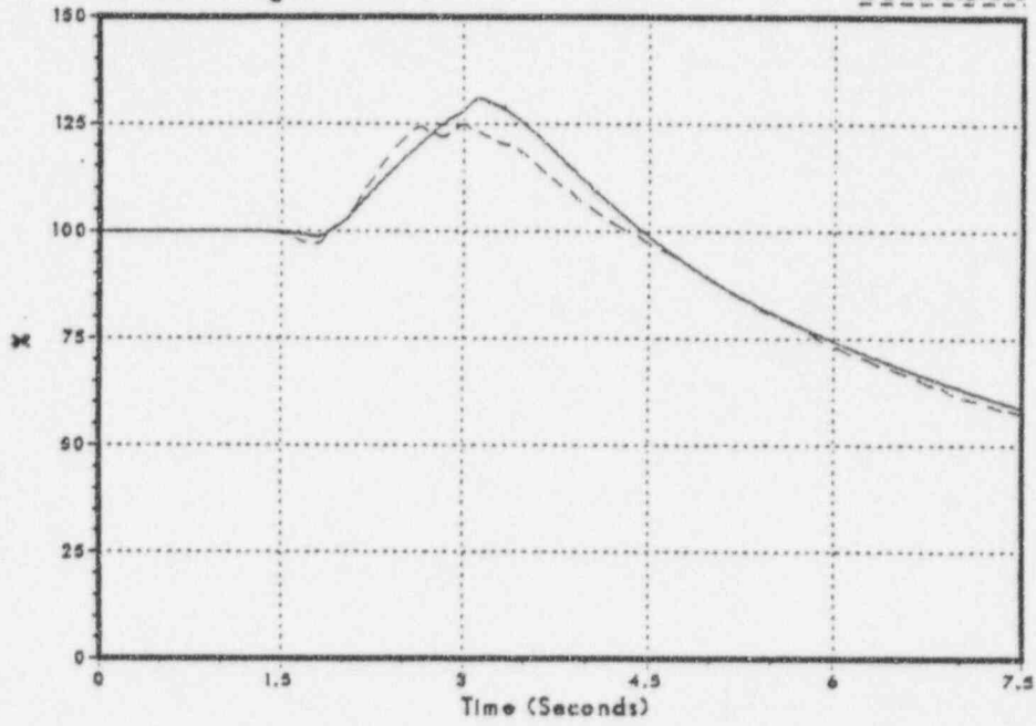
Figure 3.2-108 Core Average Heat Flux
