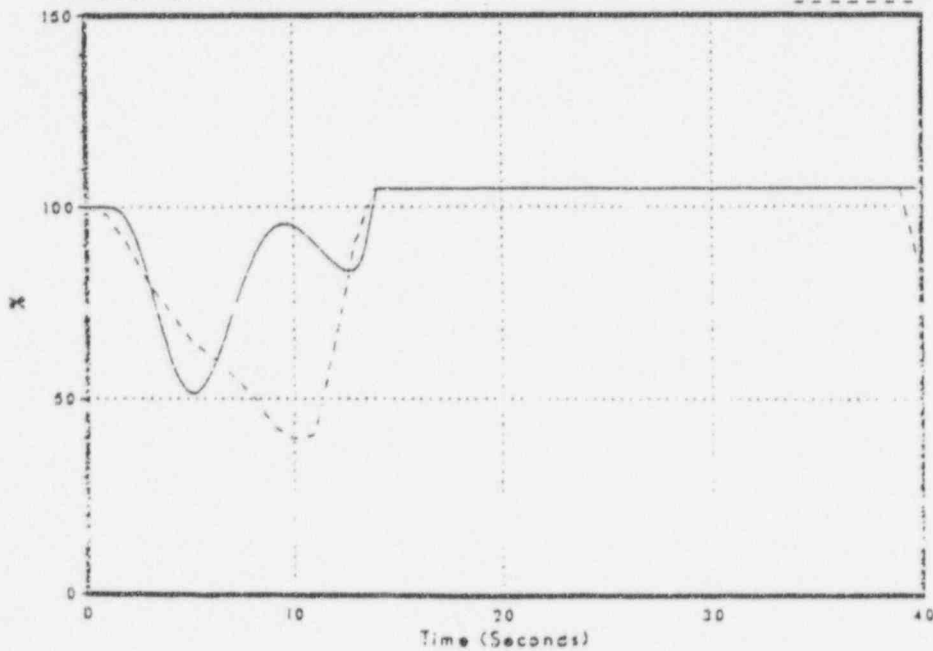
Figure 3.2-55 Feedwater Flow
