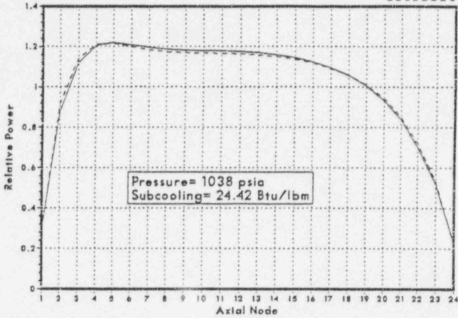
Figure 3.1-1 Relative Power
