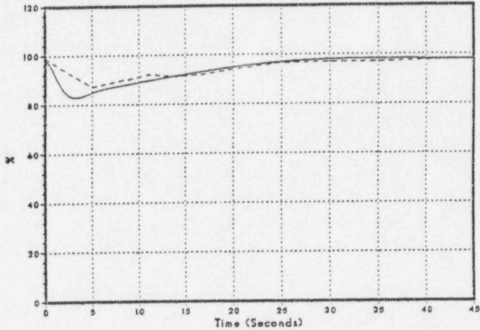
Figure 3.2-148 Feedwater Flow
