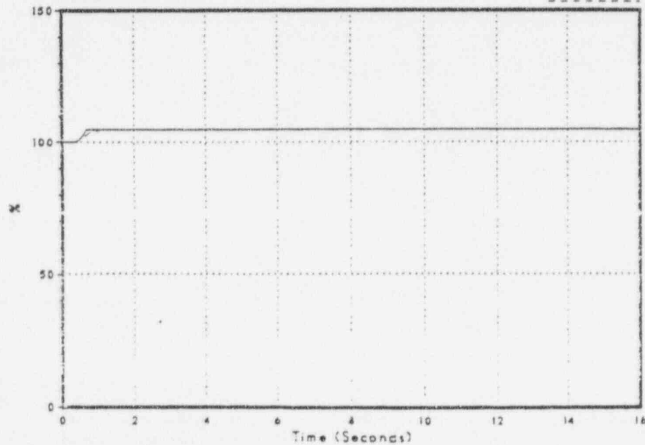
Figure 3.2-6 Feedwater Flow
