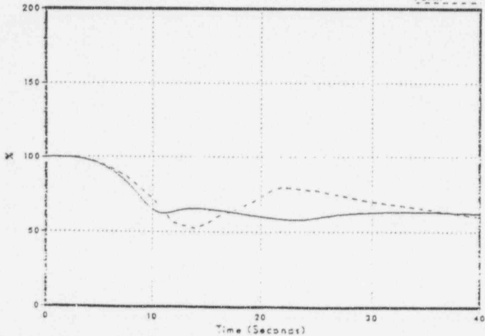
Figure 3.2-83 Feedwater Flow
