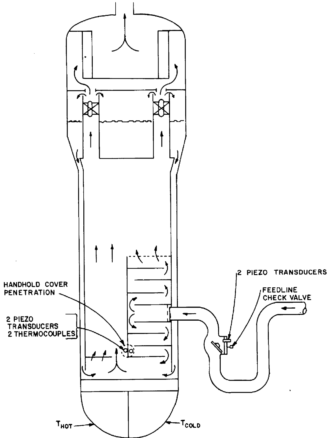
Figure 14-1. Special Test Instrumentation
