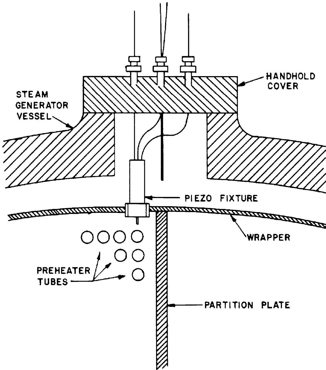
Figure 14-2. Piezo Transducer Fixture Installation in Preheater
