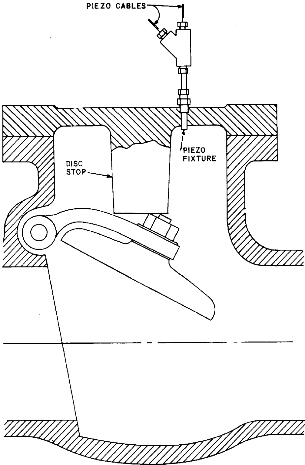
Figure 14-3. Piezoelectric Transducer Probe in Feedline Check Valve
