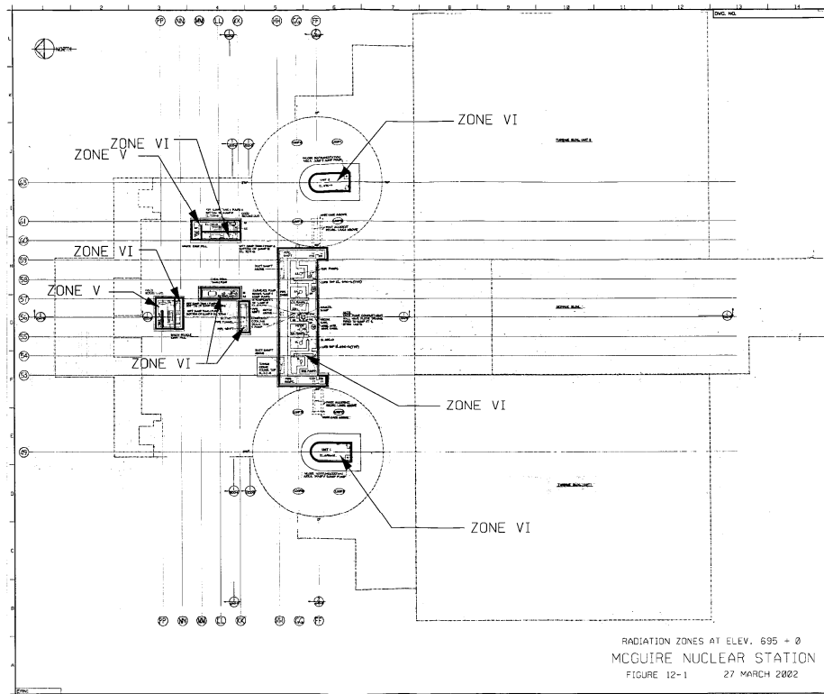
Figure 12-1. Radiation Zones at El. 695 + 0
