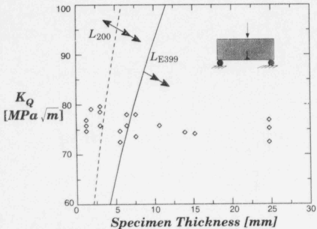
FIG. 9—Variation of fracture toughness with specimen thickness for 4340 steel a_0 = 12.7 mm, W = 25.4 mm.
