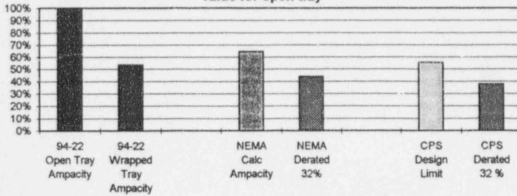
#8 AWG, 1/C ampacity as a percentage of the IEIN 94-22 test result value for open tray
