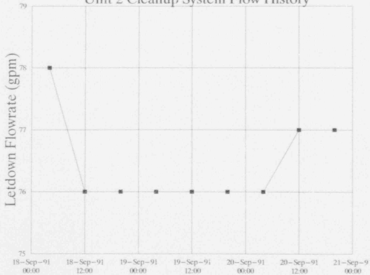
Unit 2 Cleanup System Flow History
