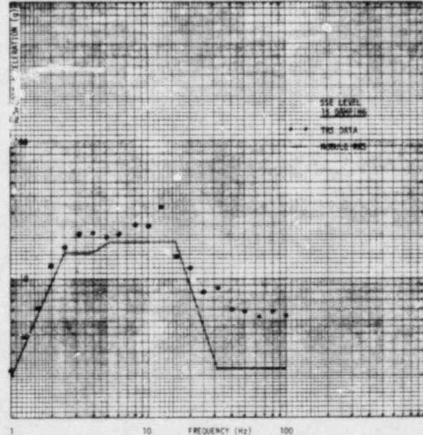
Vertical Response
