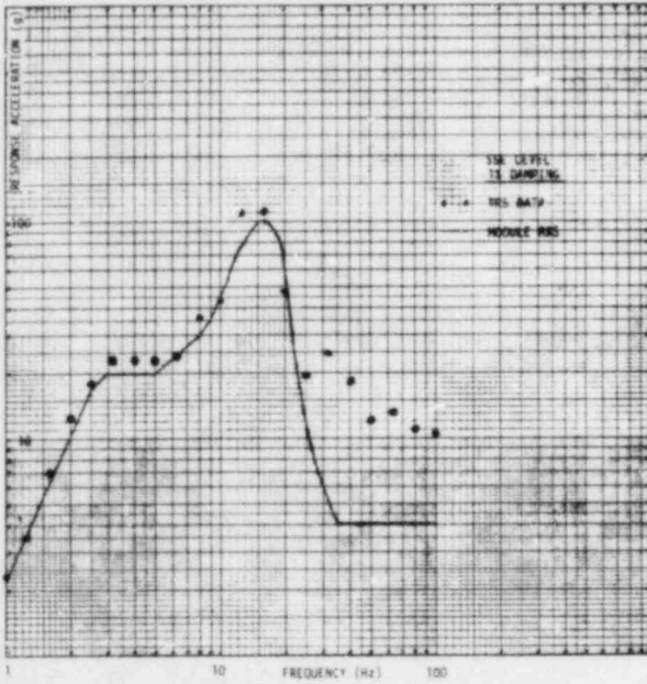
Back-to-Front Response
