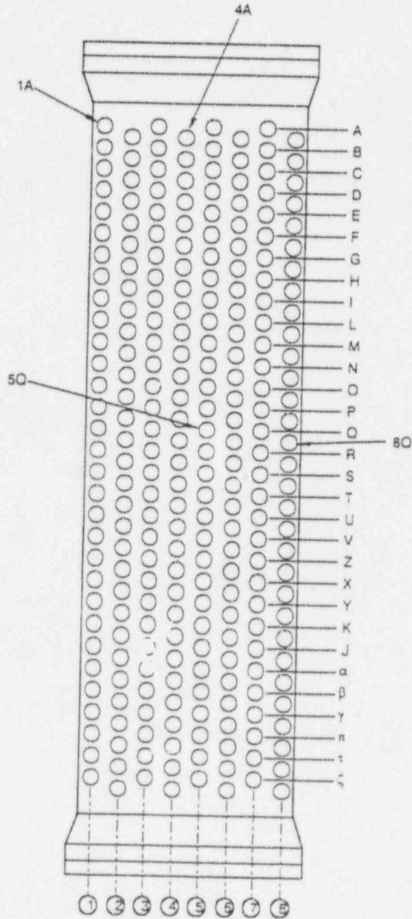
FIGURE 4-3. LOCATION OF PCC WALL TEMPERATURE MEASUREMENT
