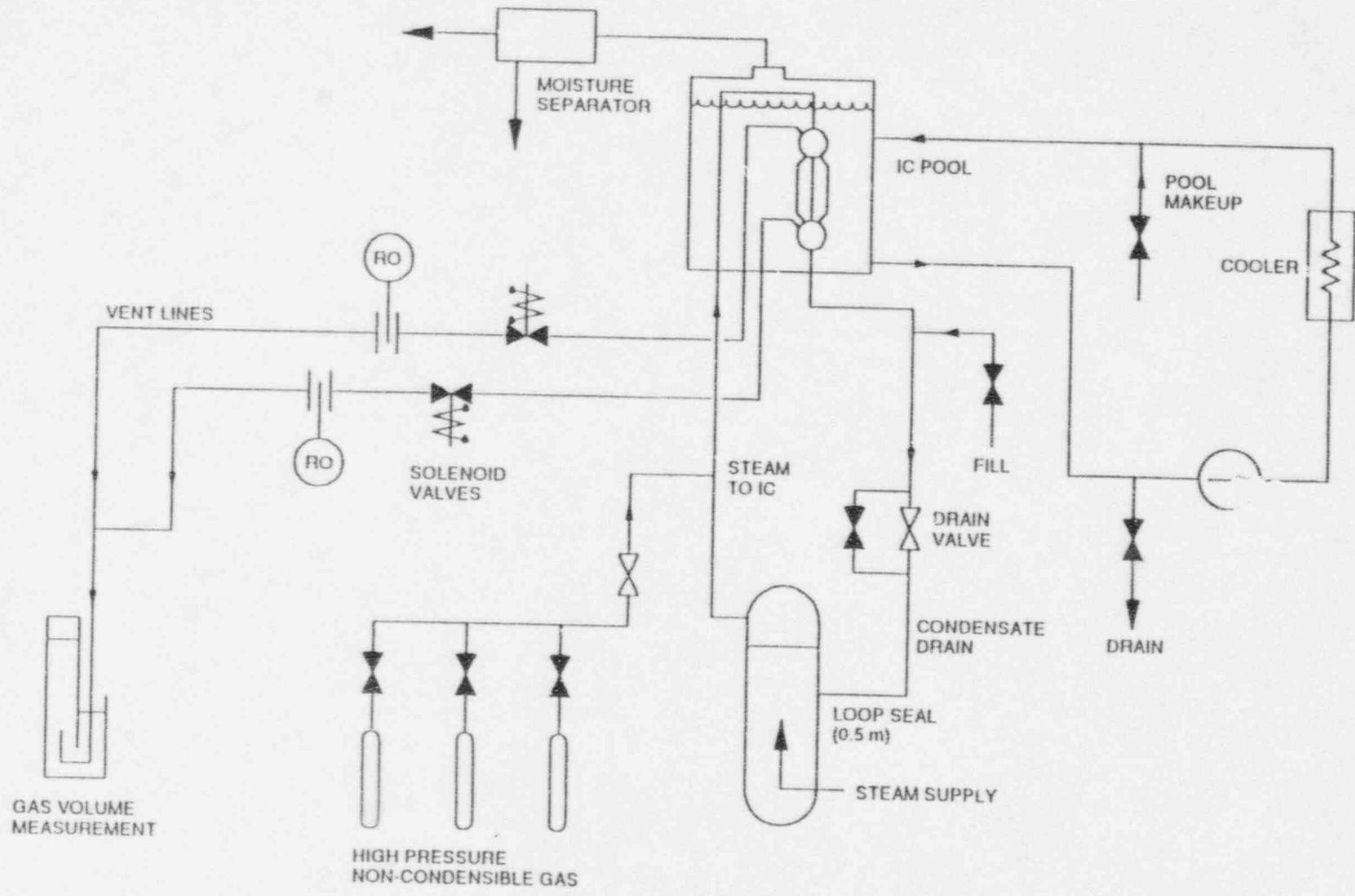
FIGURE 4-5. SCHEMATIC OF IC TEST FACILITY
