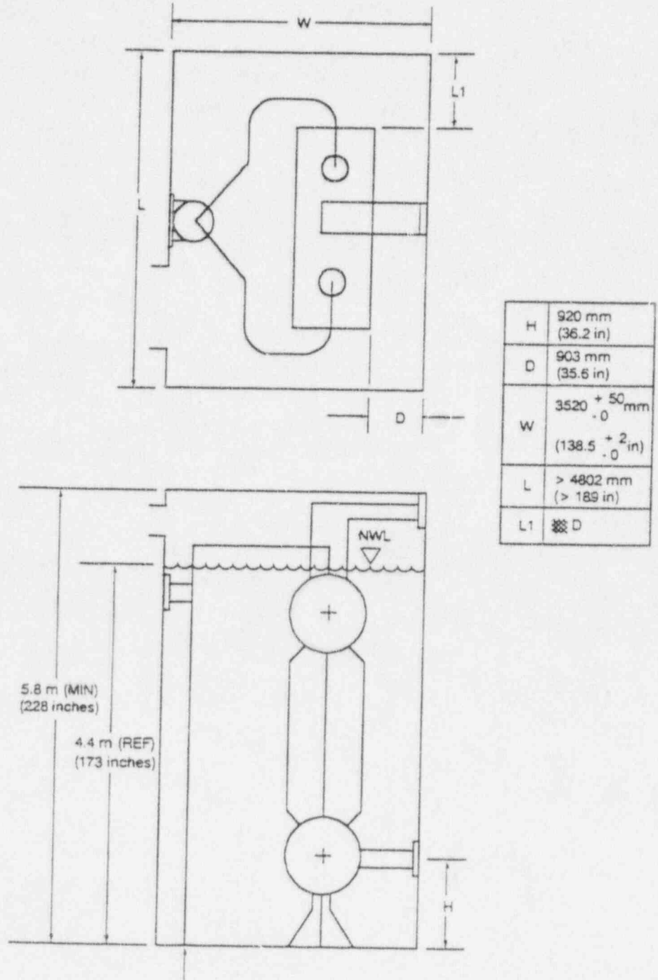
FIGURE 4-6. REQUIRED DIMENSIONS FOR IC TEST POOL
