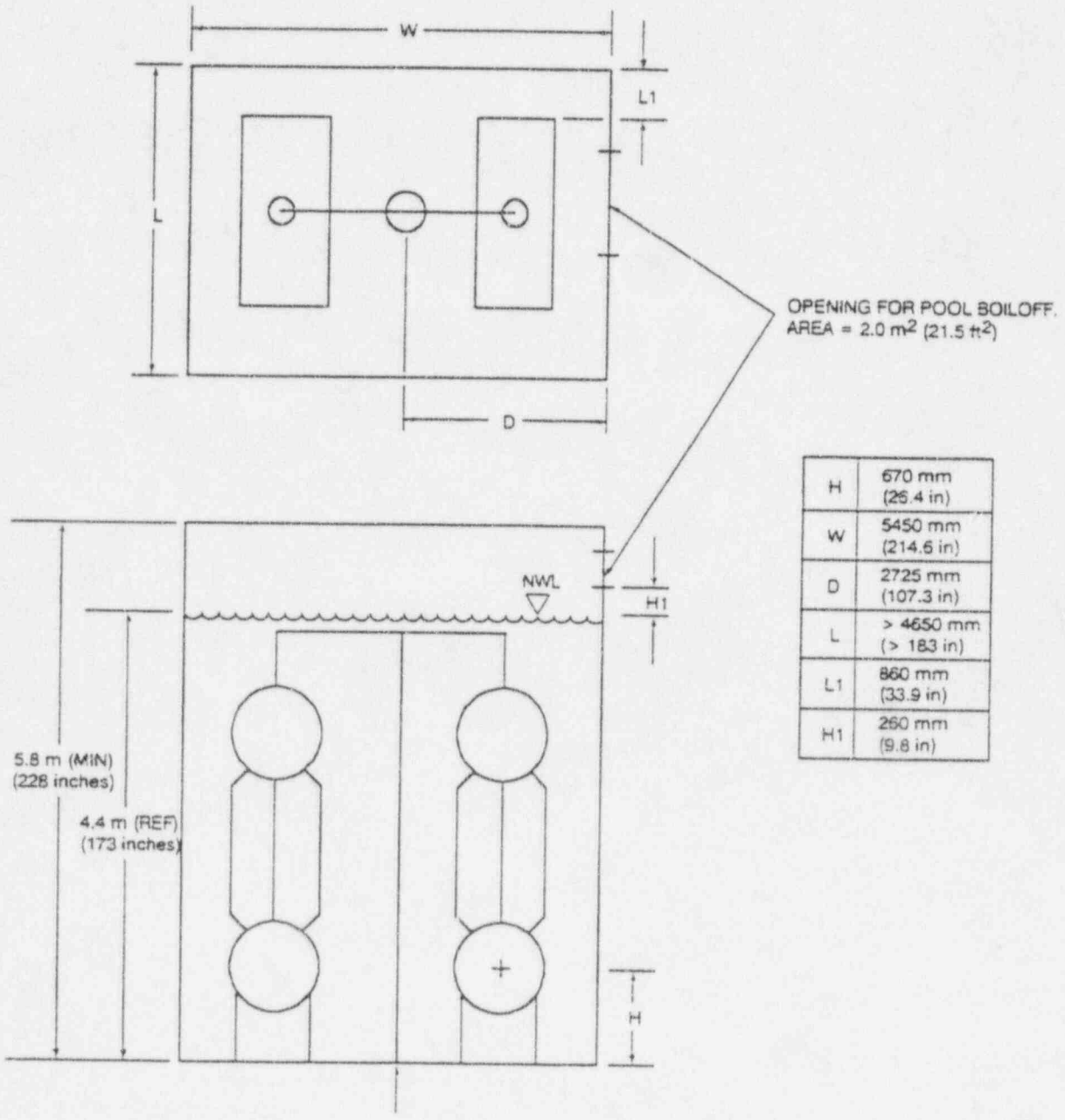
FIGURE 4-2. REQUIRED DIMENSIONS FOR PCC TEST POOL
