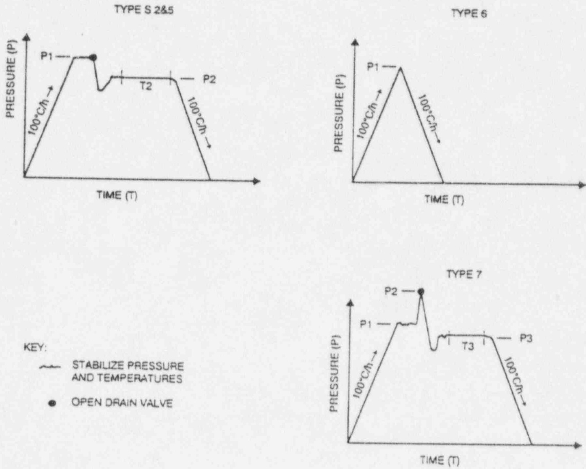
FIGURE 6-1. BASIC IC STRUCTURAL TEST CYCLES
