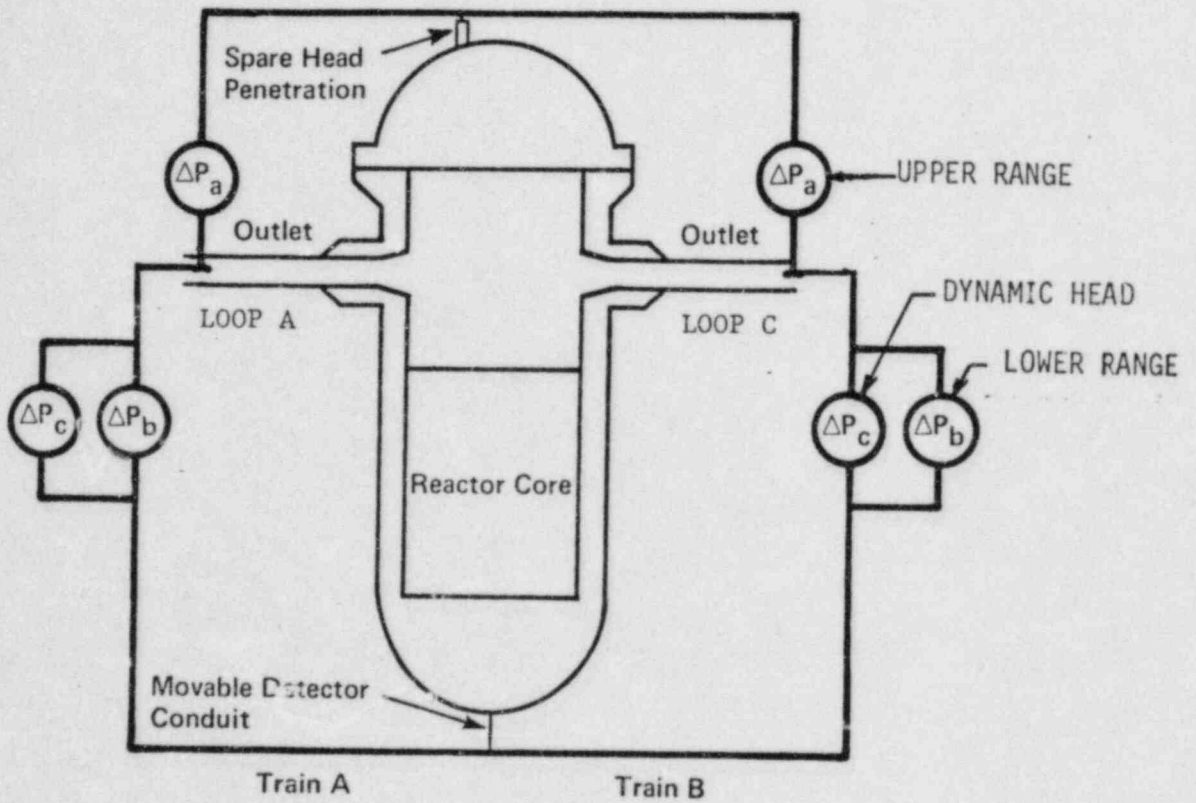
Figure 4.9-1. RVLIS System
