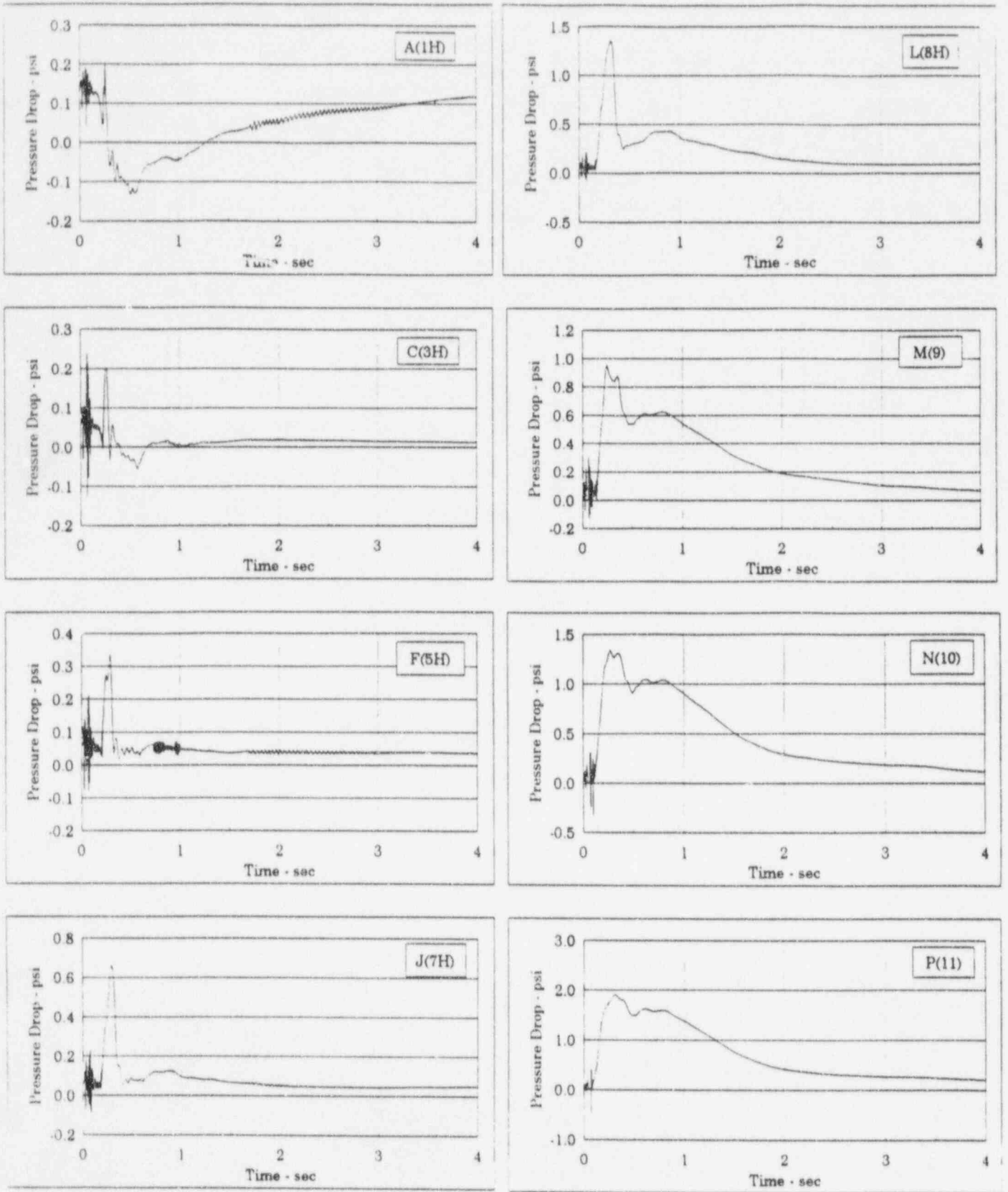
Figure 5. RELAP Pressure Drops
