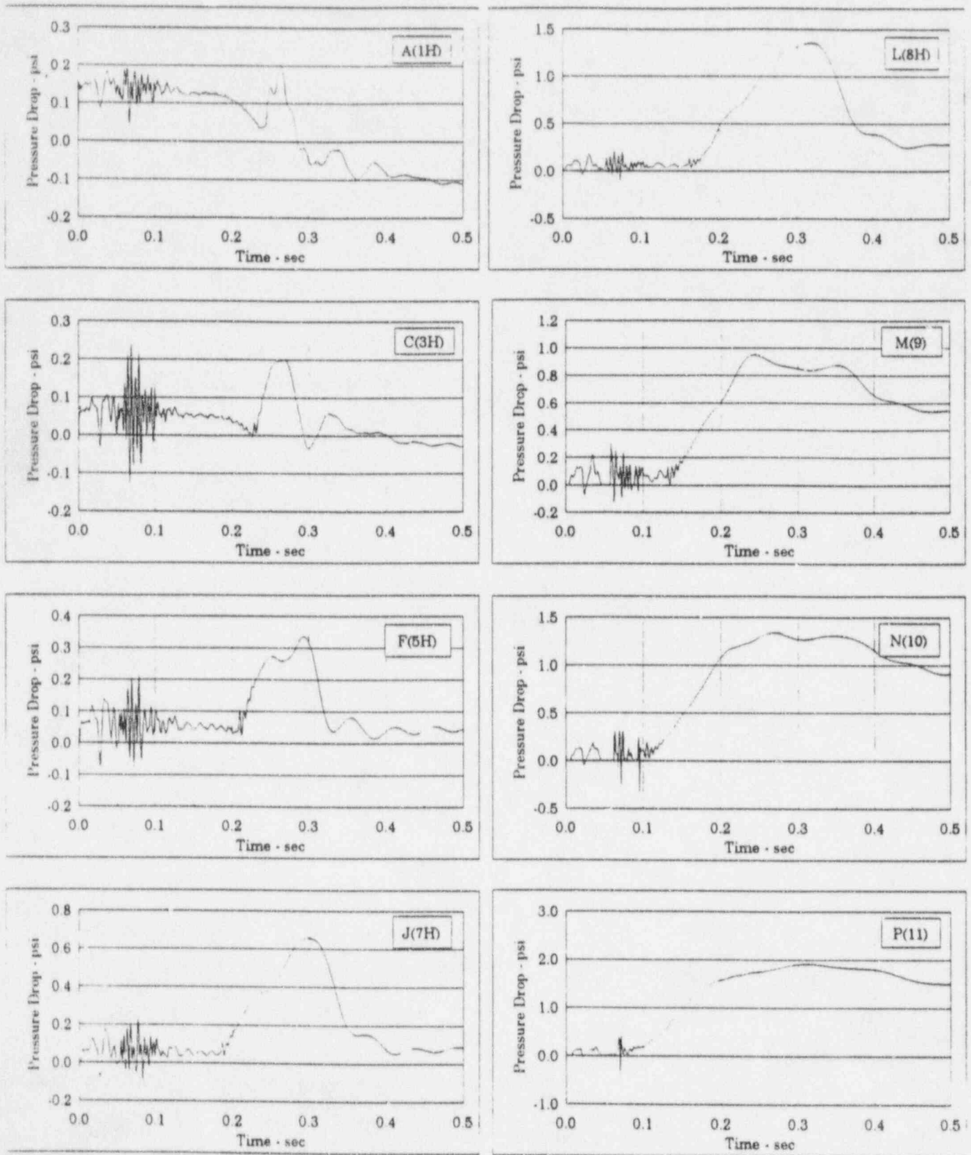
Figure 6. RELAP Pressure Drops: Time = 0. - 0.5 Second
