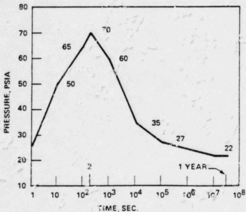
Figure 2 High Energy Line Break
