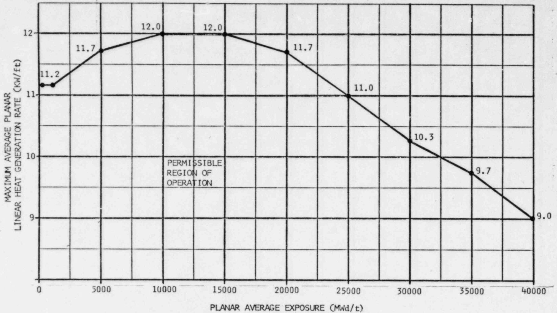
FUEL TYPE P8DRB284H (P8X8R) MAXIMUM AVERAGE PLANAR LINEAR HEAT GENERATION RATE (MAPLHGR) VERSUS AVERAGE PLANAR EXPOSURE
