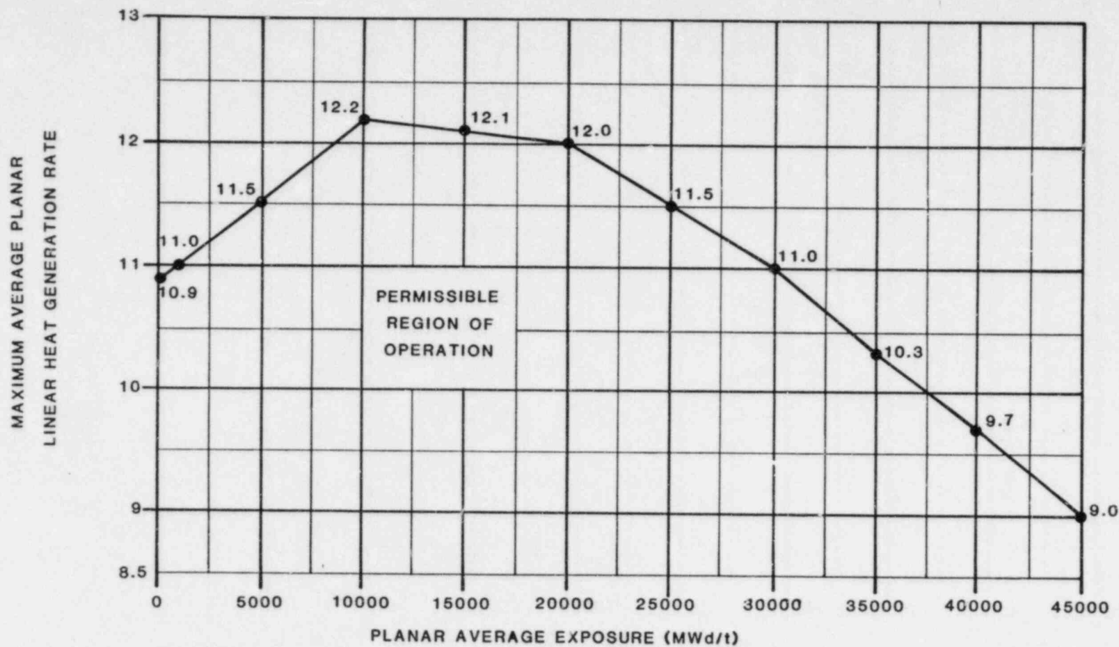
FUEL TYPE BP8DRB299 (BP8x8R) MAXIMUM AVERAGE PLANAR LINEAR HEAT GENERATION RATE (MAPLHGR) VERSUS AVERAGE PLANAR EXPOSURE
