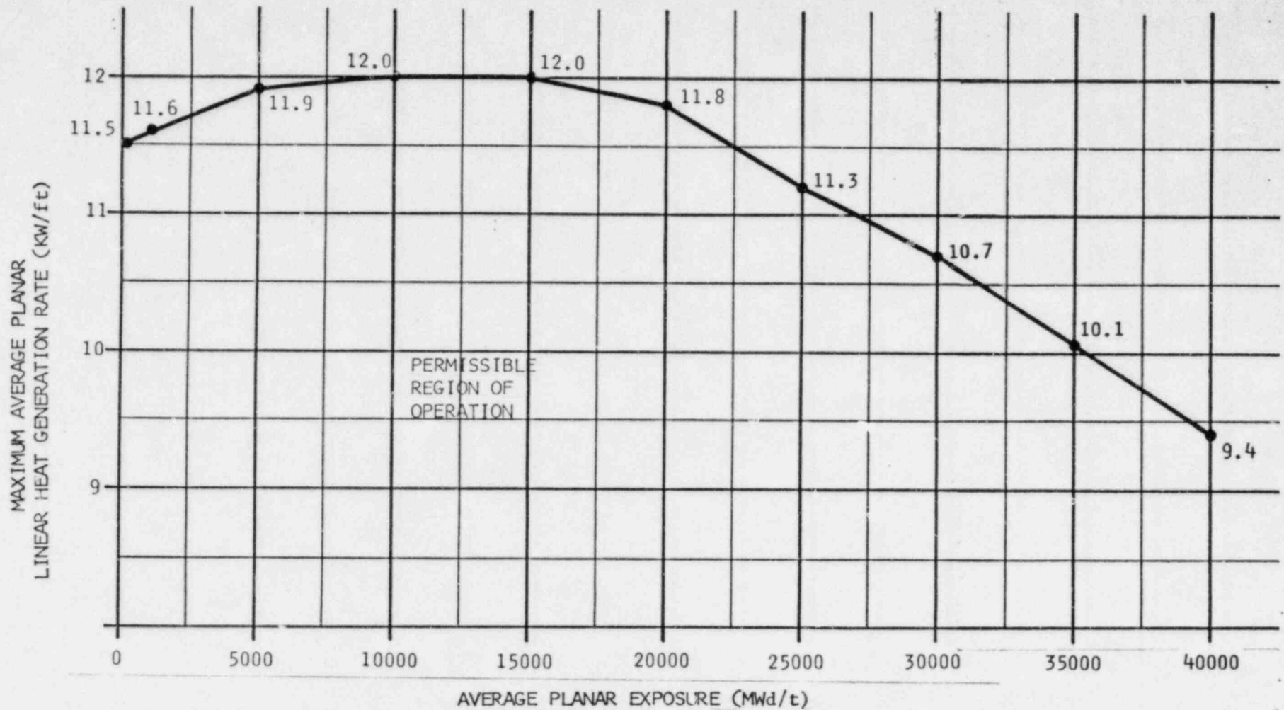
FUEL TYPE 8DRB265H (8X8R) MAXIMUM AVERAGE PLANAR LINEAR HEAT GENERATION RATE (MAPLHGR) VERSUS AVERAGE PLANAR EXPOSURE
