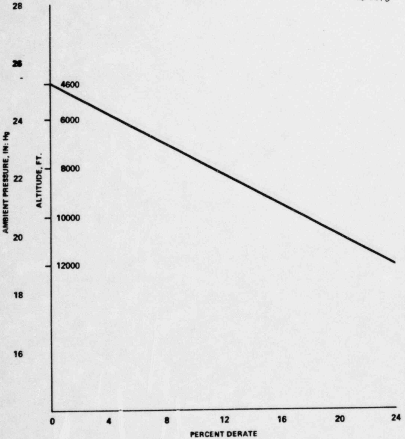
HOPE CREEK GENERATING STATION FINAL SAFETY ANALYSIS REPORT 12 CYL. PC2 (4238KW AT 514 RPM) AMBIENT PRESSURE VS. PERCENT DERATE FIGURE 430.145-1 AMENDMENT 6, 06/84
