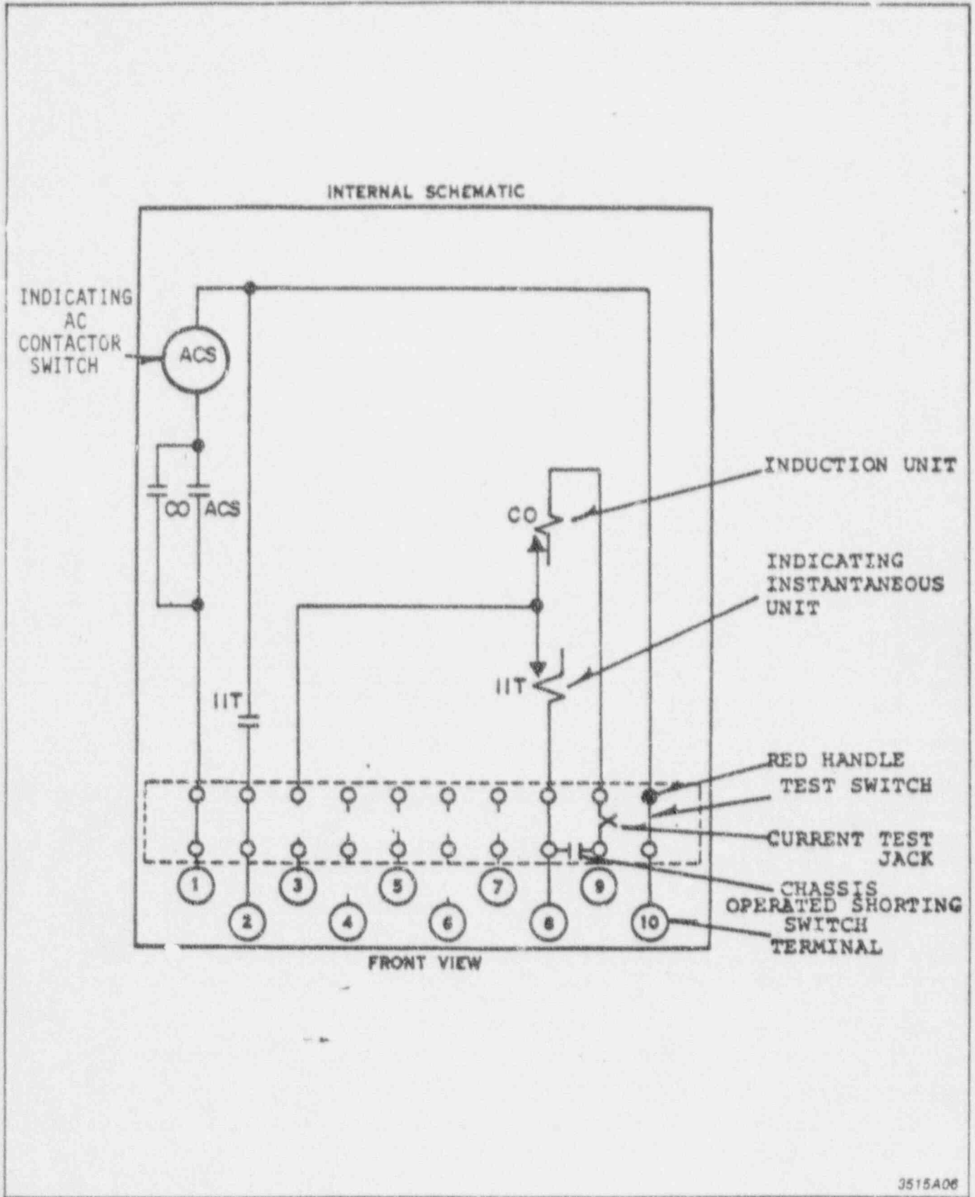
Fig. 8. Internal Schematic of the Single Trip Relay with an ACS unit and IIT
