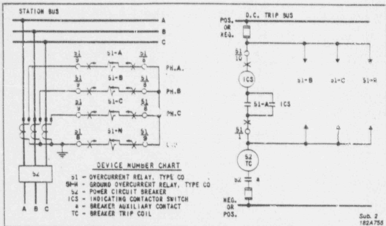
Fig. 17. External Schematic of HiLo CO relay for Phase and Ground Overcurrent Protection on a Three Phase System.
