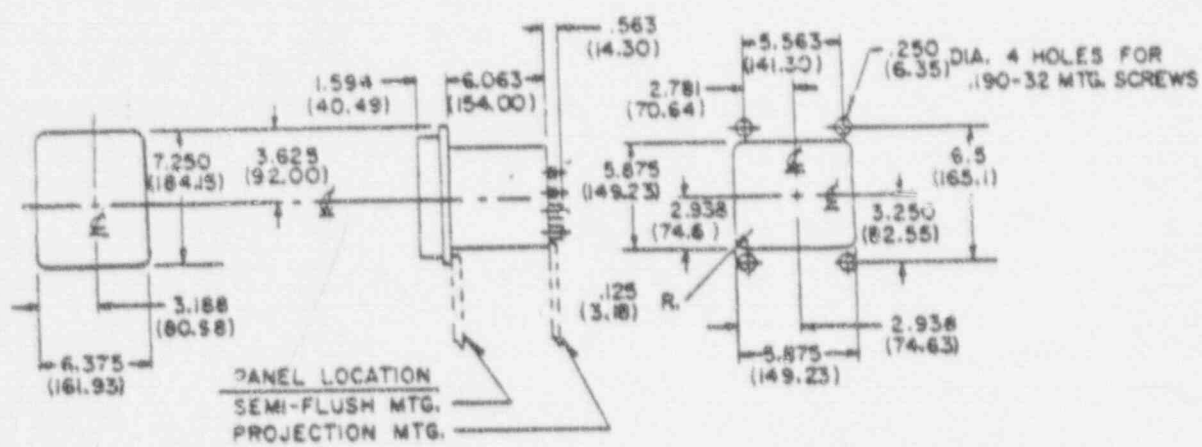
PANEL CUTOUT & DRILLING FOR SEMI-FLUSH MTG.
