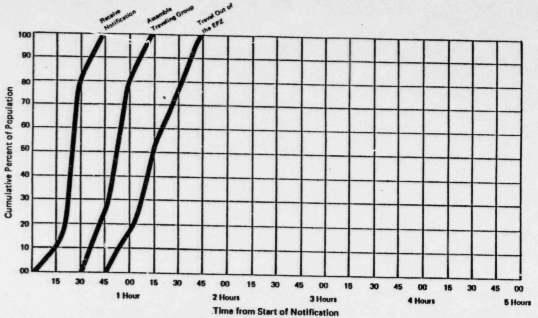
Figure 18. Evacuation Times for the Transient Population
