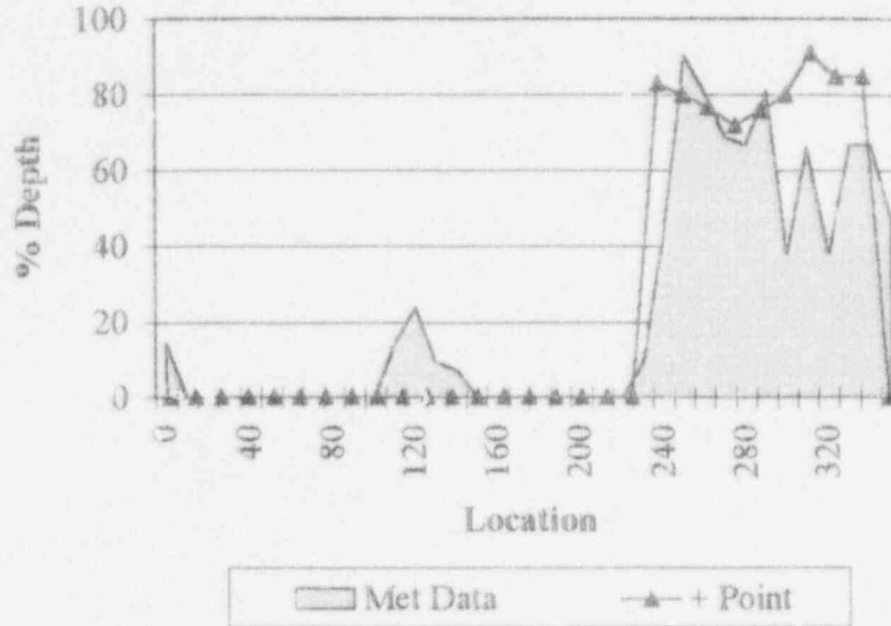
Figure B-2 Lab Crack #2 - Comparison of Met and + Point Data
