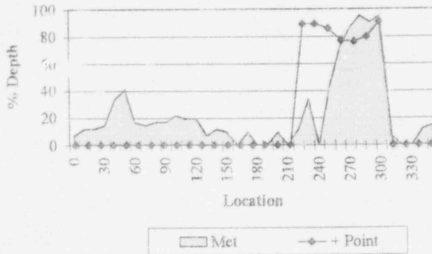
Figure B-5 Lab Crack #5 - Comparison of Met and + Point Data
