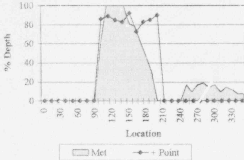
Figure B-4 Lab Crack #4 - Comparison of Met and + Point Data
