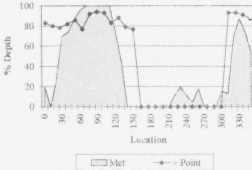
Figure B-3 Lab Crack #3 - Comparison of Met and + Point Data
