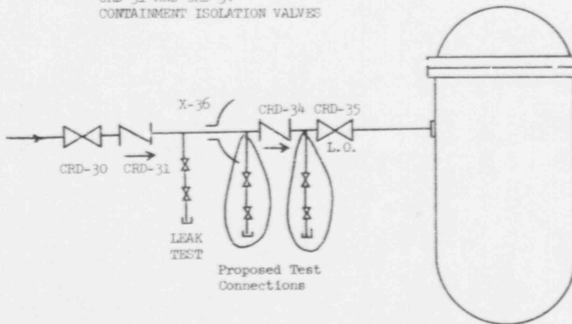
Figure 4. CRD Hydraulic Return Containment Penetration
