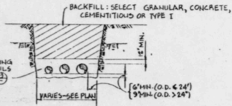
TYPICAL PIPE BEDDING SECTION IN ROCK
