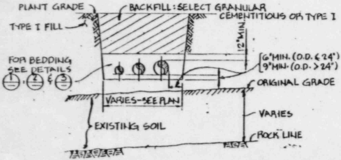
TYPICAL PIPE BEDDING SECTION IN SOIL
