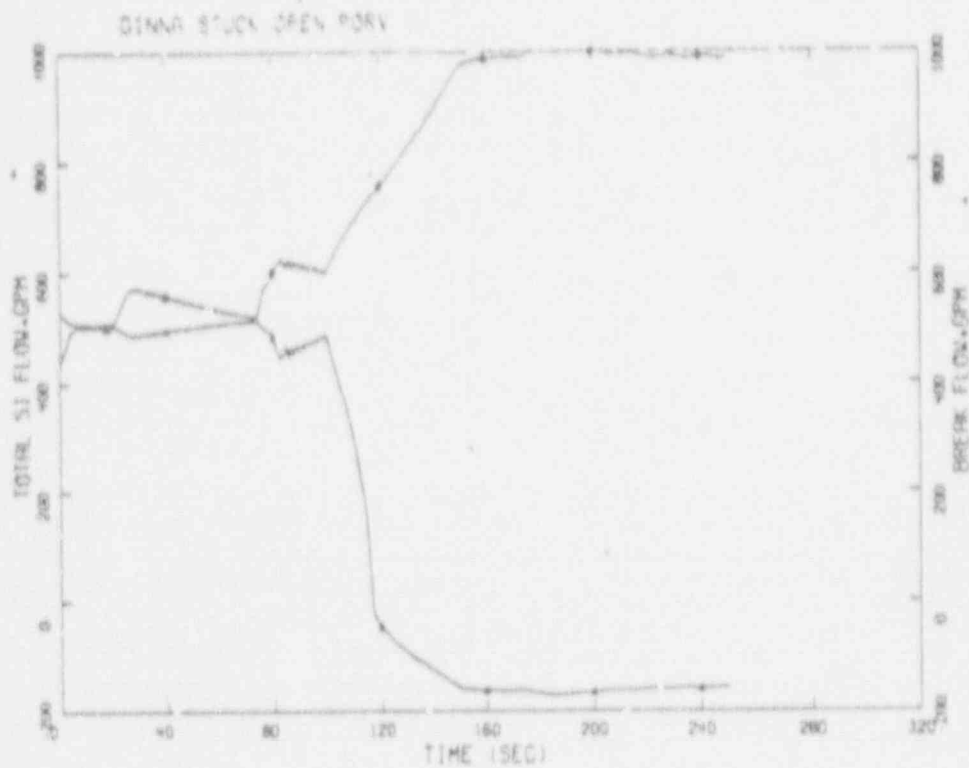
Figure 4.2-10. SI Flow/Break Flow.
