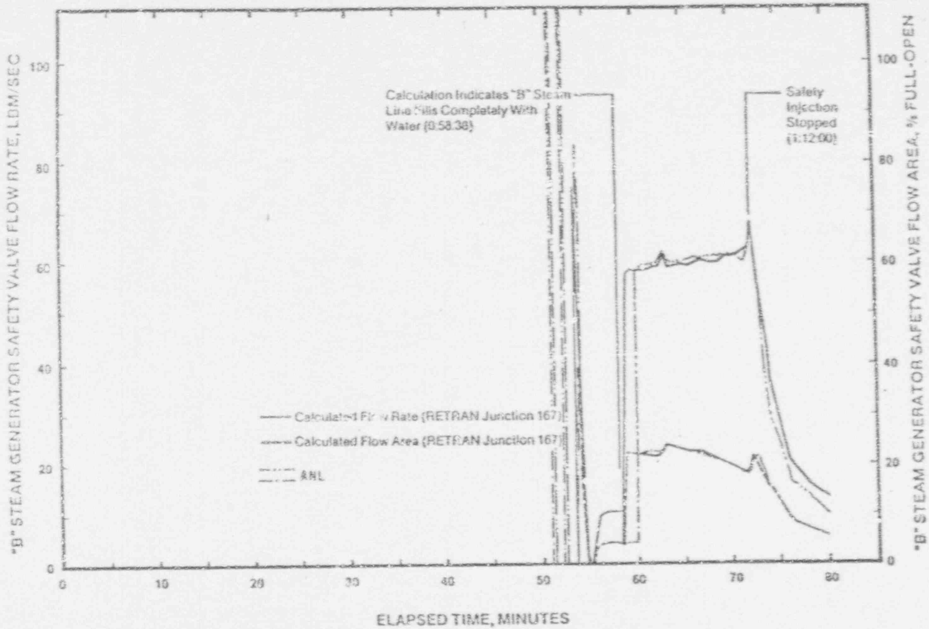
"B" Steam Generator Safety Valve Flow Rate And Flow Area vs. Time
