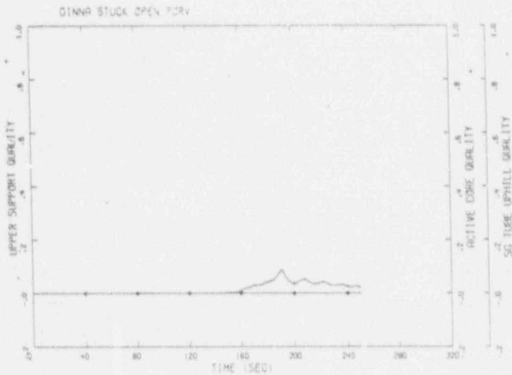
Figure 4.2-3. Upper Support Vol. 20/Active Core Vol. 1/SG Tube, Vol. 43 Quality.
