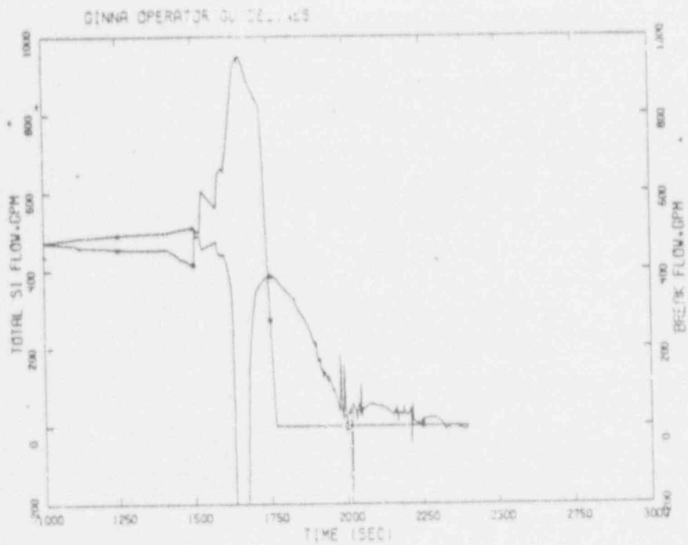
Figure 4.1-4. SI Flow/Break Flow.
