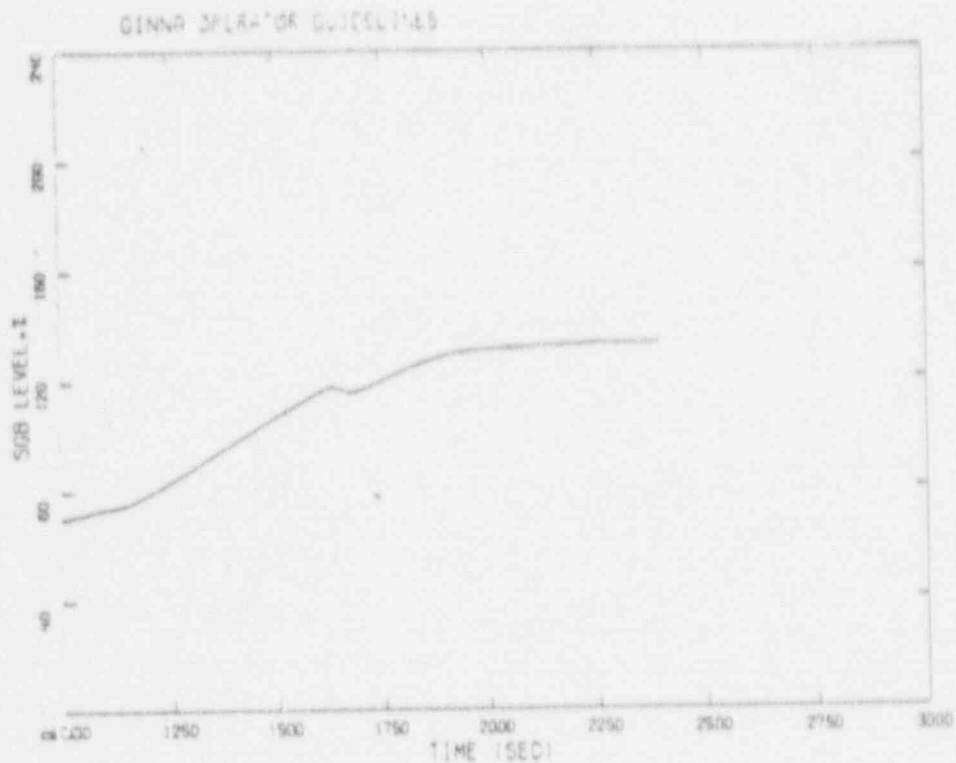
Figure 4.1-5. SGB Level.
