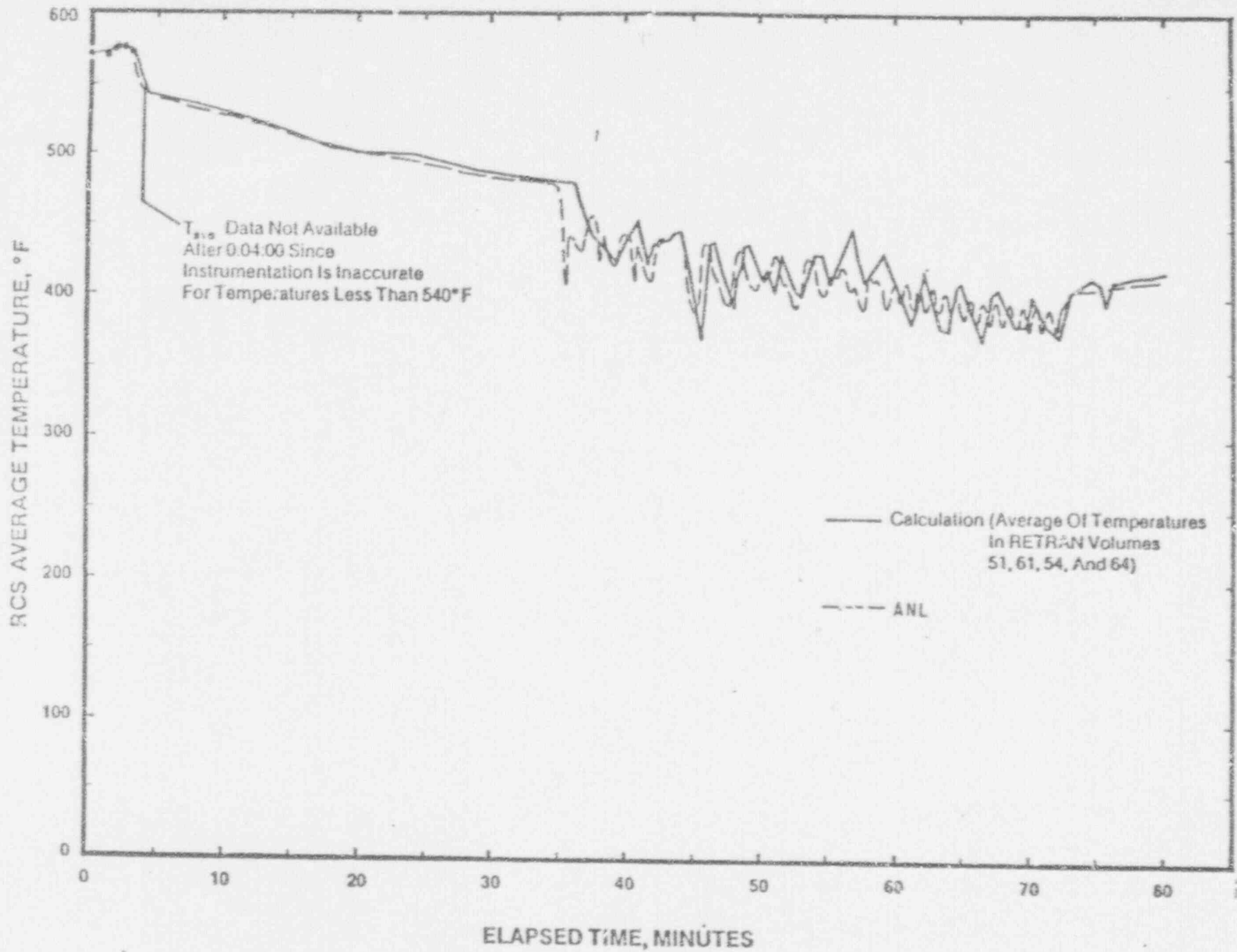
RCS Average Temperature vs. Time
