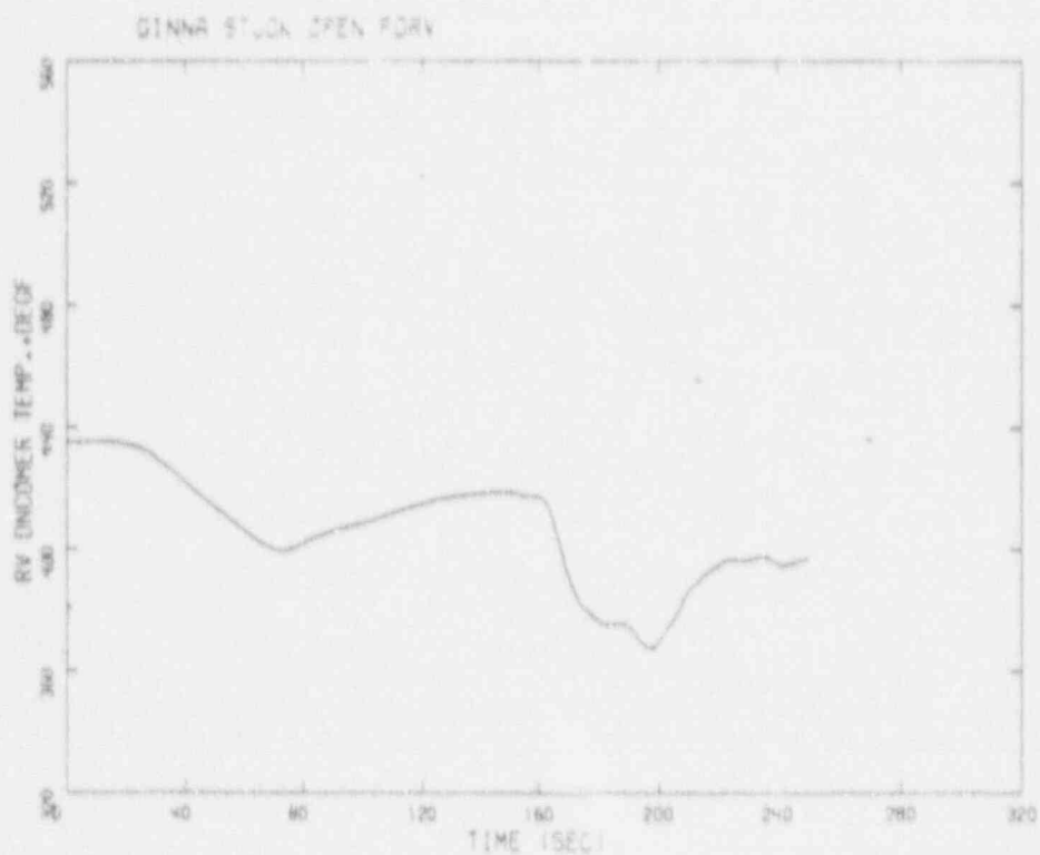
Figure 4.2-11. Vessel Downcomer Temp. vs Time.
