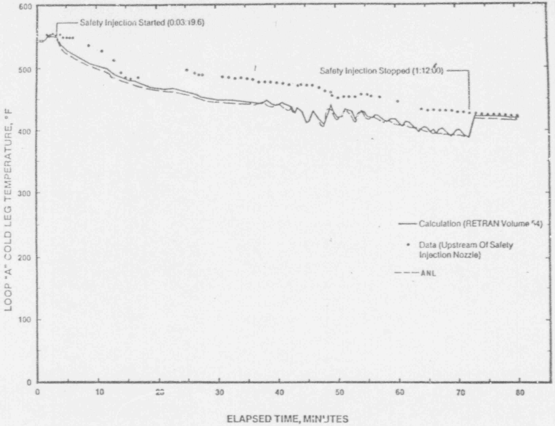
Loop "A" Cold Leg Temperature vs. Time
