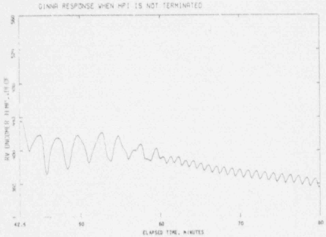
FIGURE 4.3-5. REACTOR VESSEL DOWNCOMER (VOL. 1R) TEMPERATURE.
