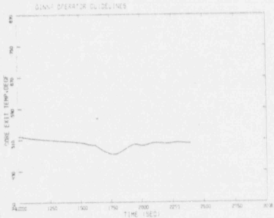
Figure 4.1-6. Core Exit Vol. 13 Temperature.
