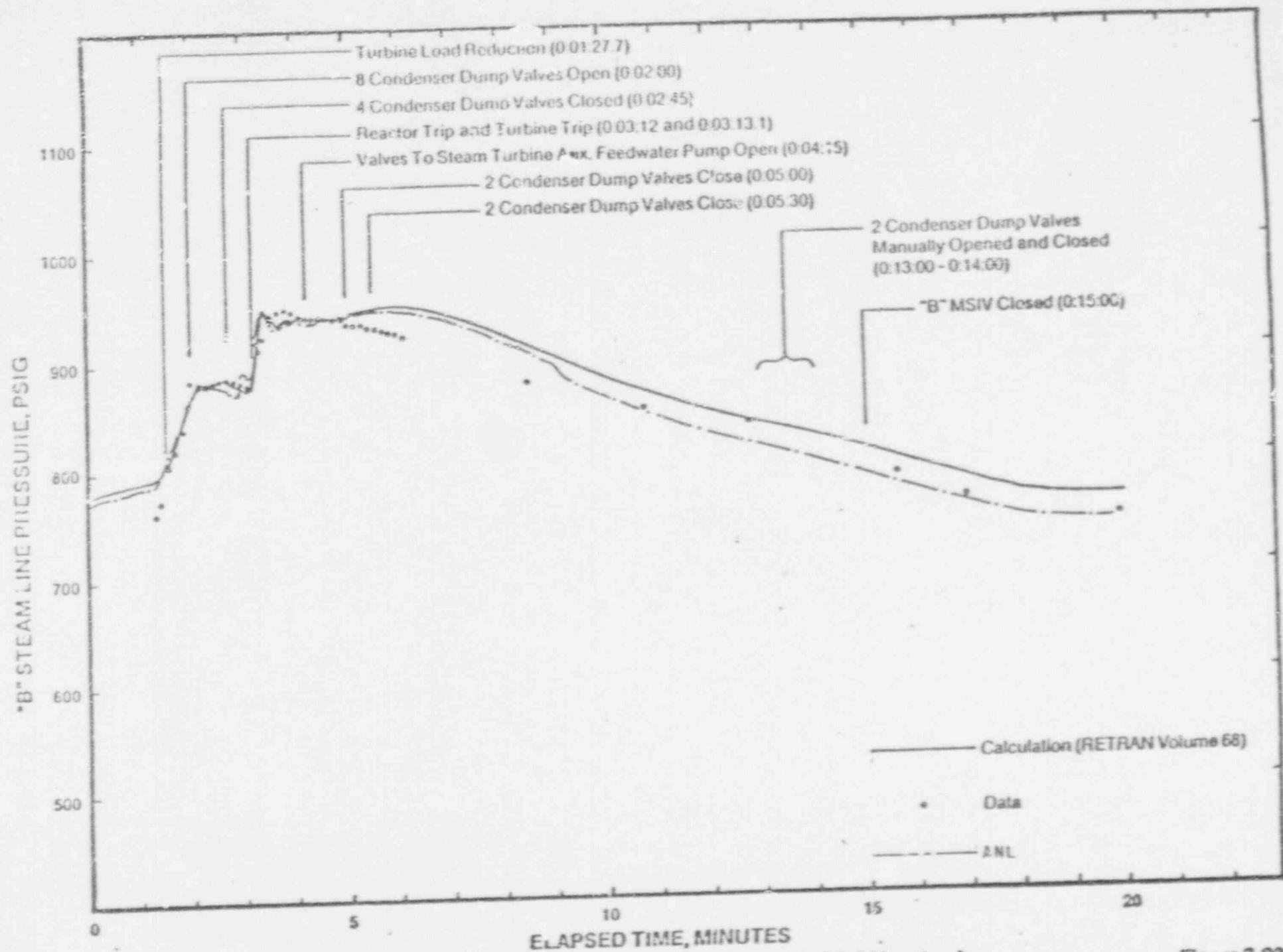
"B" Steam Line Pressure vs. Time (0-20 Minutes)
