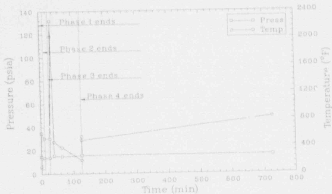
Figure B-10. Peach Bottom AE-gamma drywell data.
