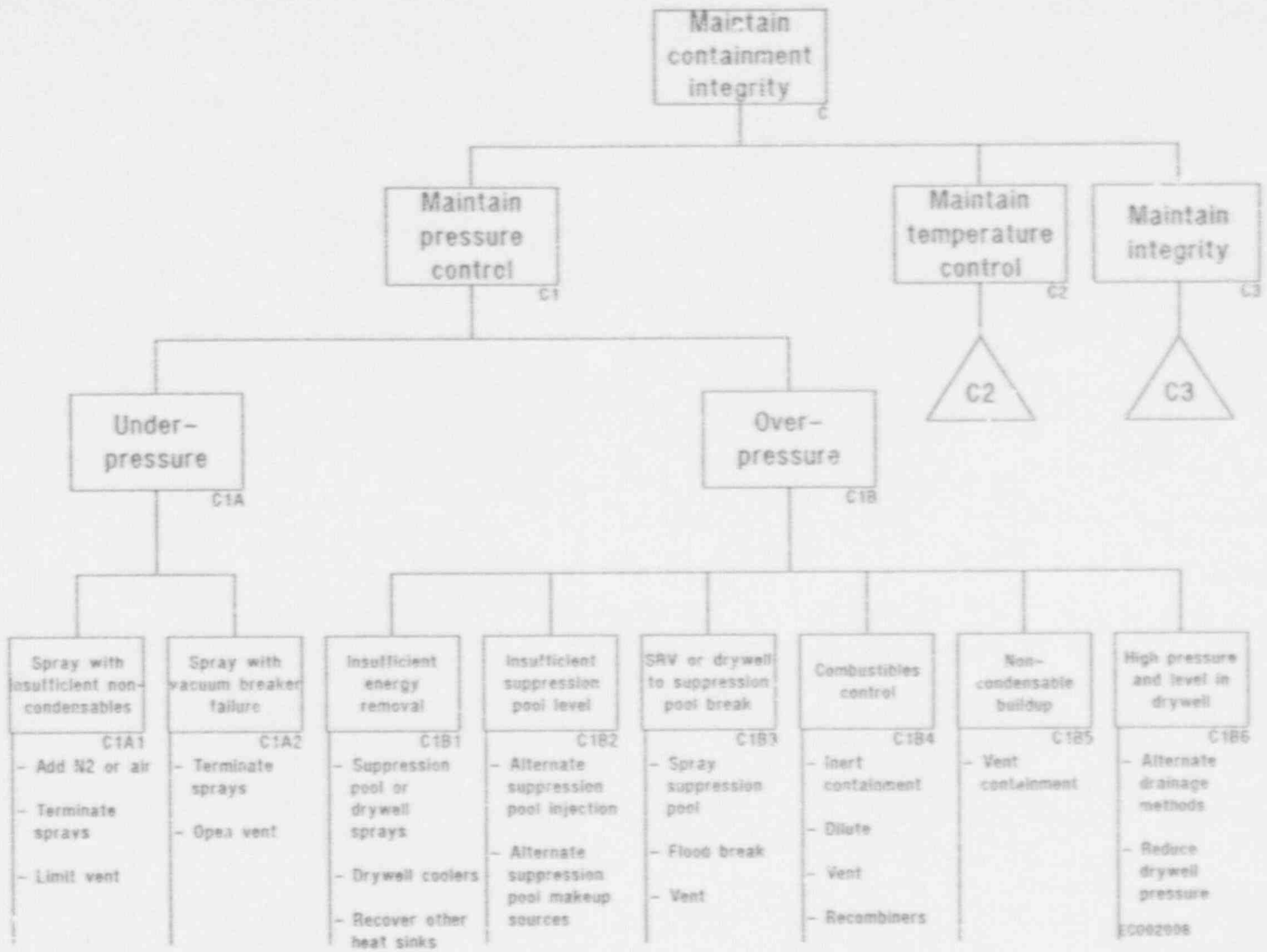
Figure 2. Safety objective tree: prevent containment failure (from NUREG/CR-5702).
