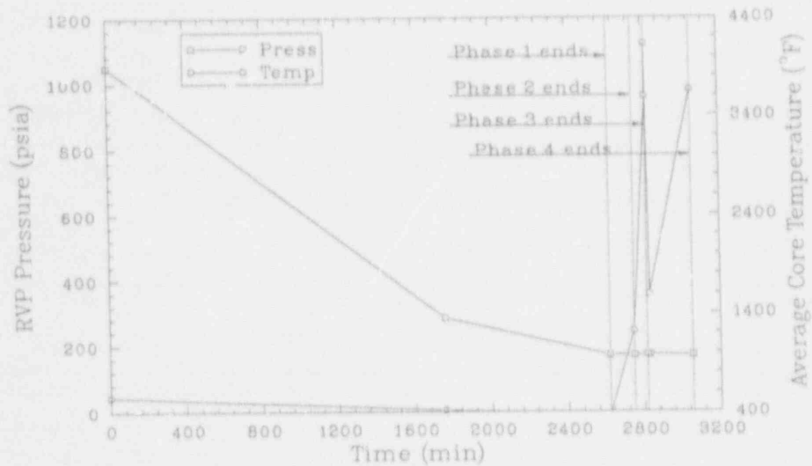
Figure B-26. Peach Bottom TW-γ reactor system data.
