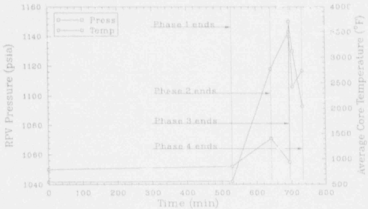
Figure B-1. Peach Bottom TB1 reactor system data.
