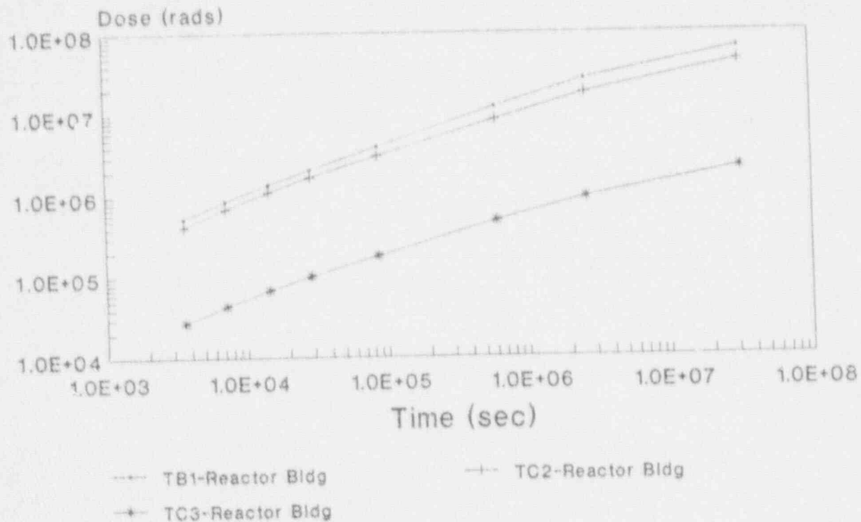
Figure D-3. Dose comparison for reactor building.
