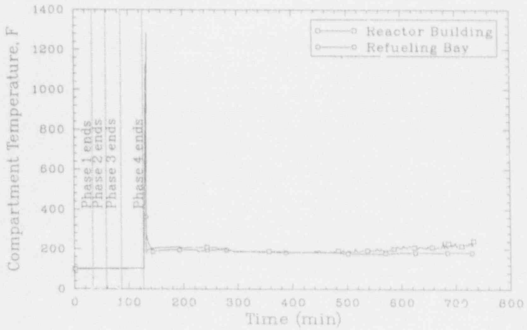
Figure B-20. Peach Bottom TC2 reactor building data.
