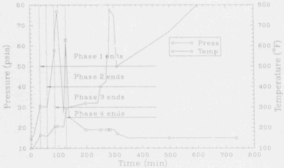
Figure B-22. Peach Bottom TC3 drywell data.
