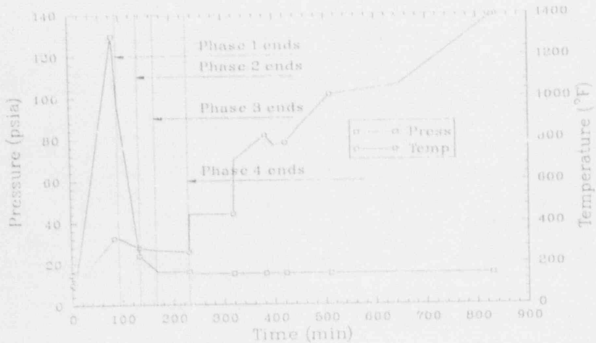
Figure B-14. Peach Bottom TCI drywell data.
