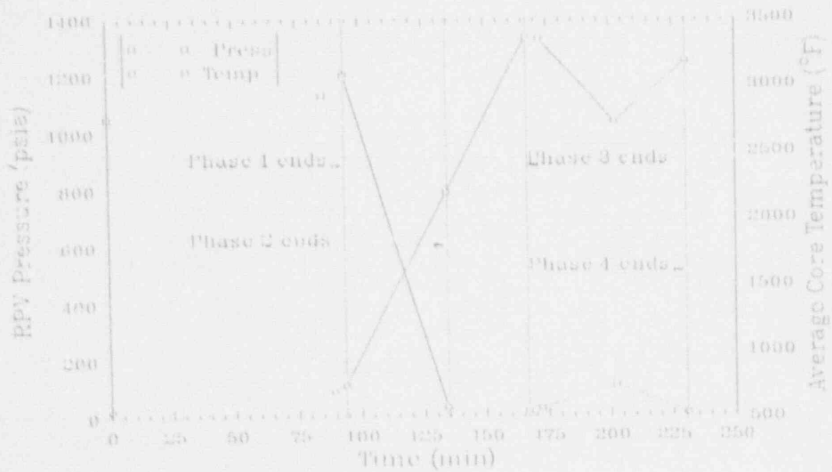
Figure B-13. Peach Bottom TCI reactor system data.
