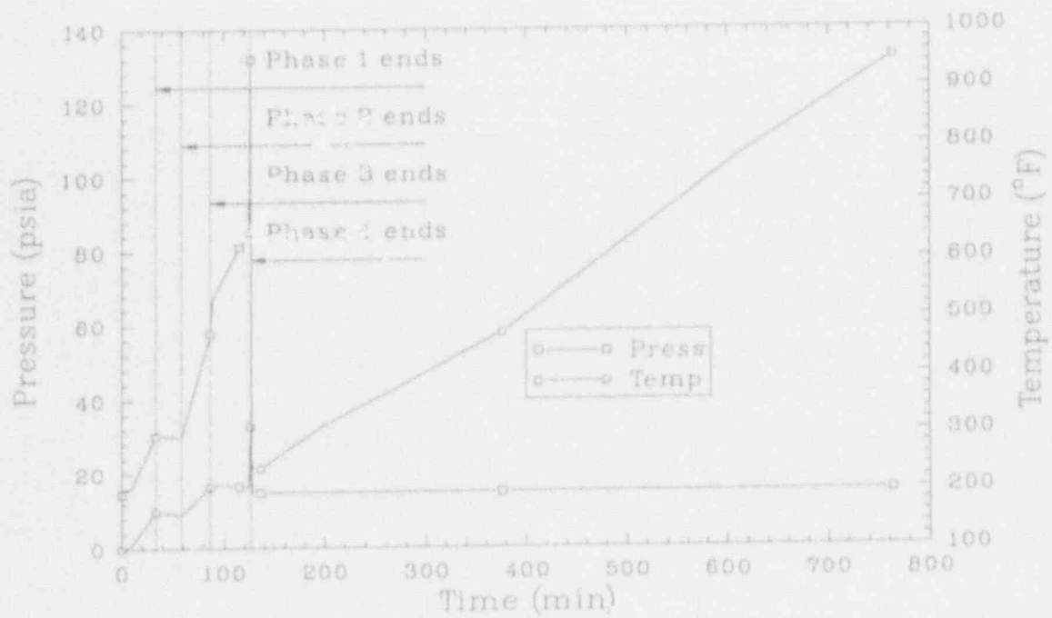
Figure B-18. Peach Bottom TC2 drywell data.
