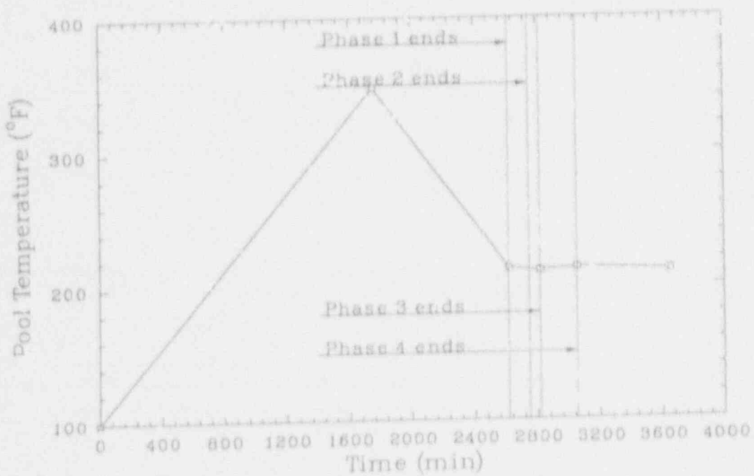
Figure B-28. Peach Bottom TW-g suppression pool temperature.
