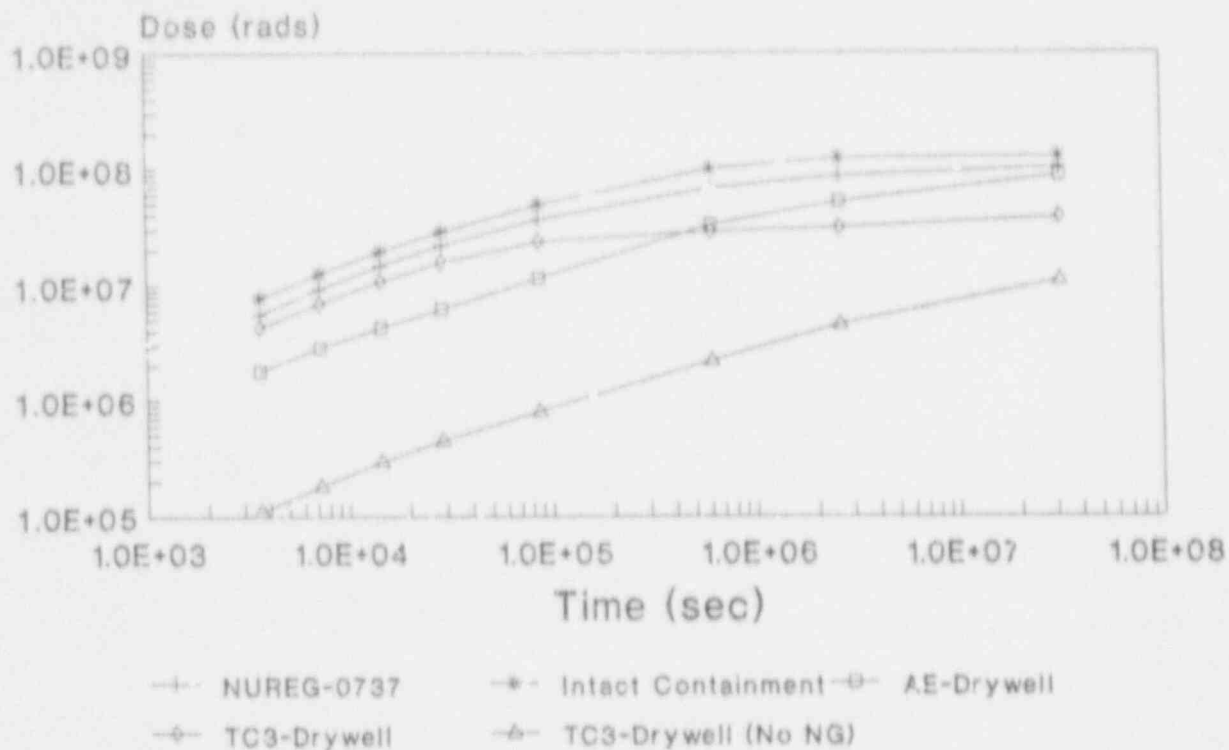
Figure D-1. Dose comparison for drywell.
