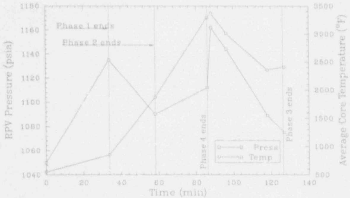
Figure B-21. Peach Bottom TC3 reactor system data.
