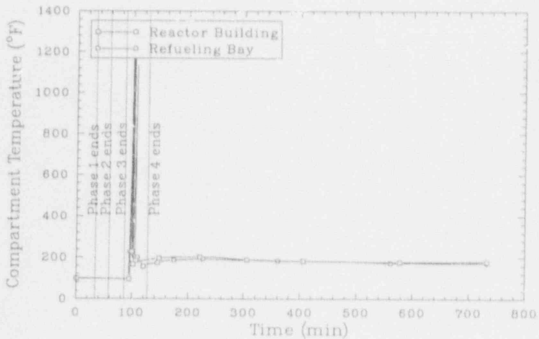
Figure B-24. Peach Bottom TC3 reactor building data.
