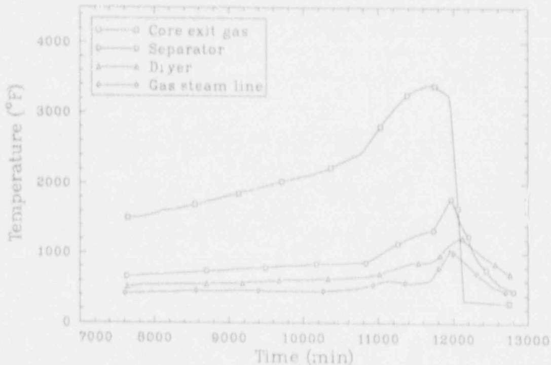
Figure B-29. Peach Bottom TW-gas and structure temperatures.
