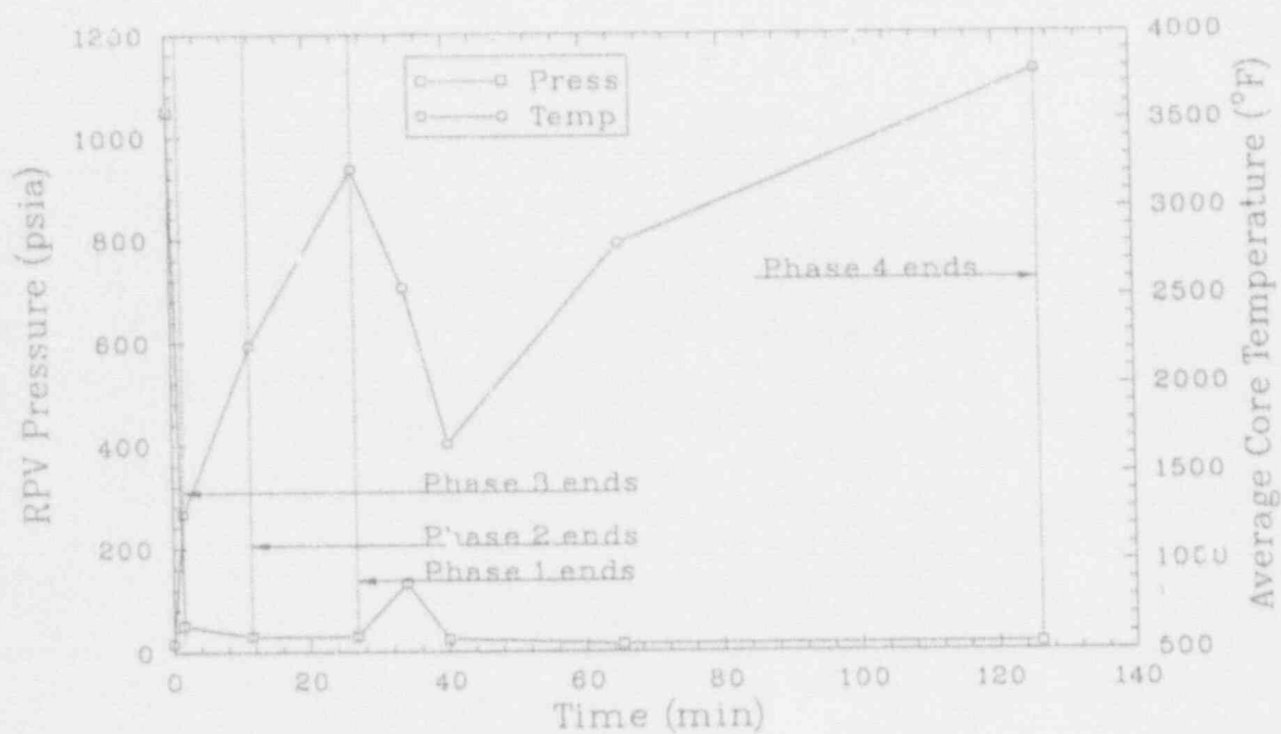
Figure B-9. Peach Bottom AE-gamma reactor system data.
