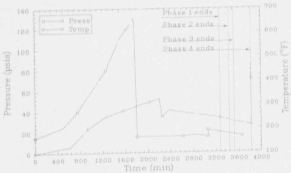
Figure B-27. Peach Bottom TW-g drywell data.
