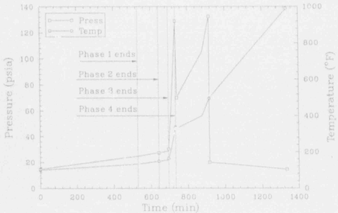
Figure B-2. Peach Bottom TB1 drywell data.
