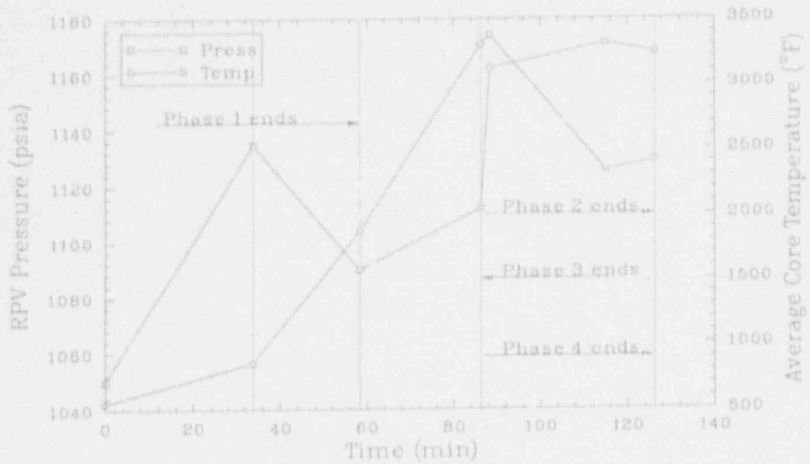
Figure B-17. Peach Bottom TC2 reactor system data.
